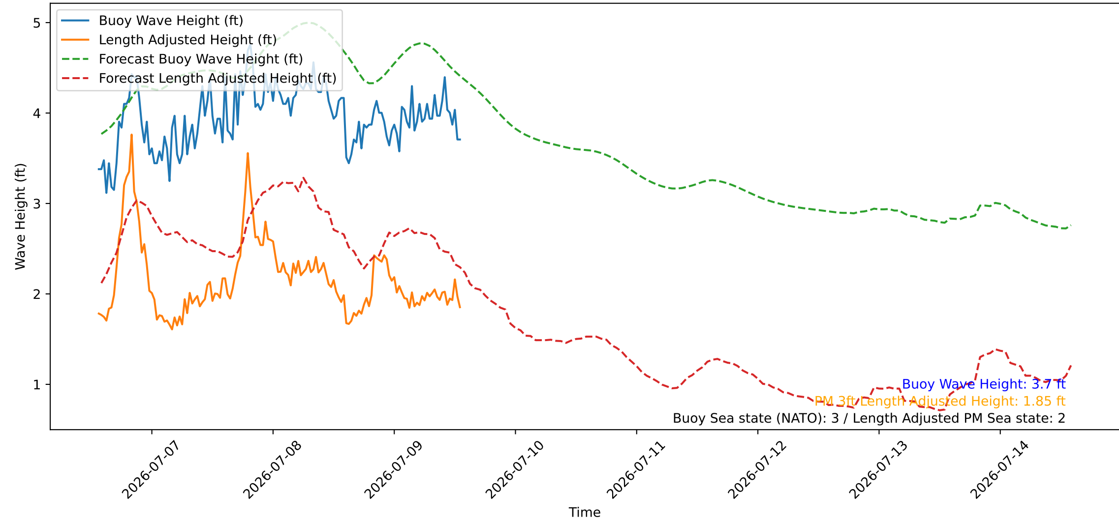
Wave Heights over Time for Green Beach at 2026-07-09 13:41:08
