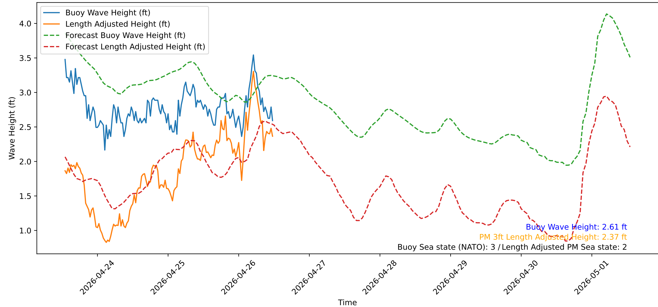
Wave Heights over Time for Red Beach at 2026-04-26 12:30:50
