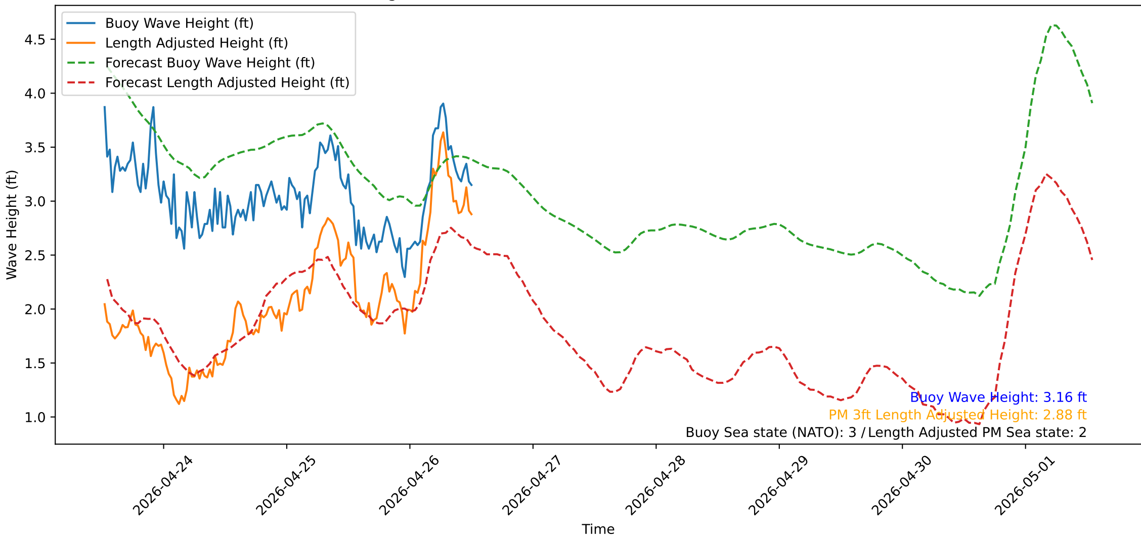
Wave Heights over Time for Oceanside Harbor at 2026-04-26 12:30:31
