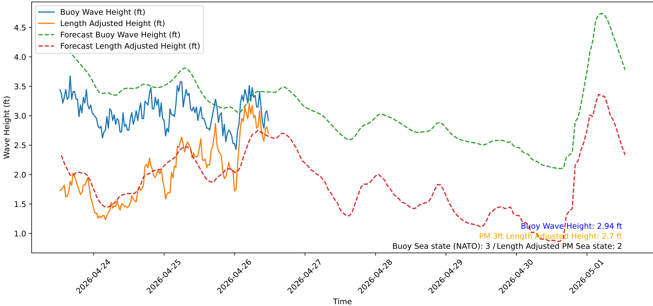
Wave Heights over Time for Green Beach at 2026-04-26 12:31:13
