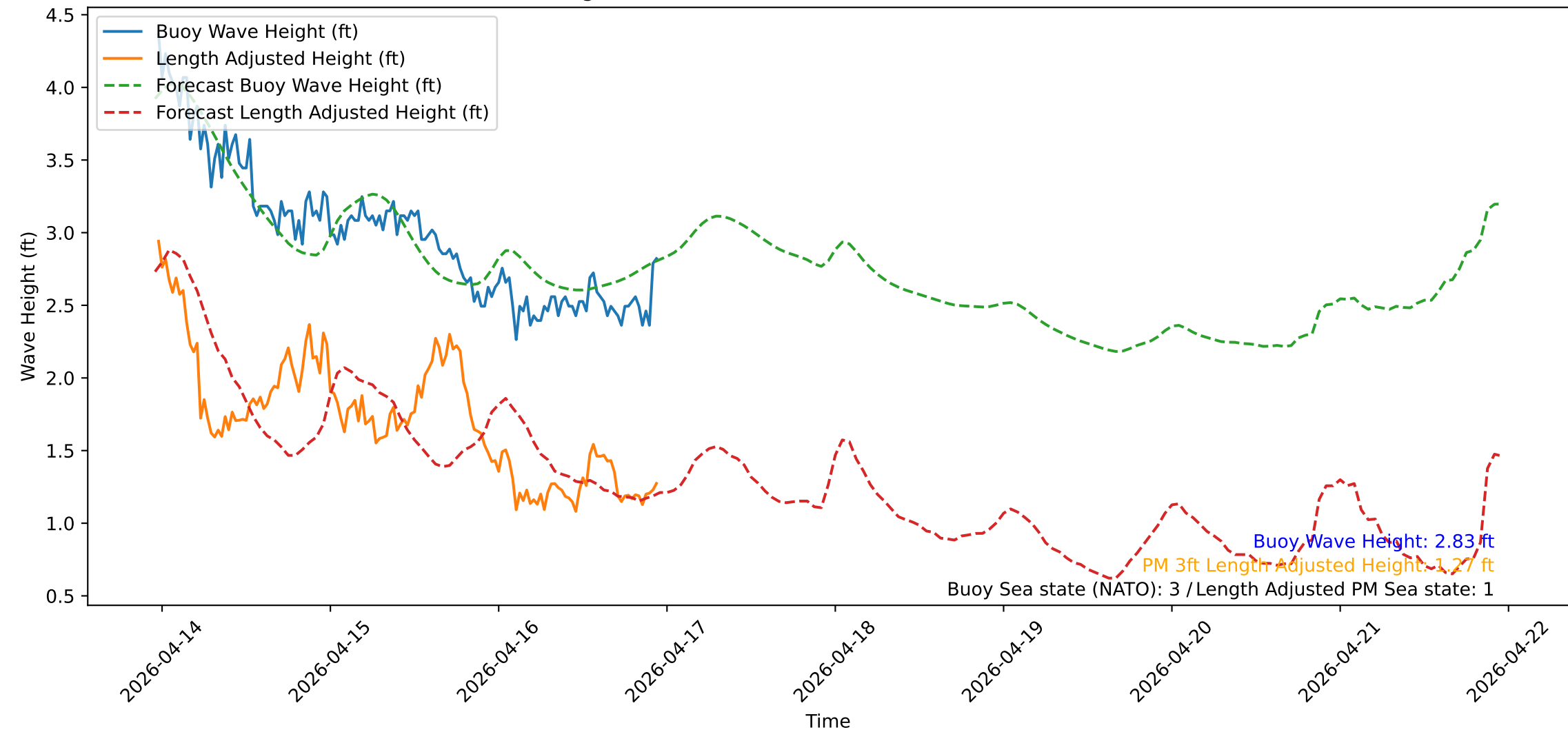
Wave Heights over Time for Red Beach at 2026-04-16 23:10:54
