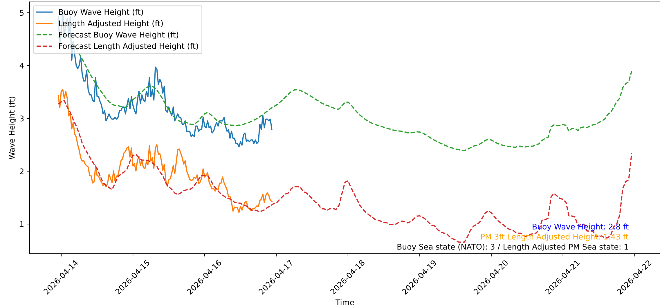
Wave Heights over Time for Green Beach at 2026-04-16 23:11:19
