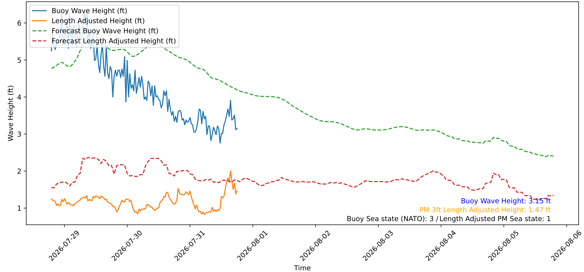
Wave Heights over Time for Green Beach at 2026-07-31 19:01:09
