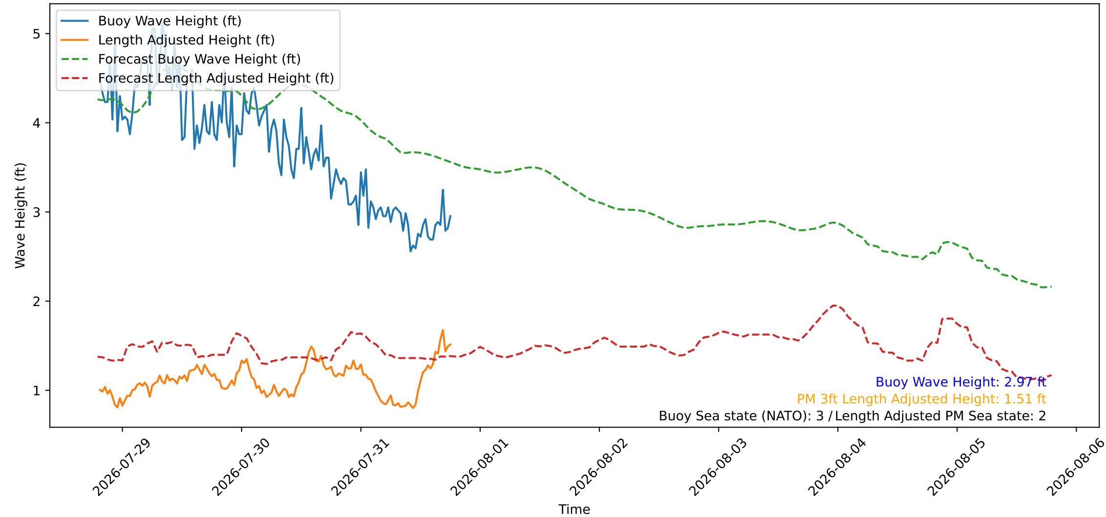
Wave Heights over Time for Red Beach at 2026-07-31 19:00:47
