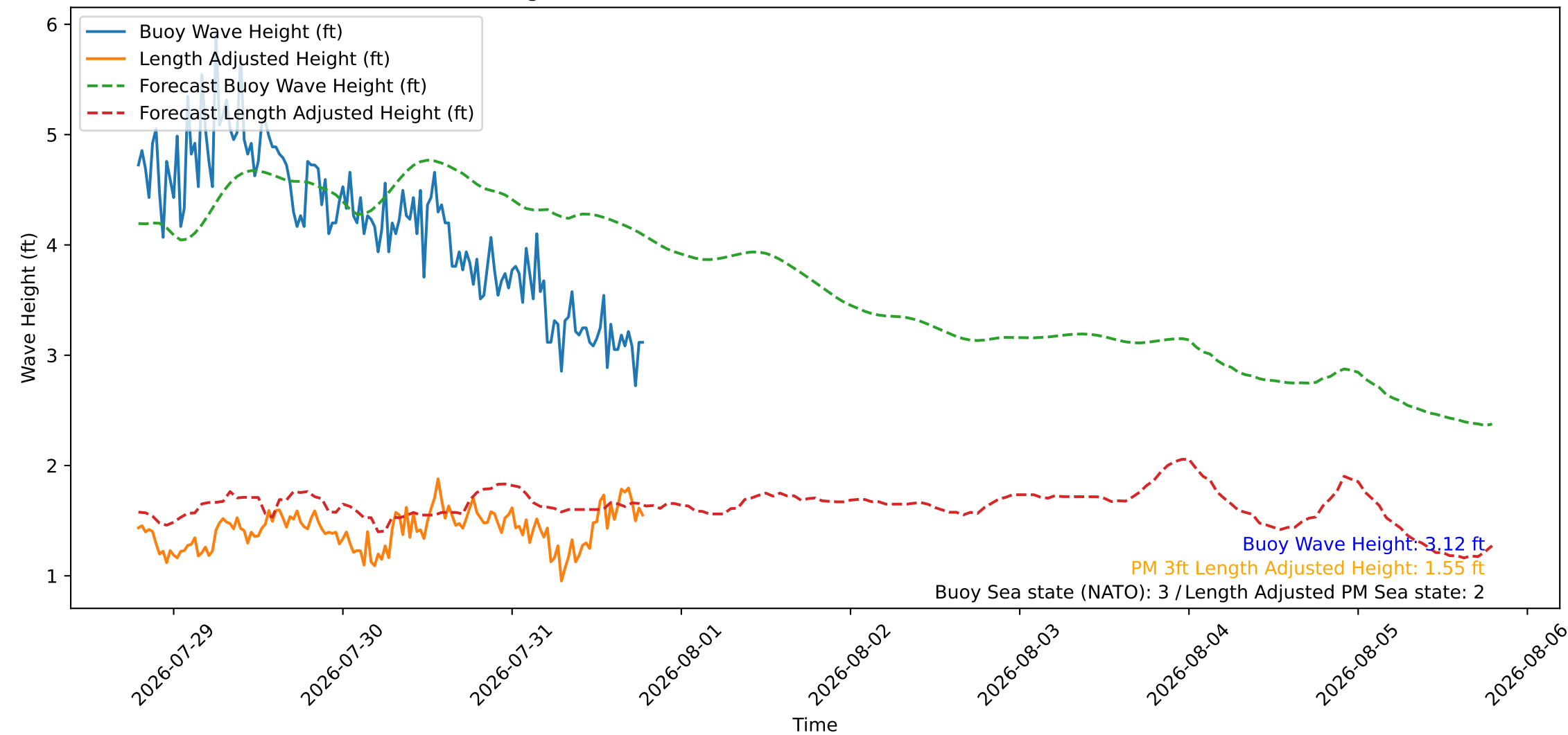
Wave Heights over Time for Oceanside Harbor at 2026-07-31 19:00:27
