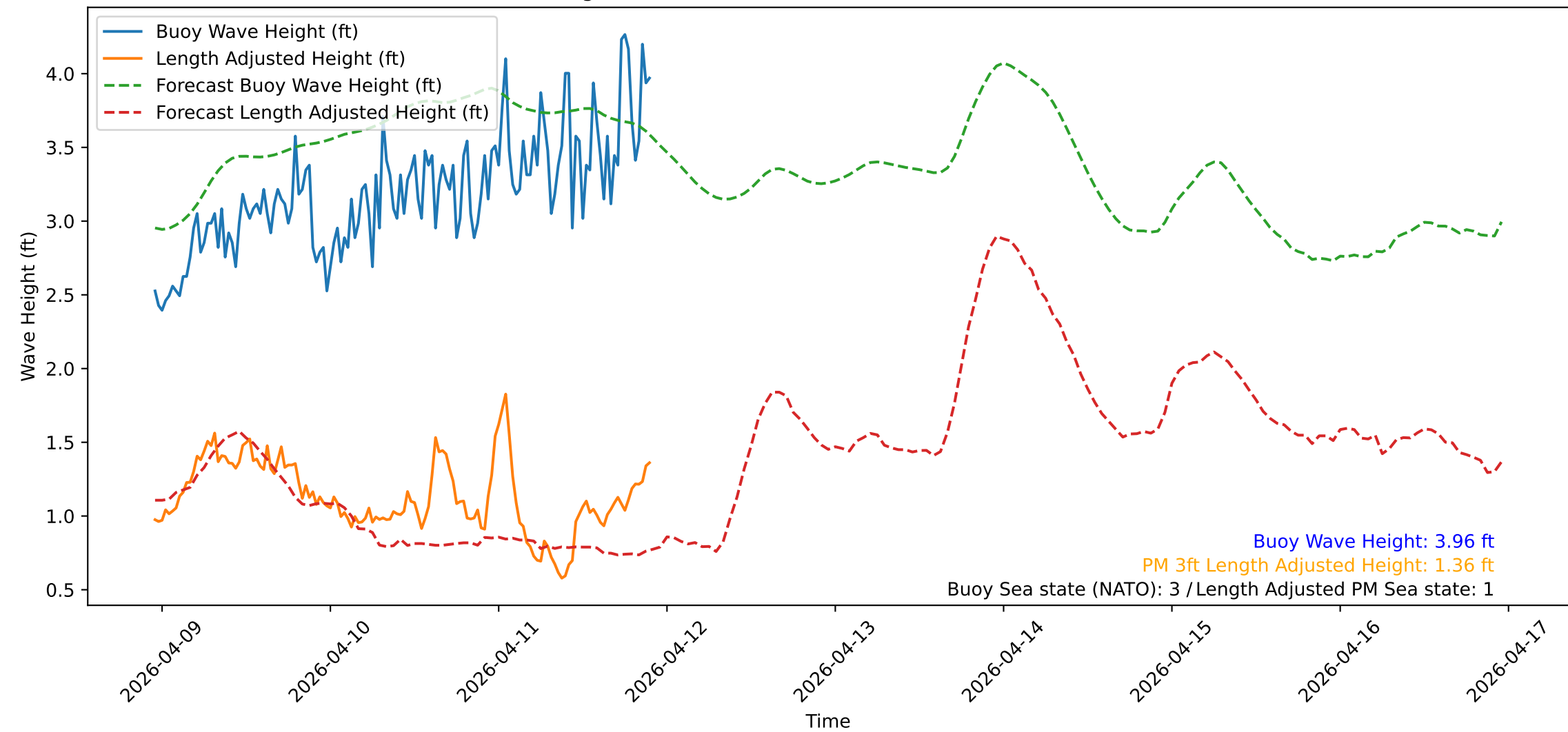
Wave Heights over Time for Red Beach at 2026-04-11 22:40:51
