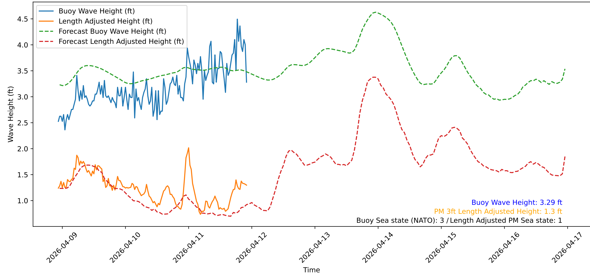
Wave Heights over Time for Green Beach at 2026-04-11 22:41:14
