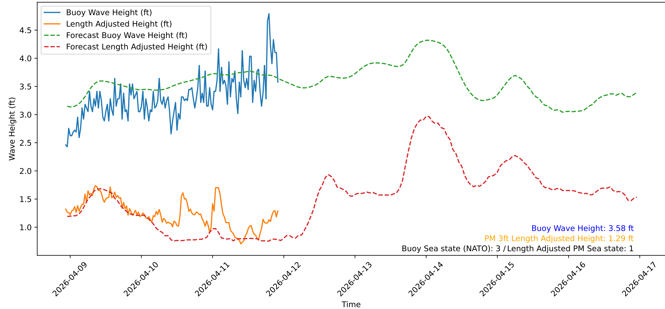
Wave Heights over Time for Oceanside Harbor at 2026-04-11 22:40:31
