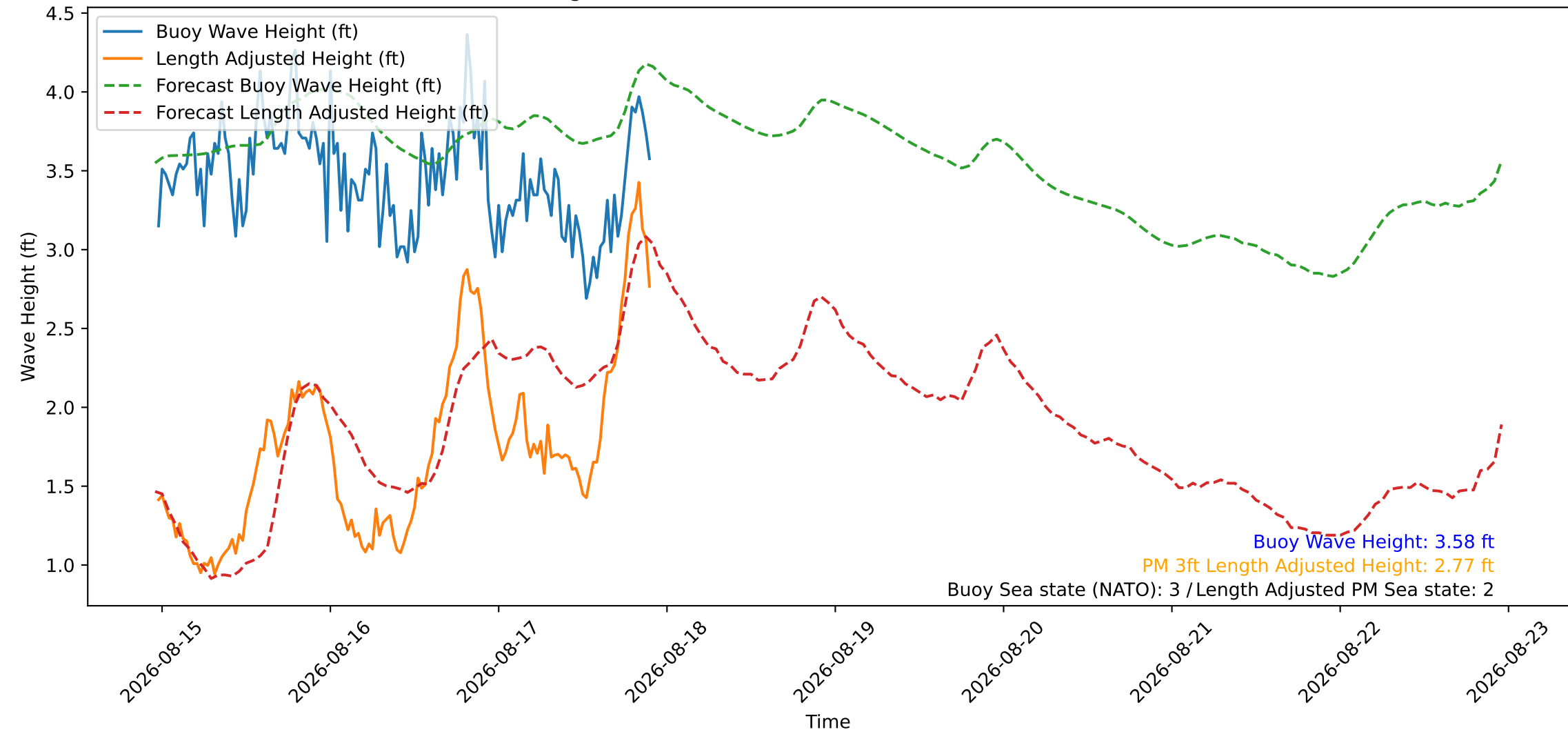
Wave Heights over Time for Green Beach at 2026-08-17 23:01:09
