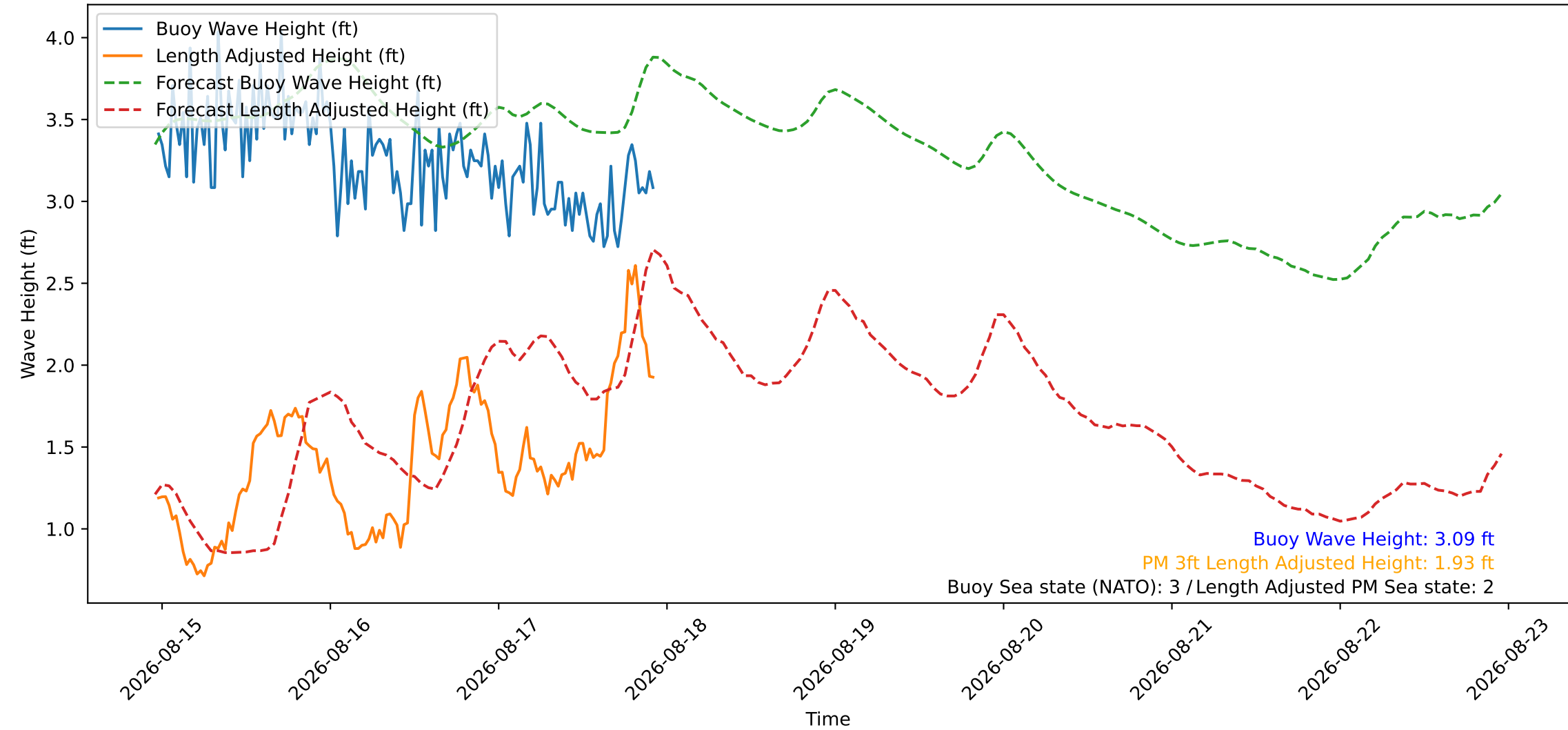
Wave Heights over Time for Red Beach at 2026-08-17 23:00:46
