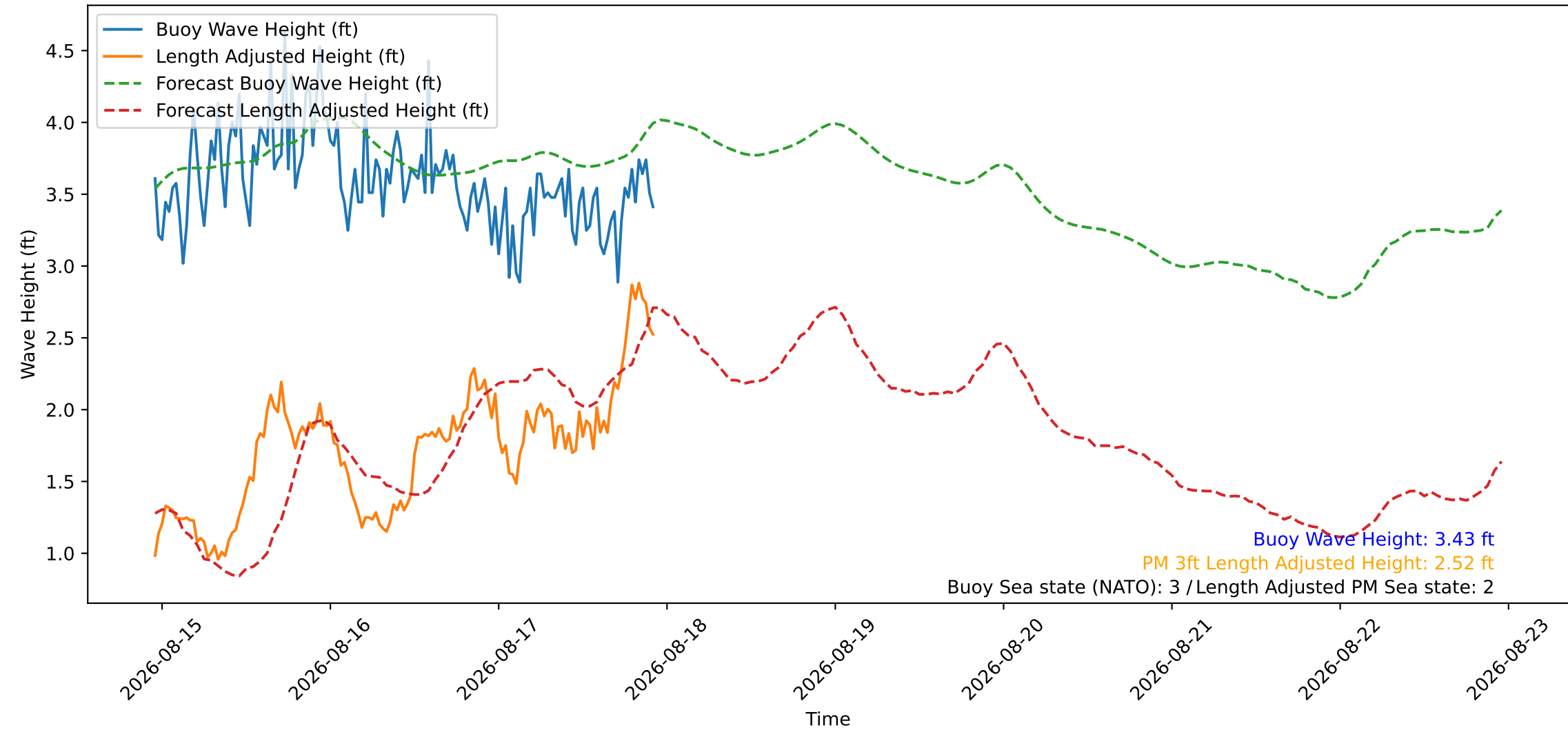
Wave Heights over Time for Oceanside Harbor at 2026-08-17 23:00:26
