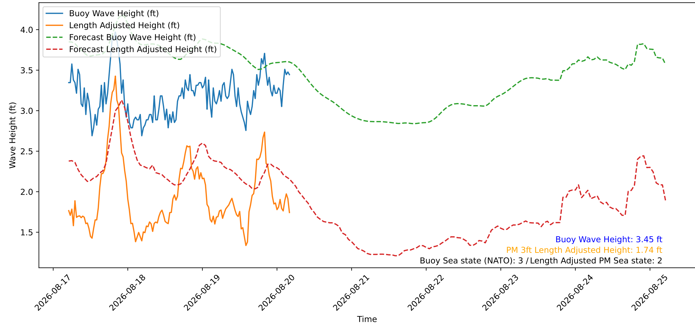
Wave Heights over Time for Green Beach at 2026-08-20 04:41:09
