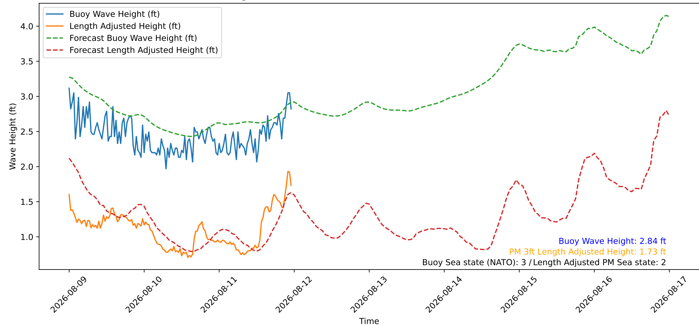
Wave Heights over Time for Oceanside Harbor at 2026-08-12 00:00:26
