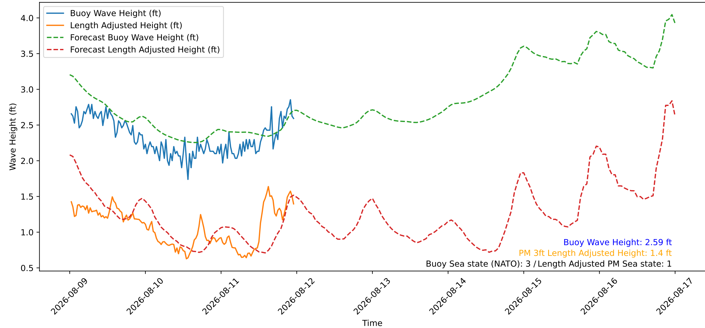
Wave Heights over Time for Red Beach at 2026-08-12 00:00:45
