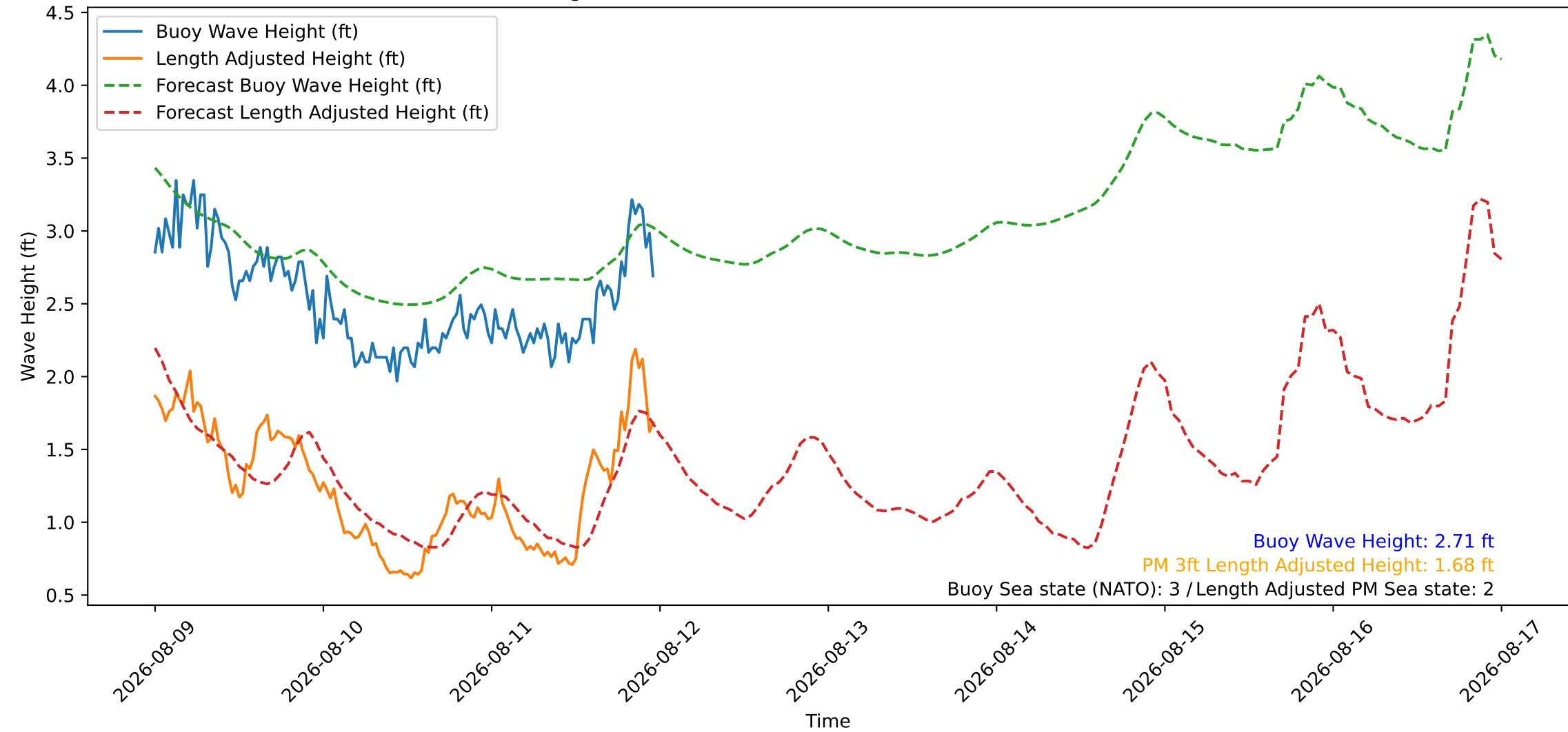
Wave Heights over Time for Green Beach at 2026-08-12 00:01:08
