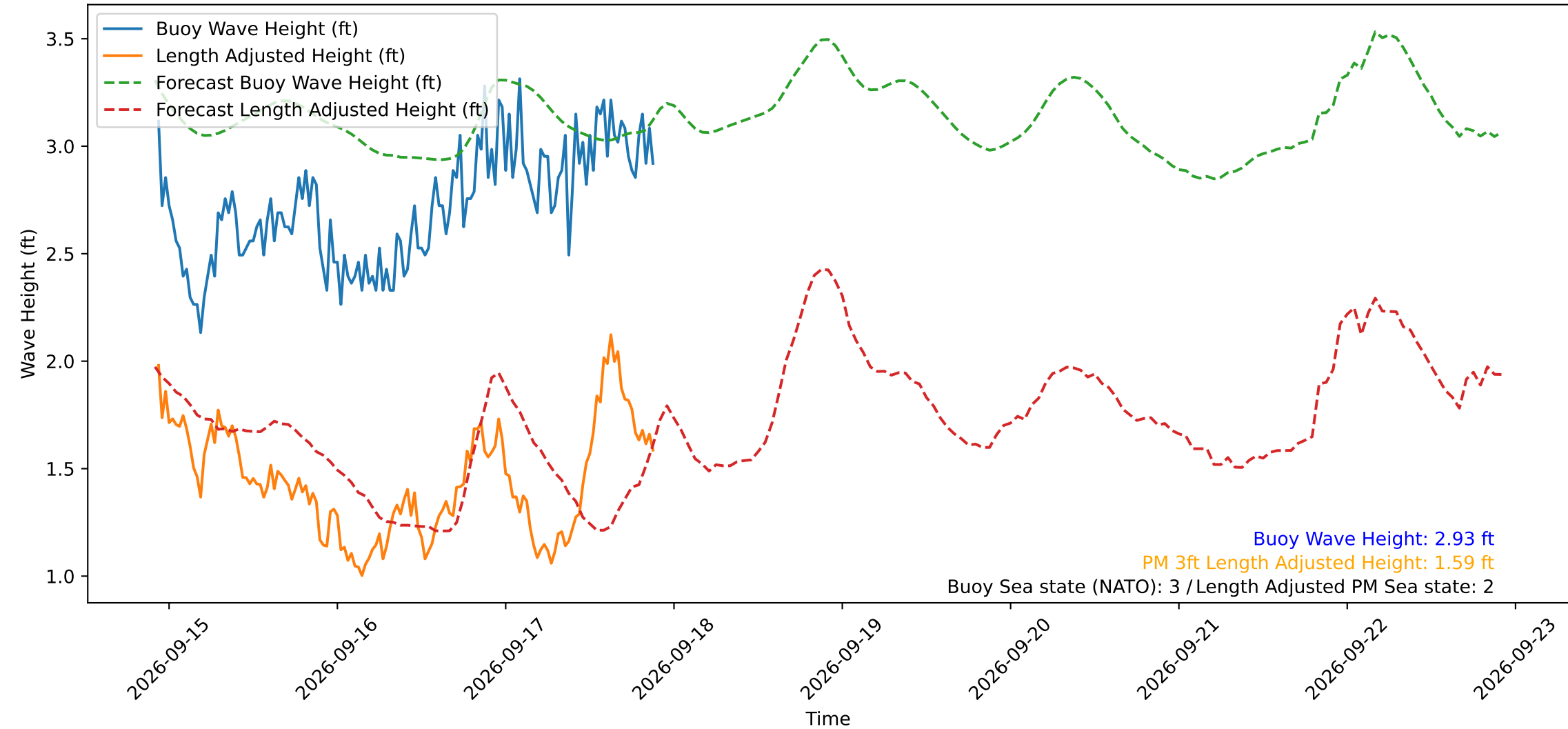
Wave Heights over Time for Green Beach at 2026-09-17 22:01:12
