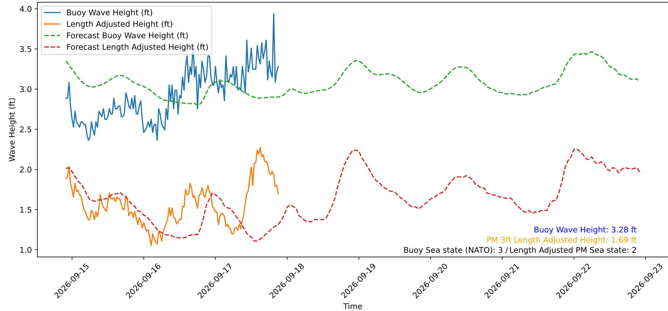
Wave Heights over Time for Oceanside Harbor at 2026-09-17 22:00:30
