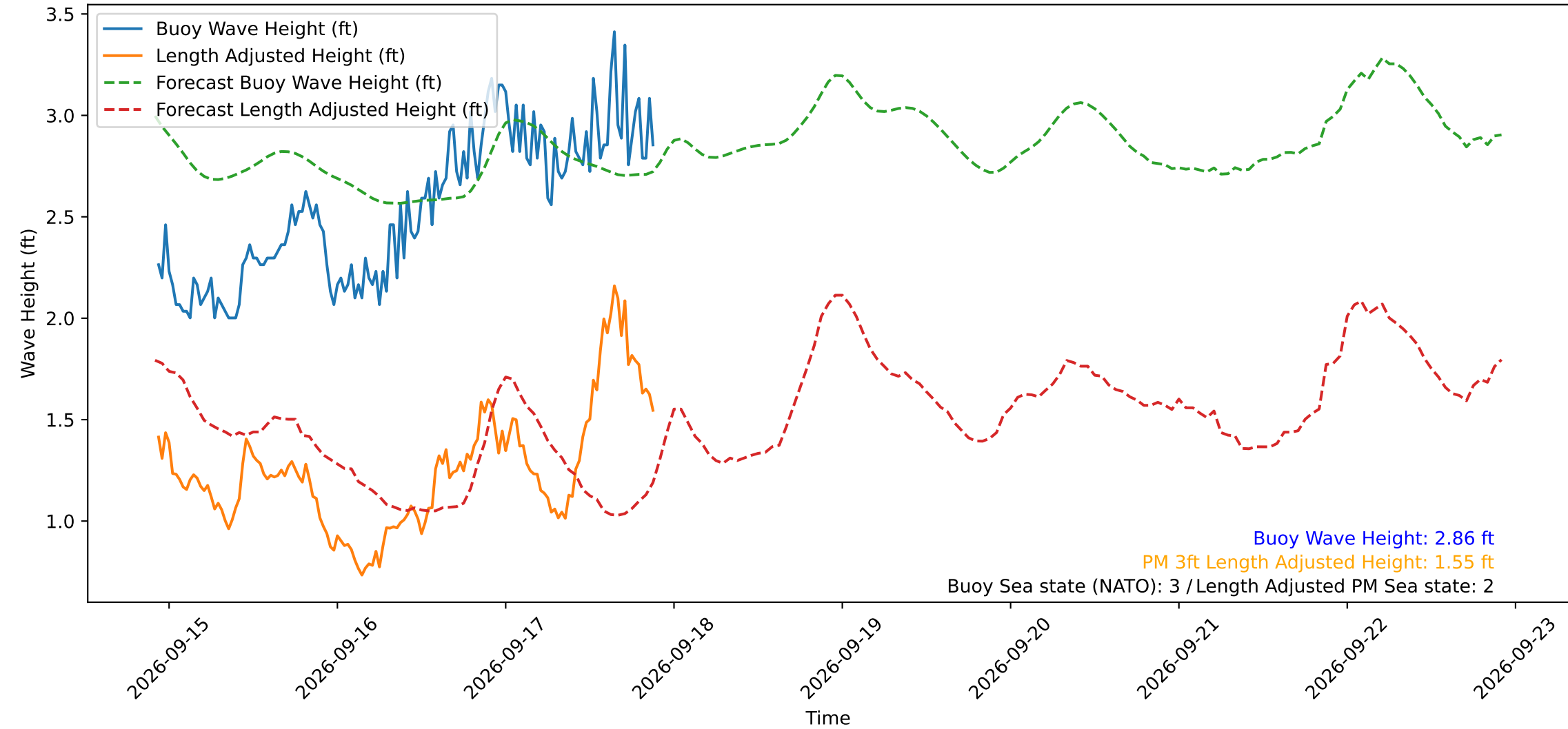
Wave Heights over Time for Red Beach at 2026-09-17 22:00:50
