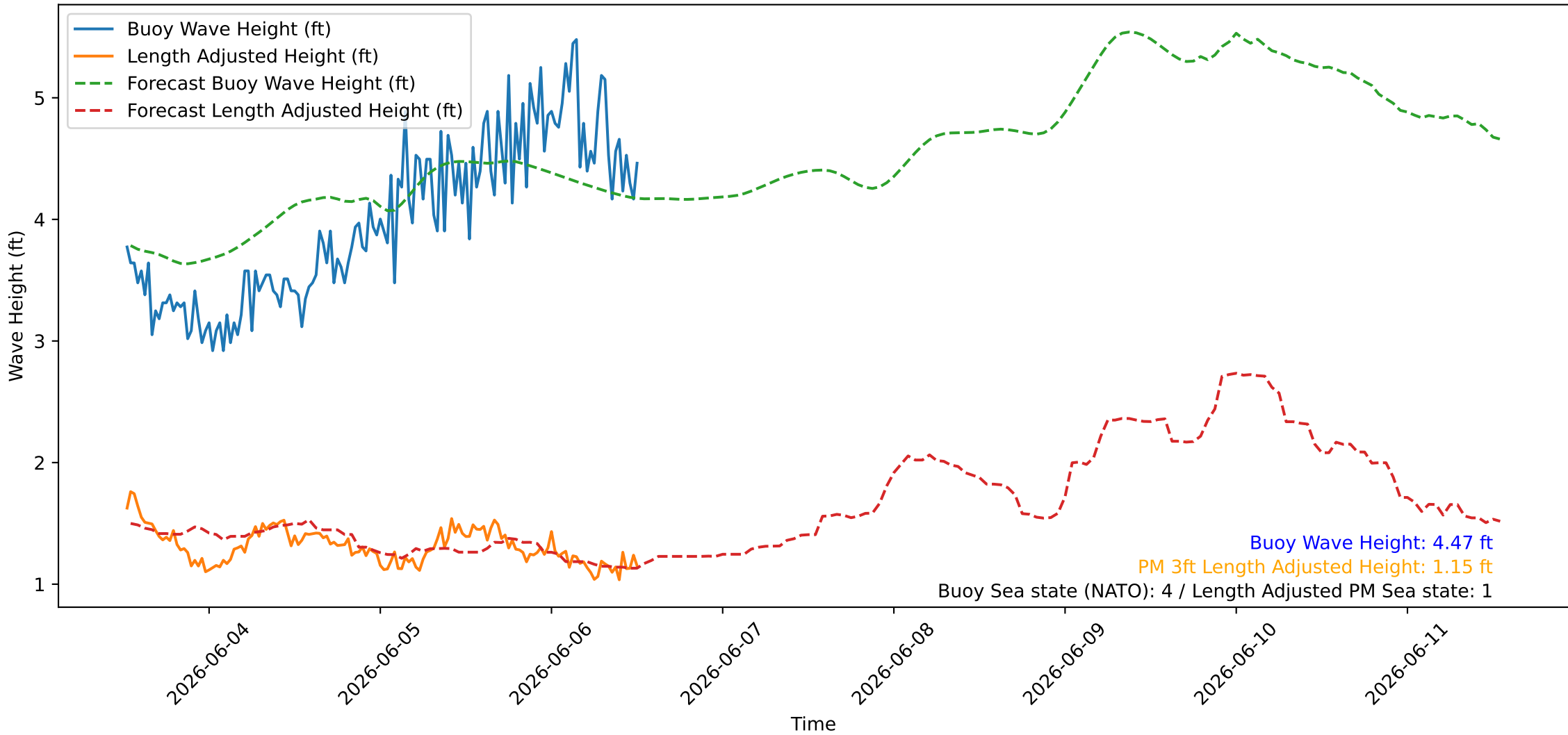
Wave Heights over Time for Oceanside Harbor at 2026-06-06 12:40:26
