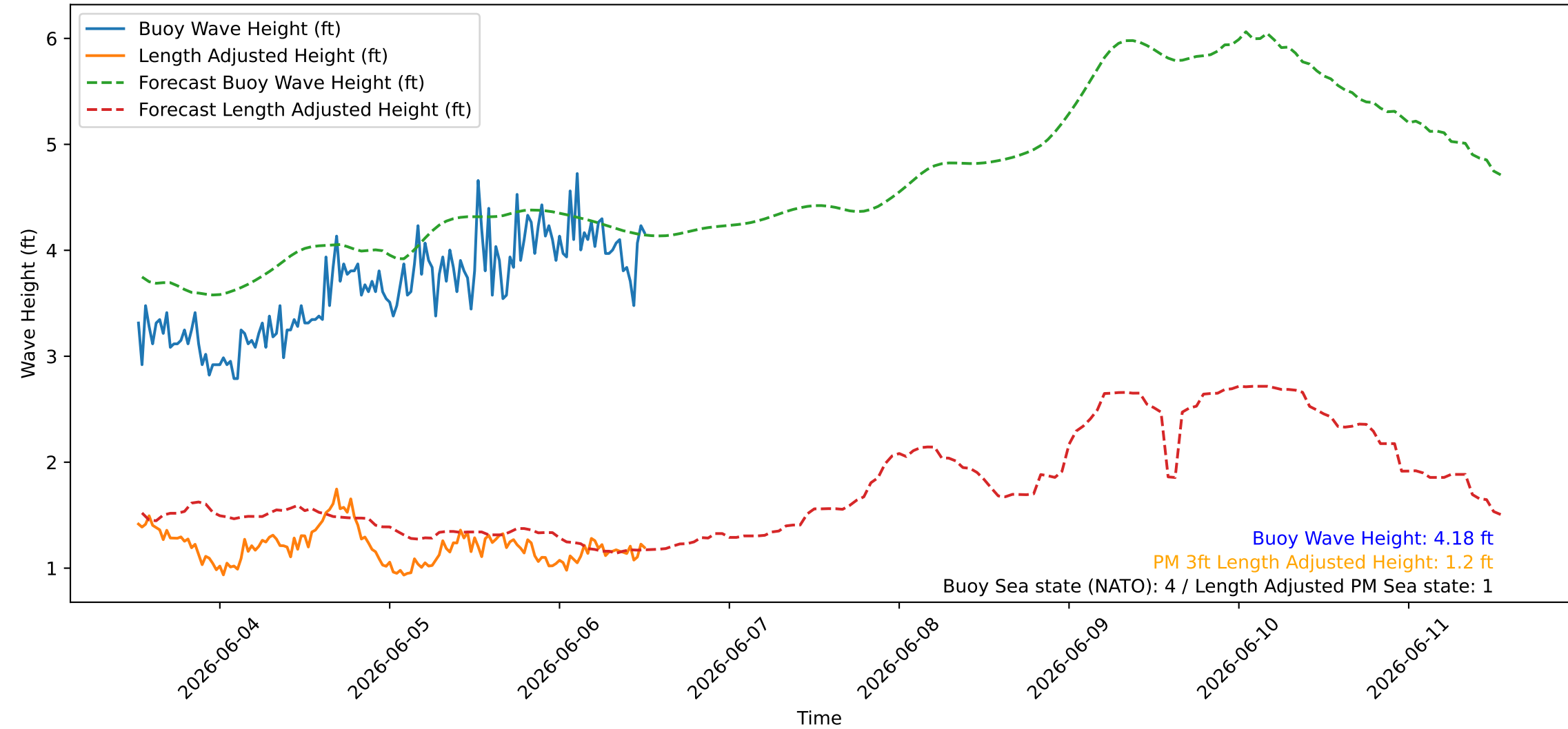
Wave Heights over Time for Green Beach at 2026-06-06 12:41:08
