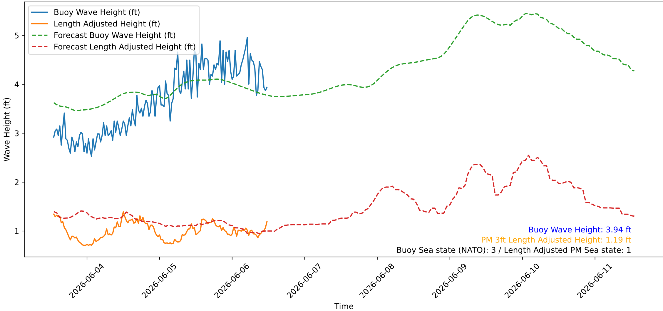
Wave Heights over Time for Red Beach at 2026-06-06 12:40:45
