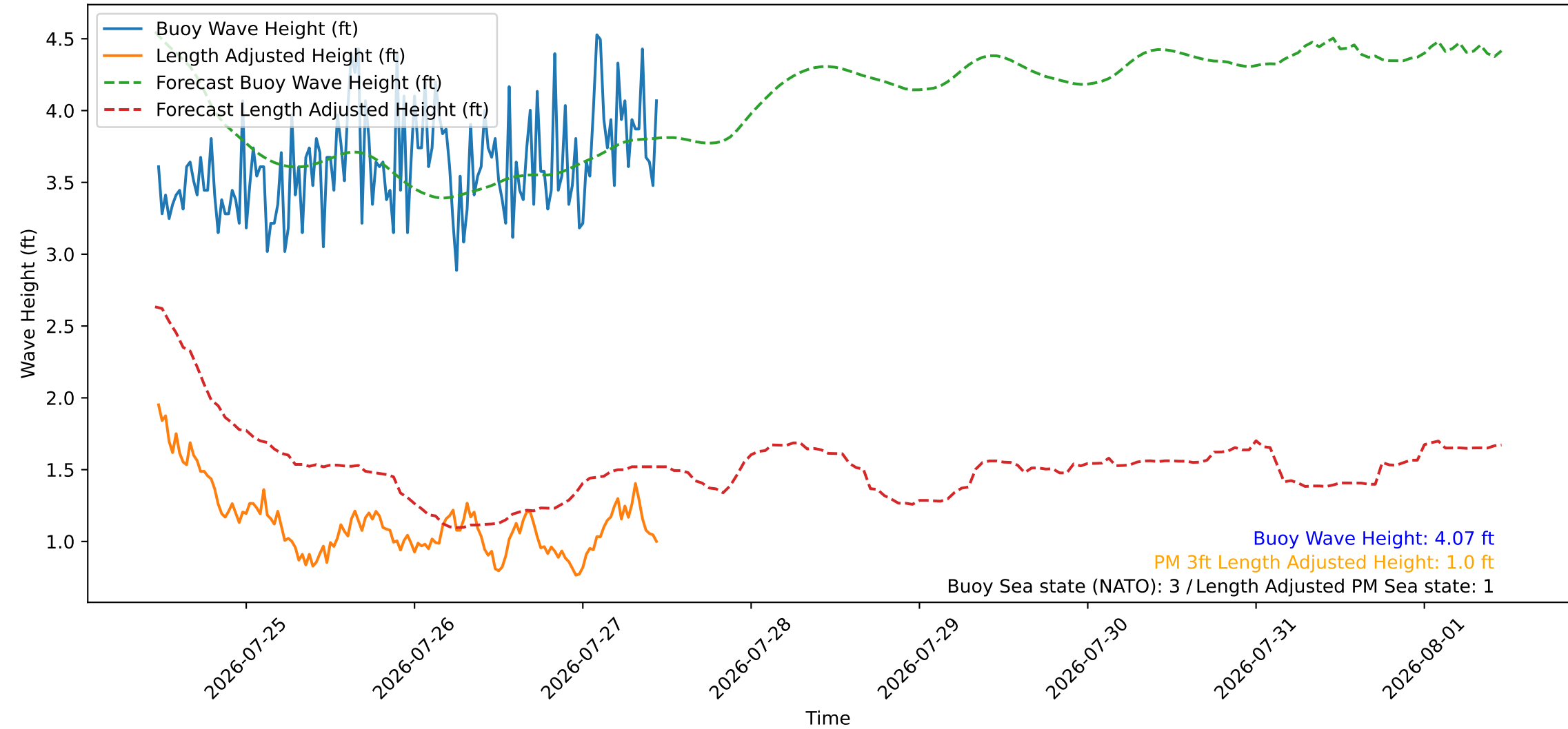
Wave Heights over Time for Red Beach at 2026-07-27 11:10:45
