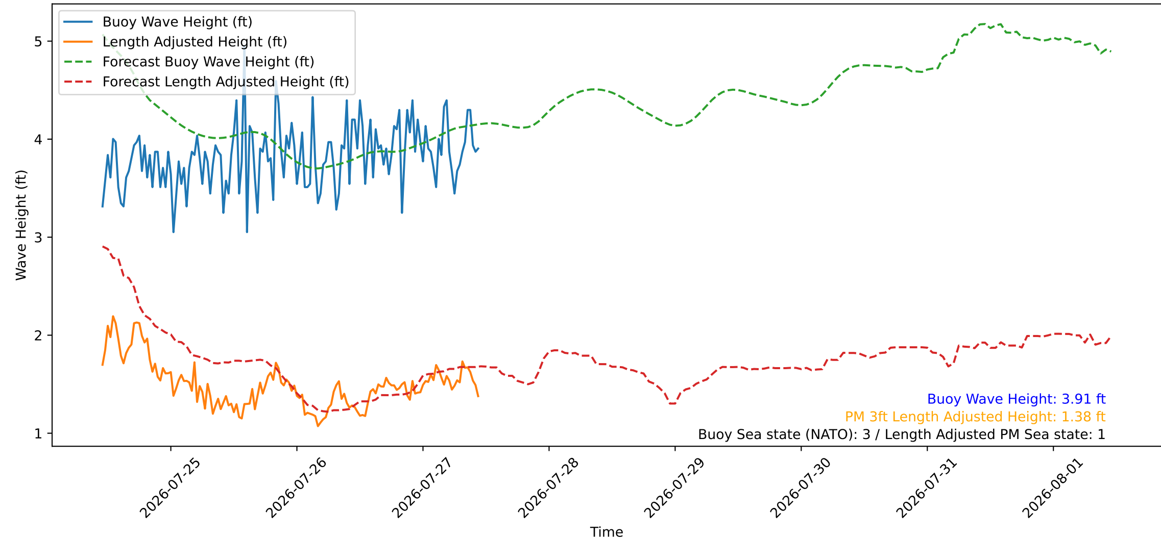
Wave Heights over Time for Oceanside Harbor at 2026-07-27 11:10:26
