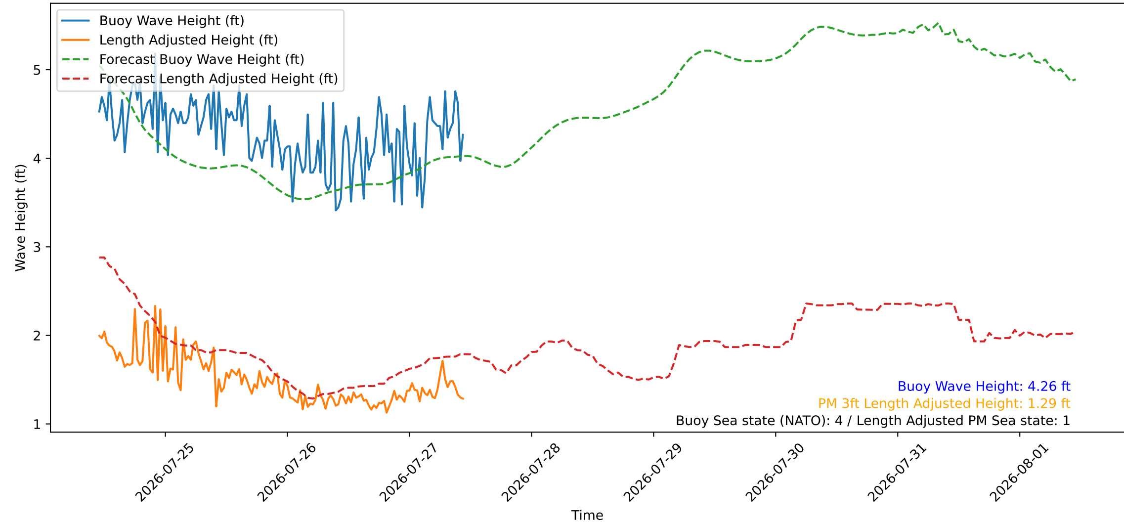
Wave Heights over Time for Green Beach at 2026-07-27 11:11:08
