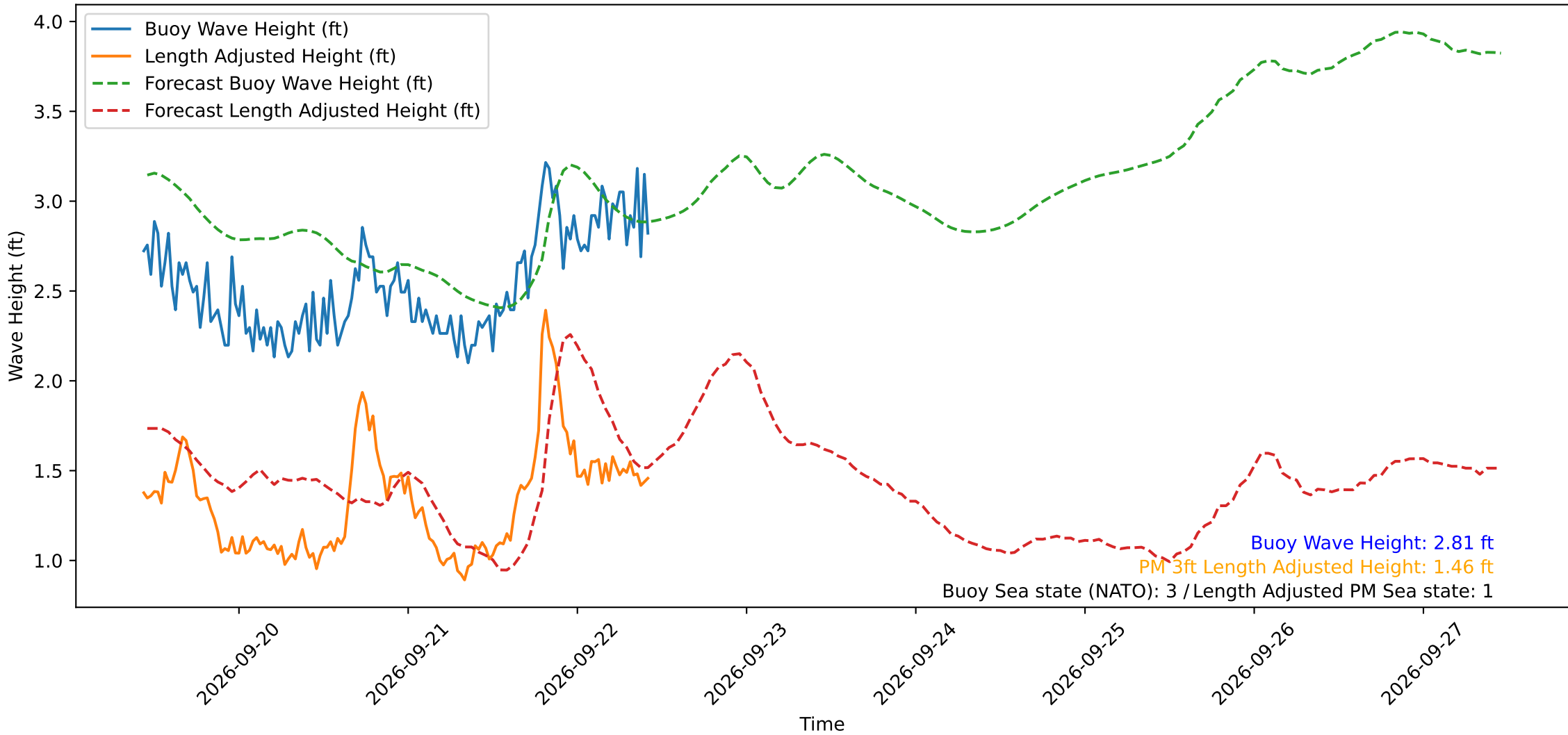
Wave Heights over Time for Oceanside Harbor at 2026-09-22 10:40:30
