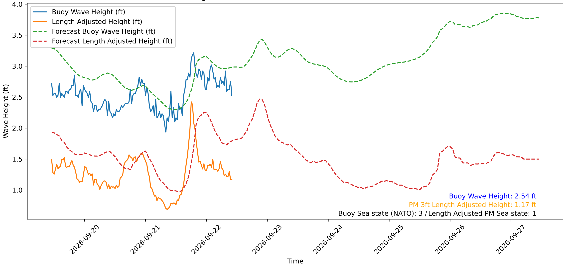
Wave Heights over Time for Green Beach at 2026-09-22 10:41:11
