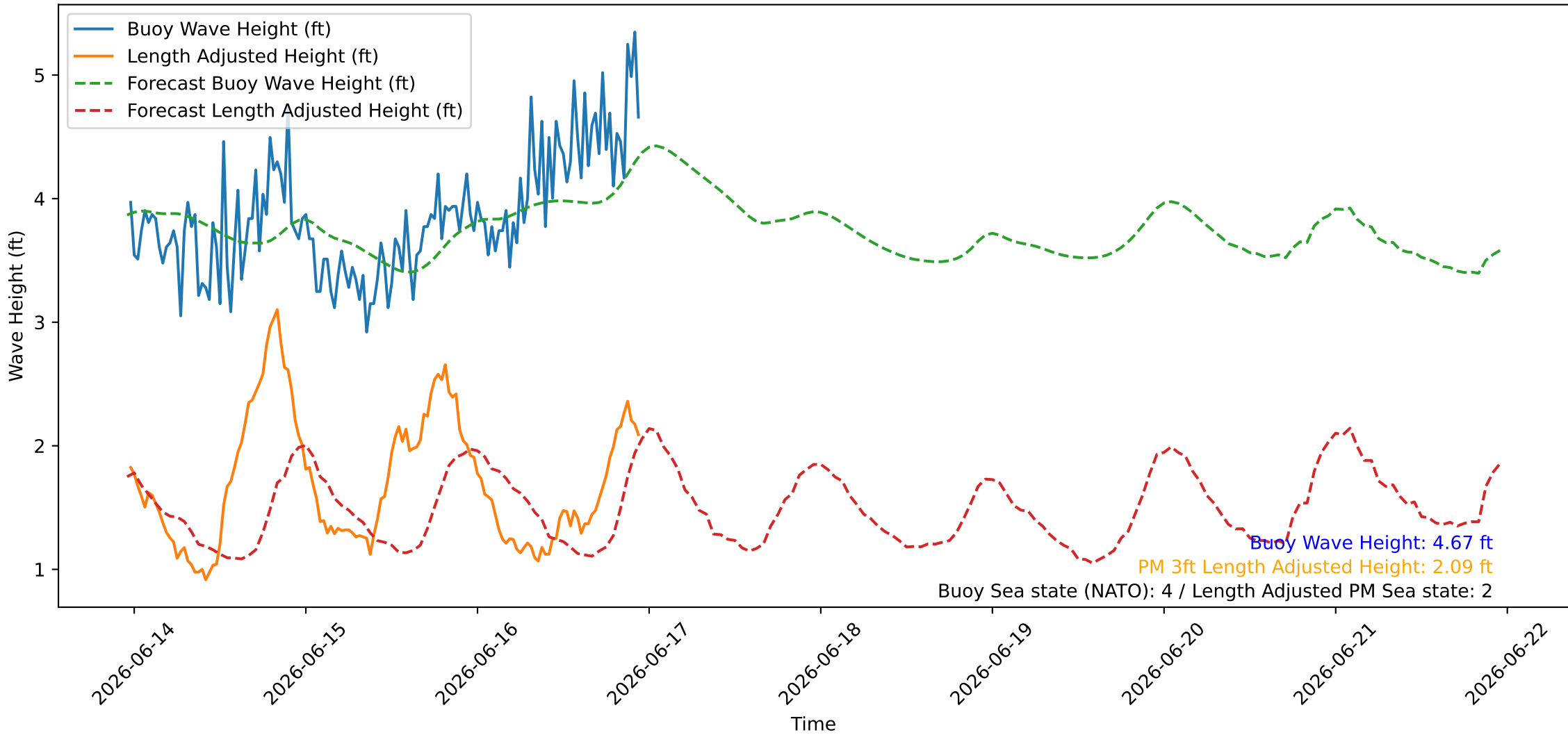
Wave Heights over Time for Red Beach at 2026-06-16 23:20:46
