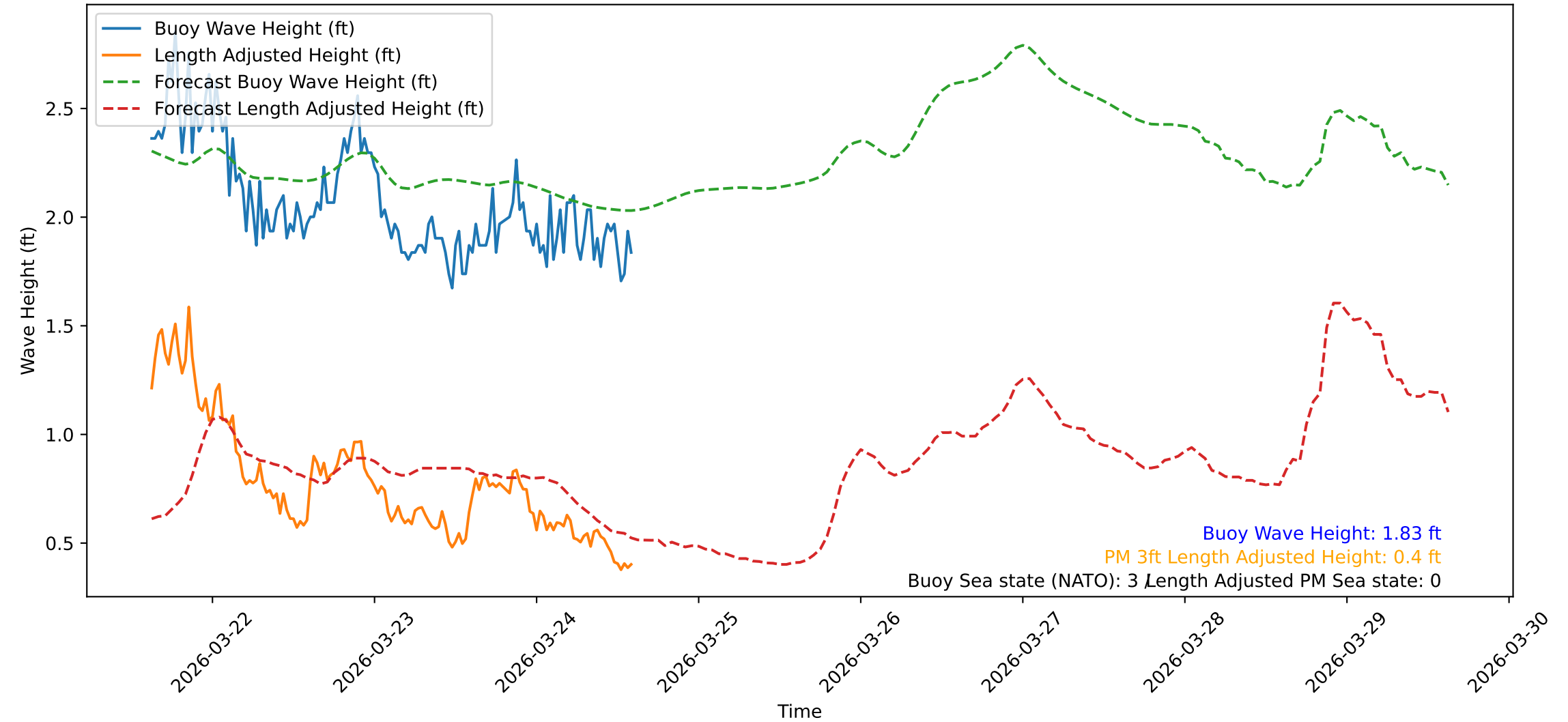
Wave Heights over Time for Red Beach at 2026-03-24 14:40:47
