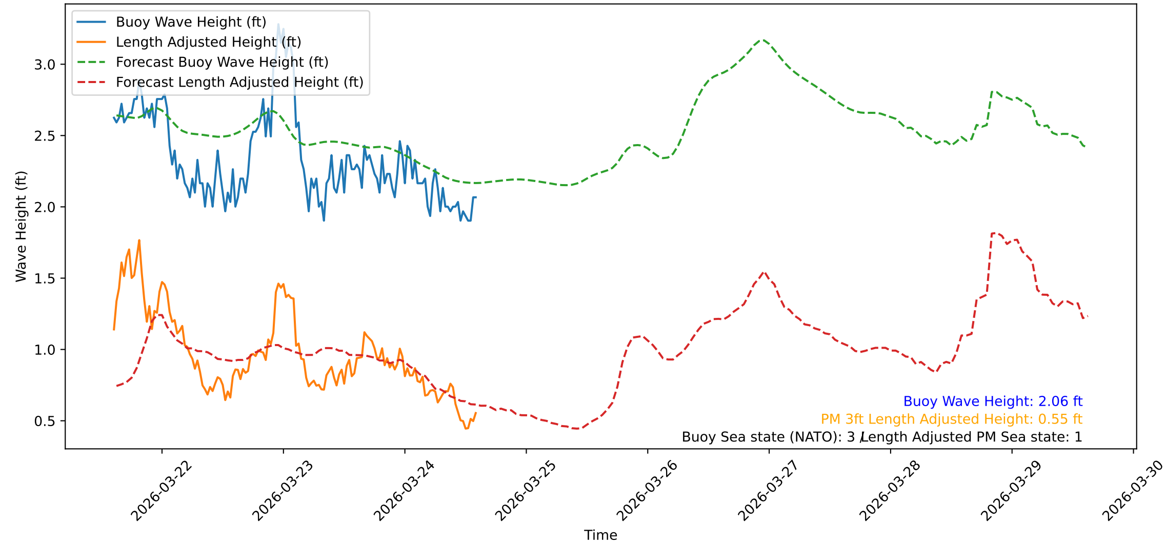
Wave Heights over Time for Green Beach at 2026-03-24 14:41:10
