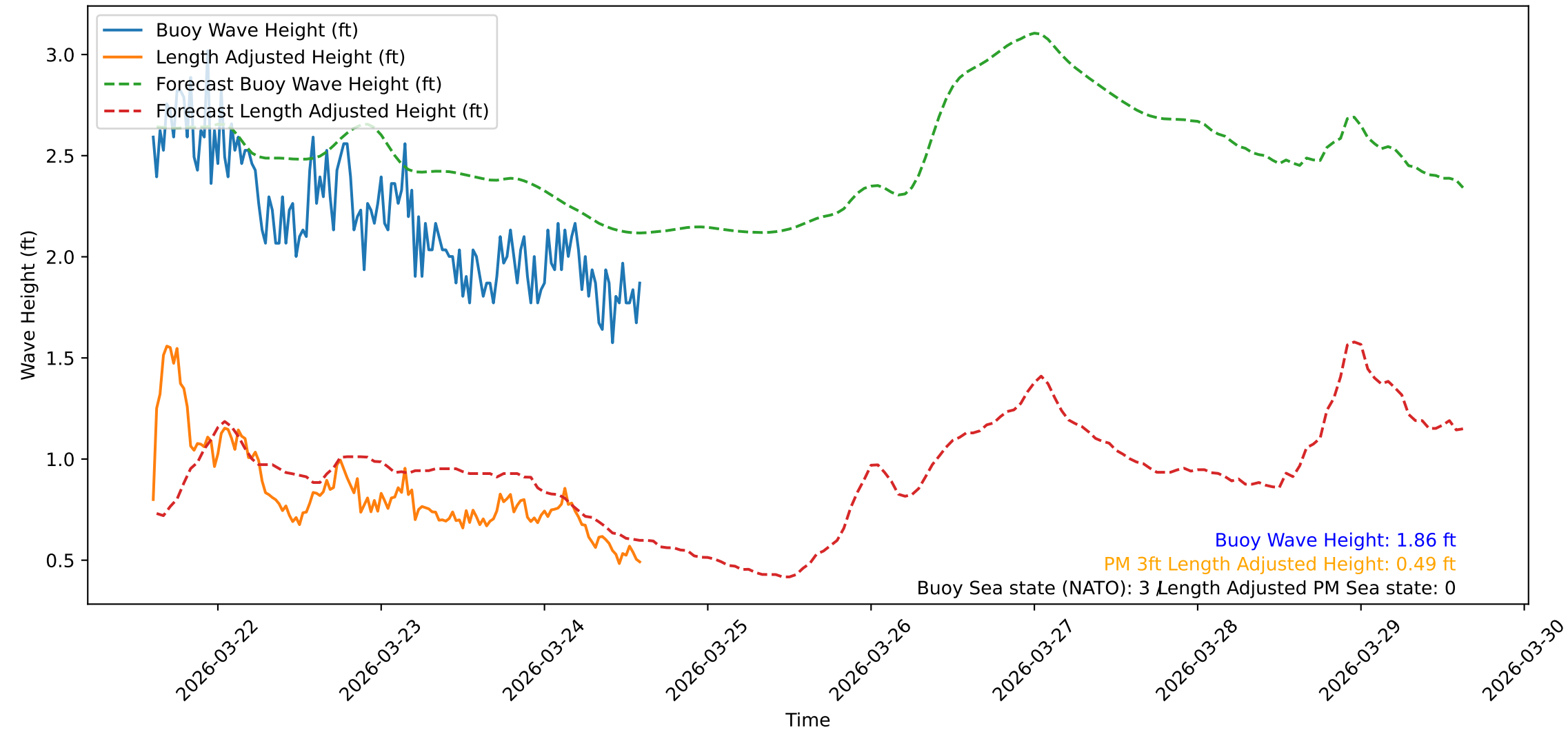
Wave Heights over Time for Oceanside Harbor at 2026-03-24 14:40:31
