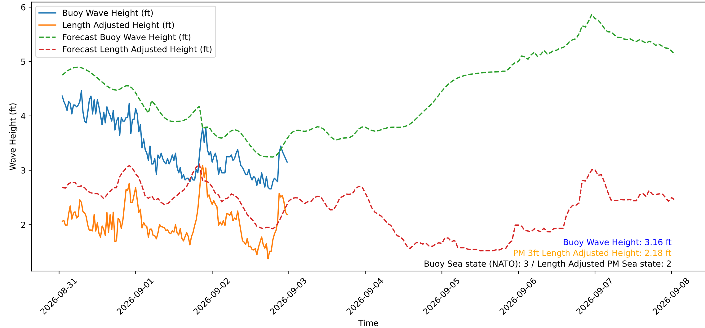
Wave Heights over Time for Green Beach at 2026-09-03 00:31:12
