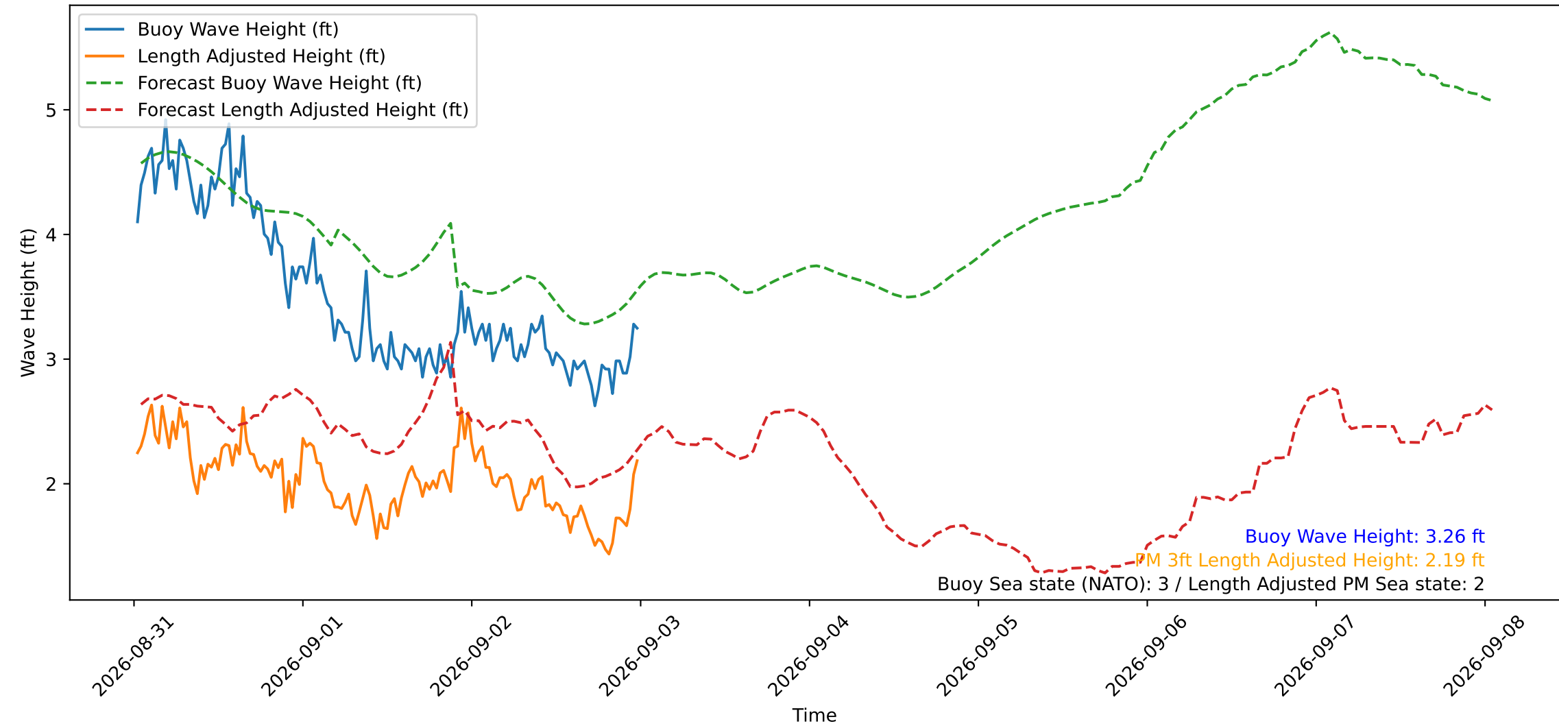
Wave Heights over Time for Oceanside Harbor at 2026-09-03 00:30:29
