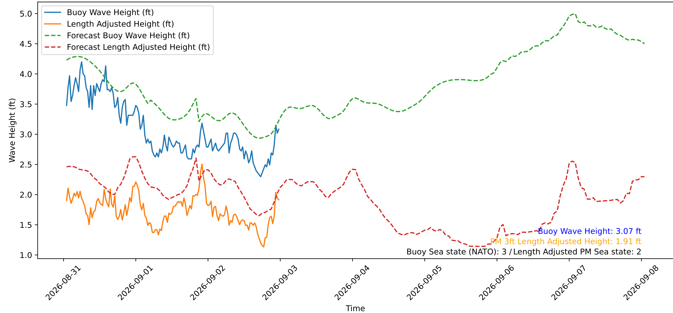
Wave Heights over Time for Red Beach at 2026-09-03 00:30:49
