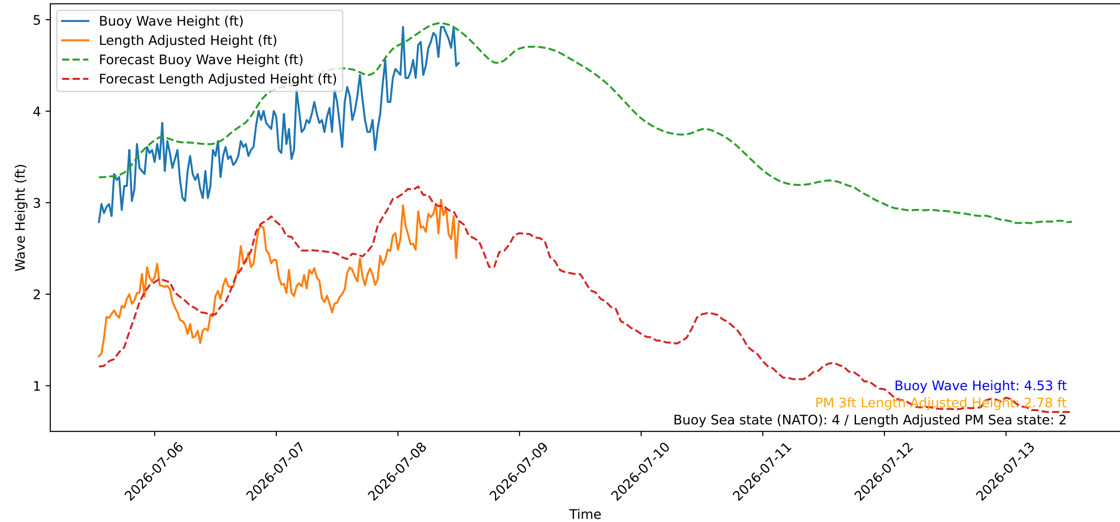
Wave Heights over Time for Oceanside Harbor at 2026-07-08 12:50:27
