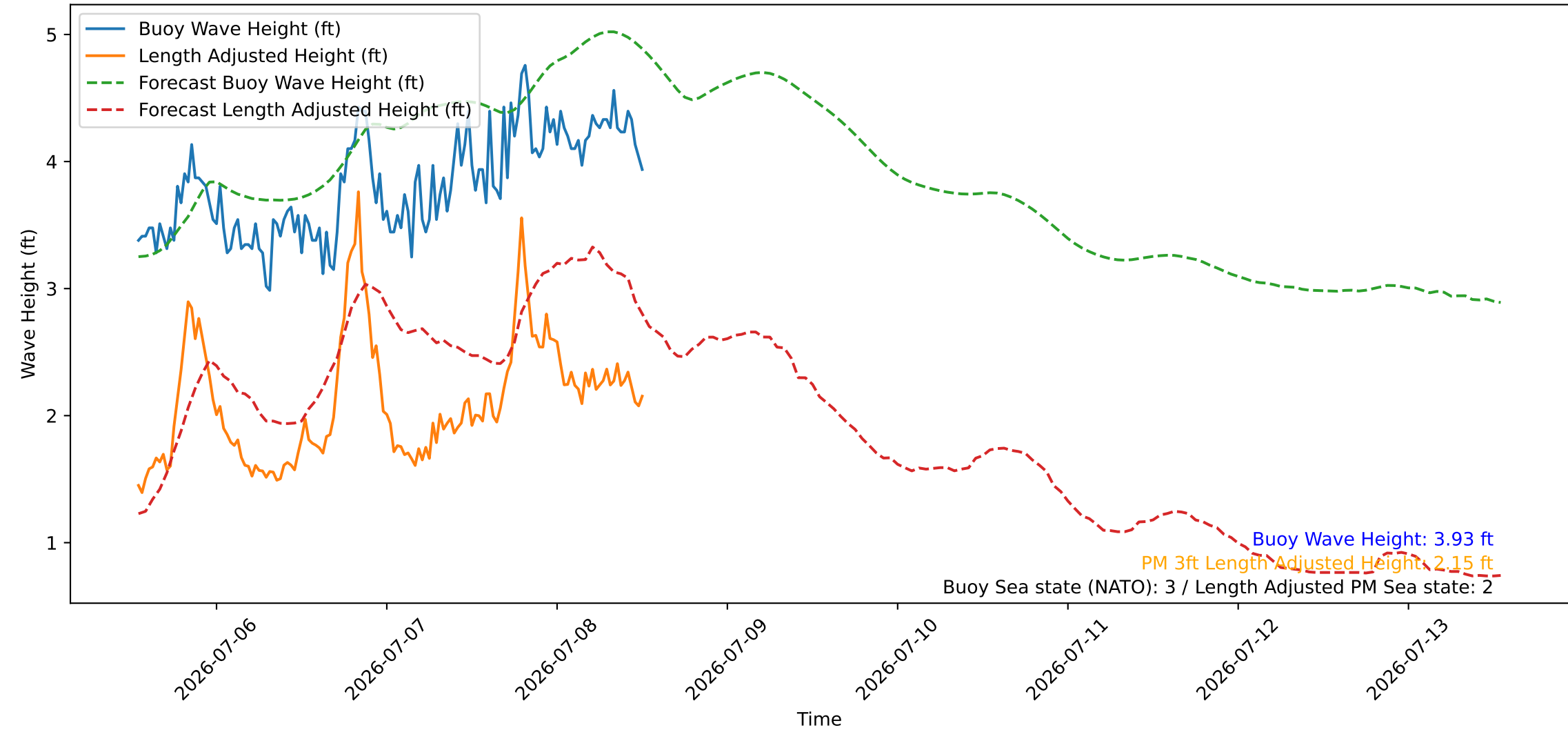
Wave Heights over Time for Green Beach at 2026-07-08 12:51:10
