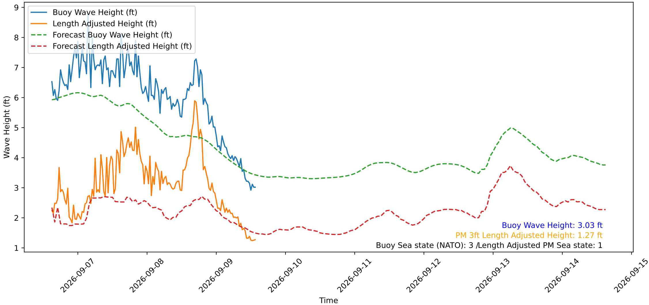
Wave Heights over Time for Green Beach at 2026-09-09 14:31:11
