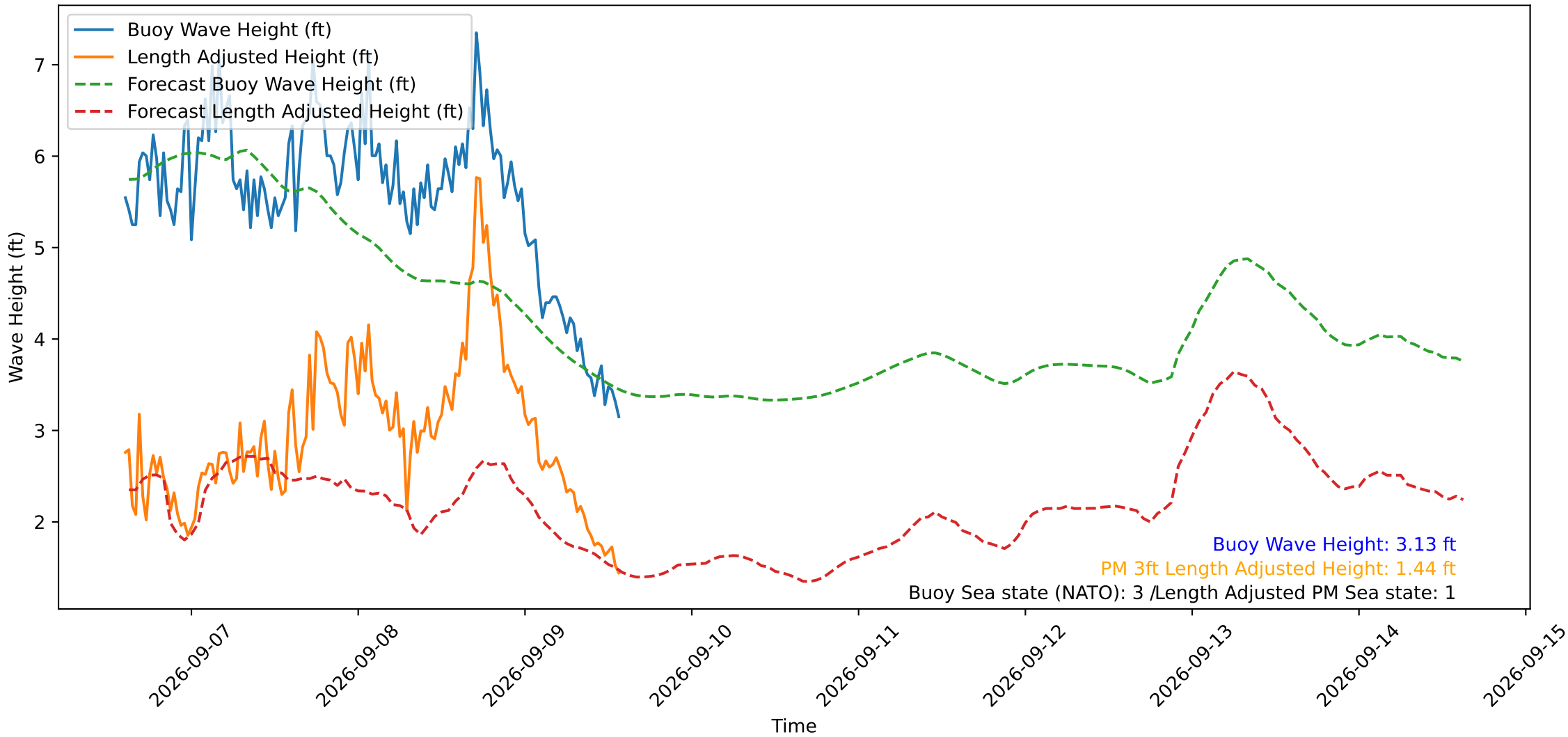
Wave Heights over Time for Oceanside Harbor at 2026-09-09 14:30:30
