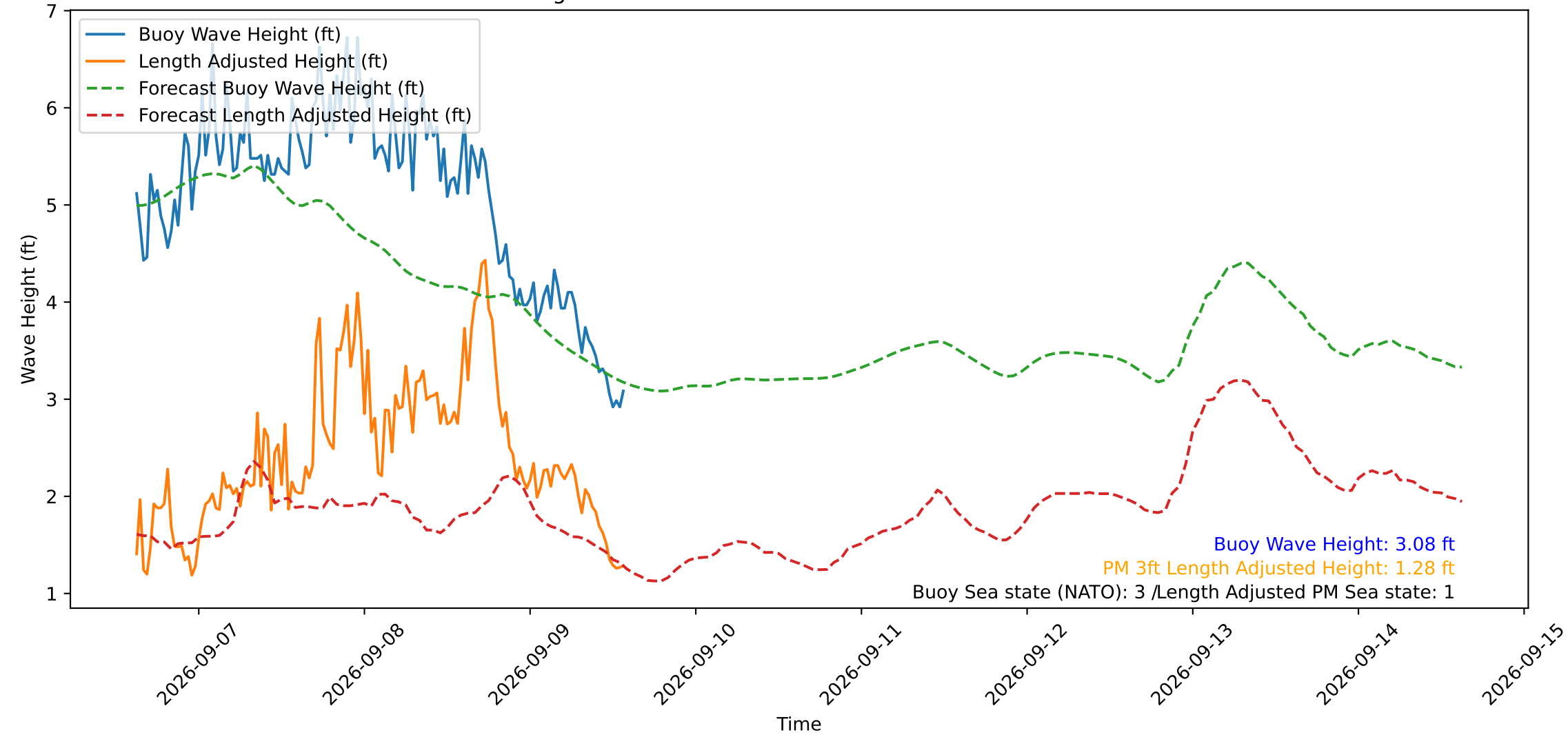
Wave Heights over Time for Red Beach at 2026-09-09 14:30:49
