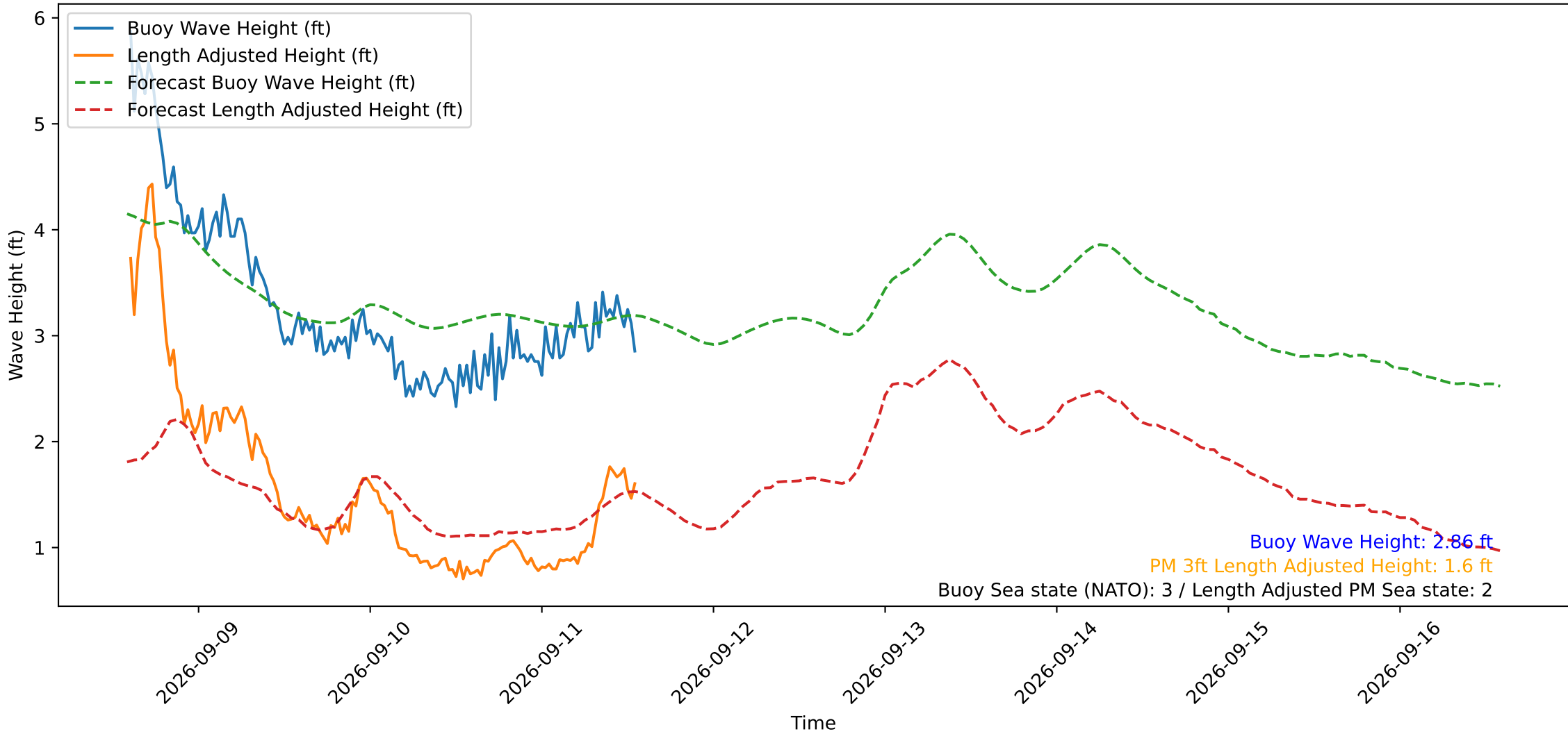
Wave Heights over Time for Red Beach at 2026-09-11 14:10:49
