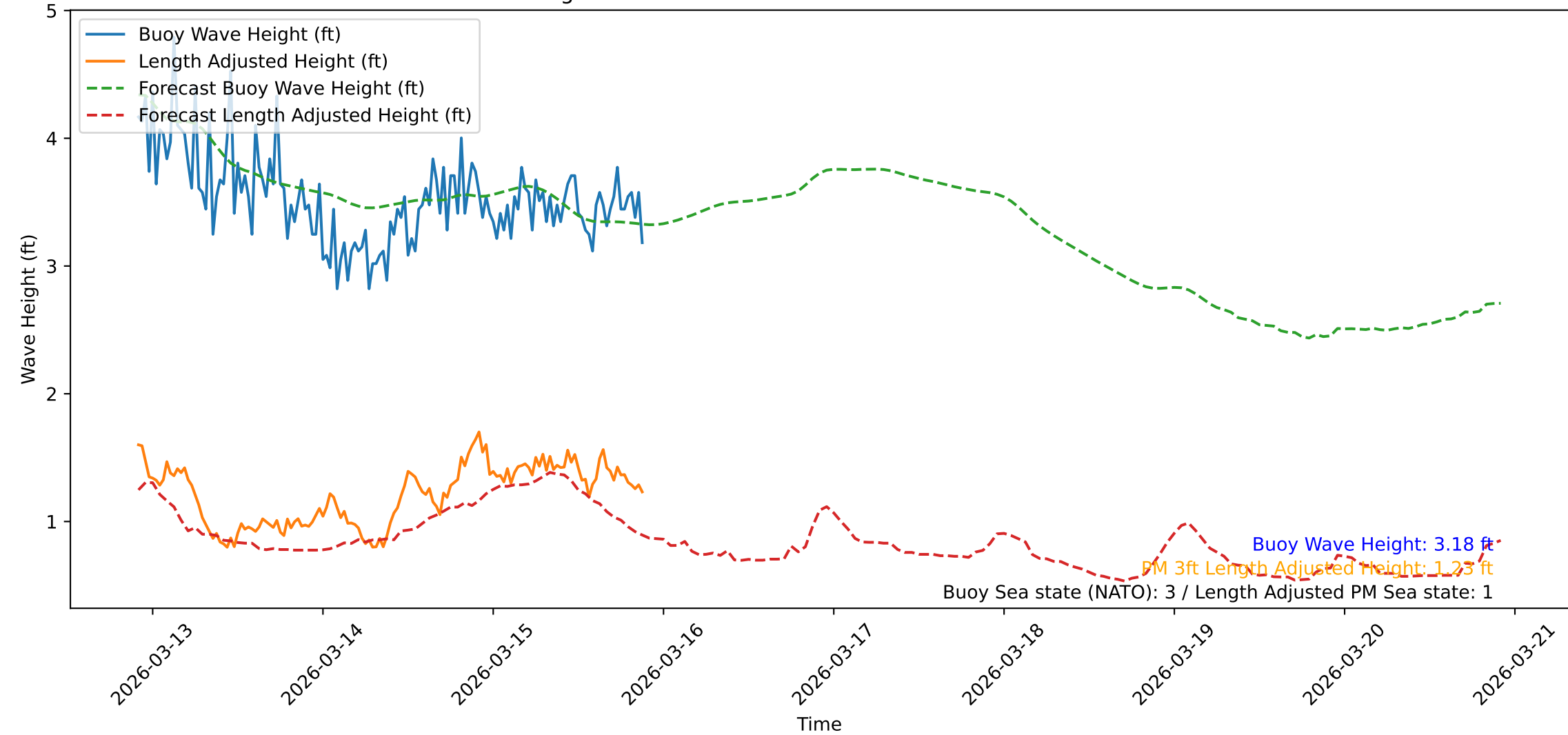
Wave Heights over Time for Green Beach at 2026-03-15 22:01:44
