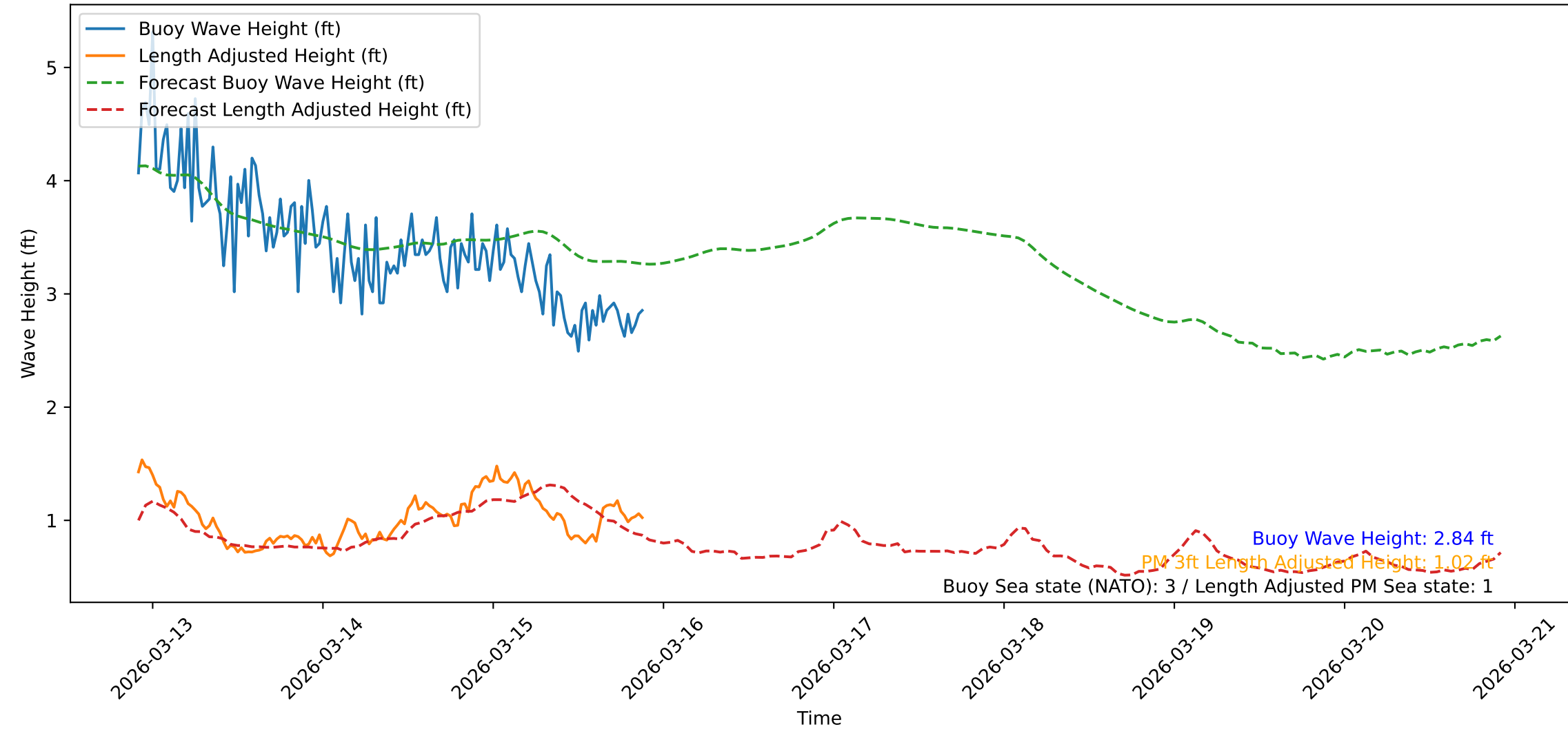
Wave Heights over Time for Oceanside Harbor at 2026-03-15 22:00:43
