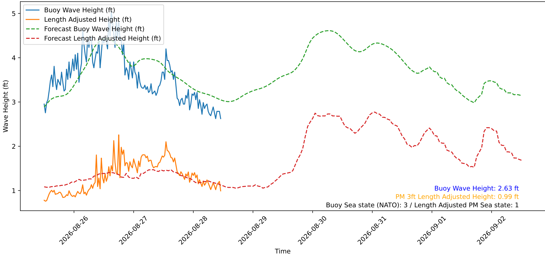
Wave Heights over Time for Red Beach at 2026-08-28 11:50:50
