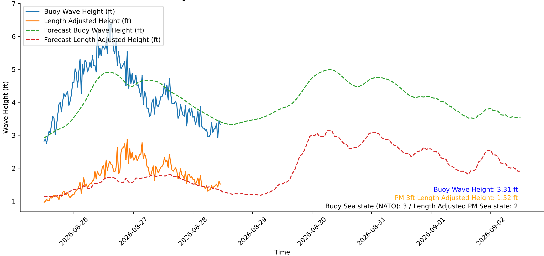
Wave Heights over Time for Oceanside Harbor at 2026-08-28 11:50:29
