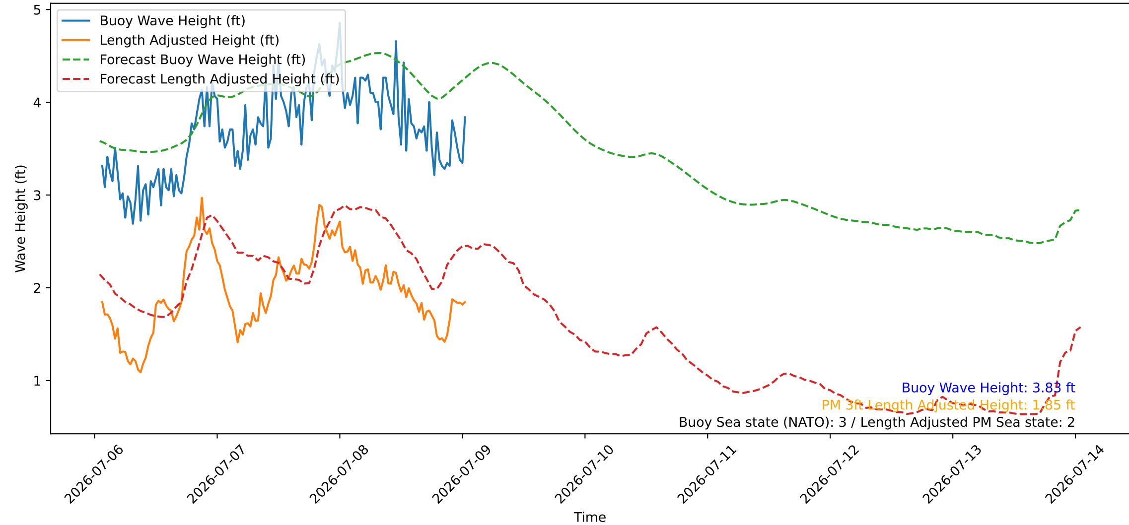
Wave Heights over Time for Red Beach at 2026-07-09 01:10:46
