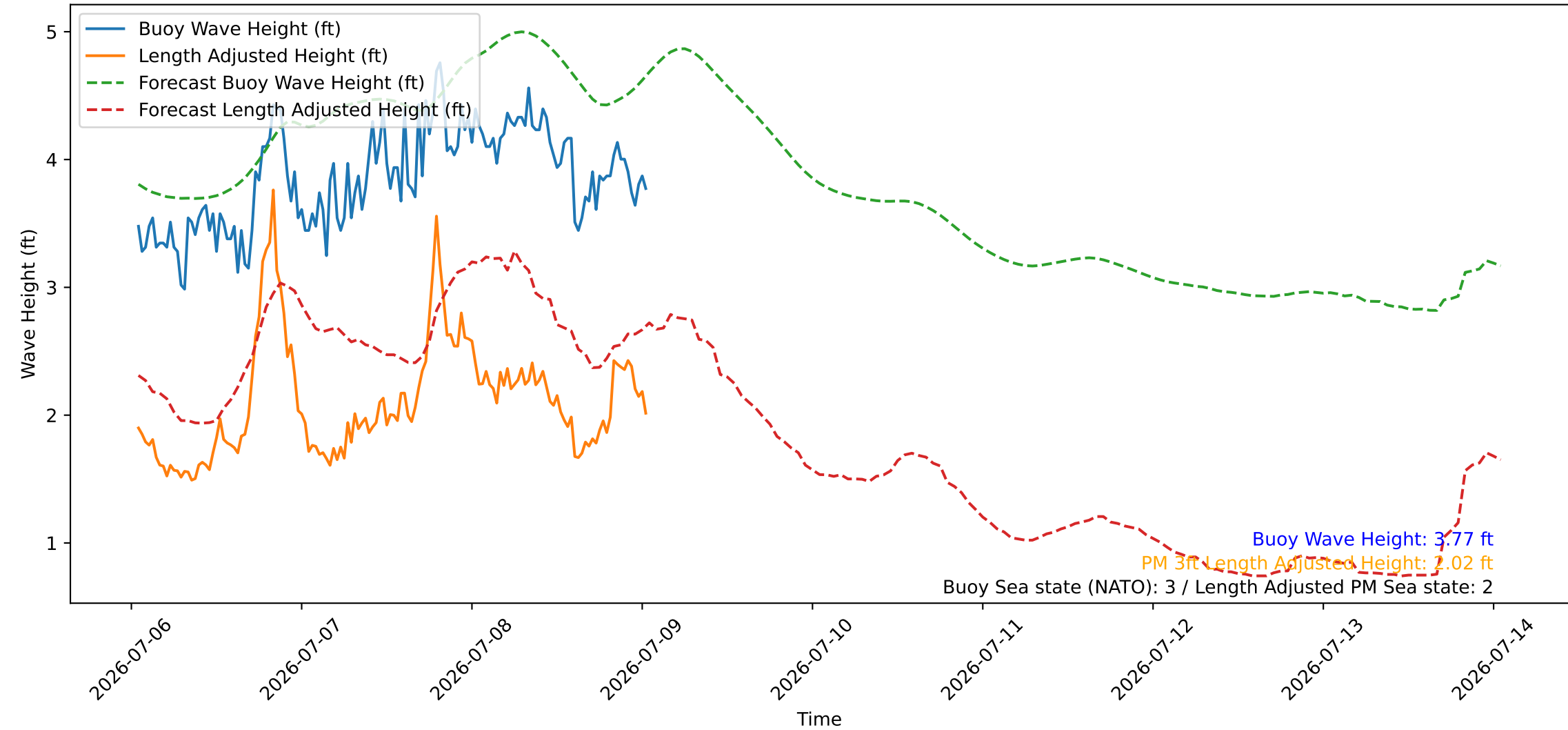
Wave Heights over Time for Green Beach at 2026-07-09 01:11:08
