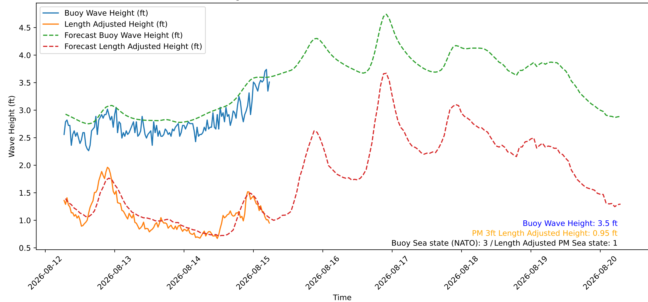
Wave Heights over Time for Green Beach at 2026-08-15 06:31:10
