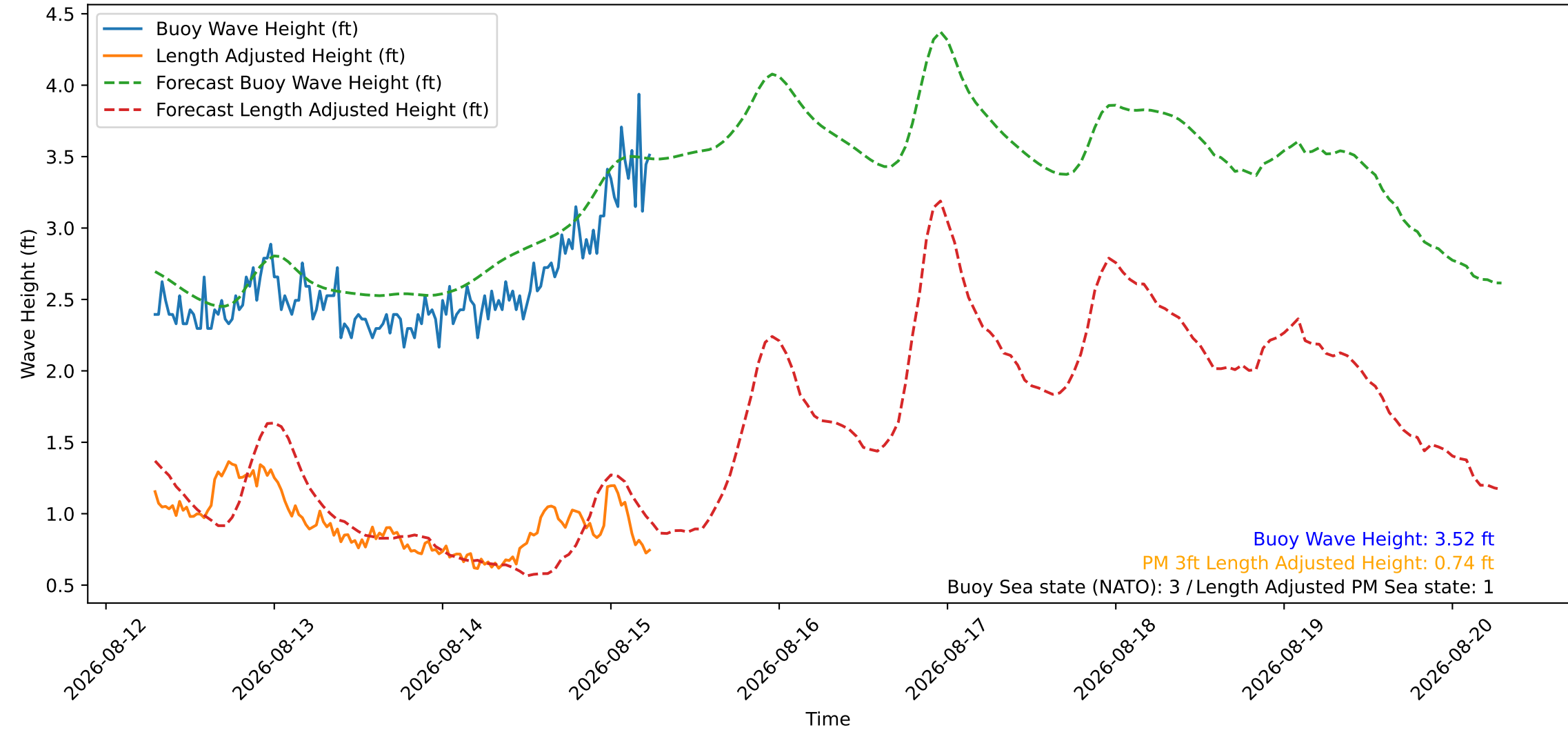
Wave Heights over Time for Red Beach at 2026-08-15 06:30:47
