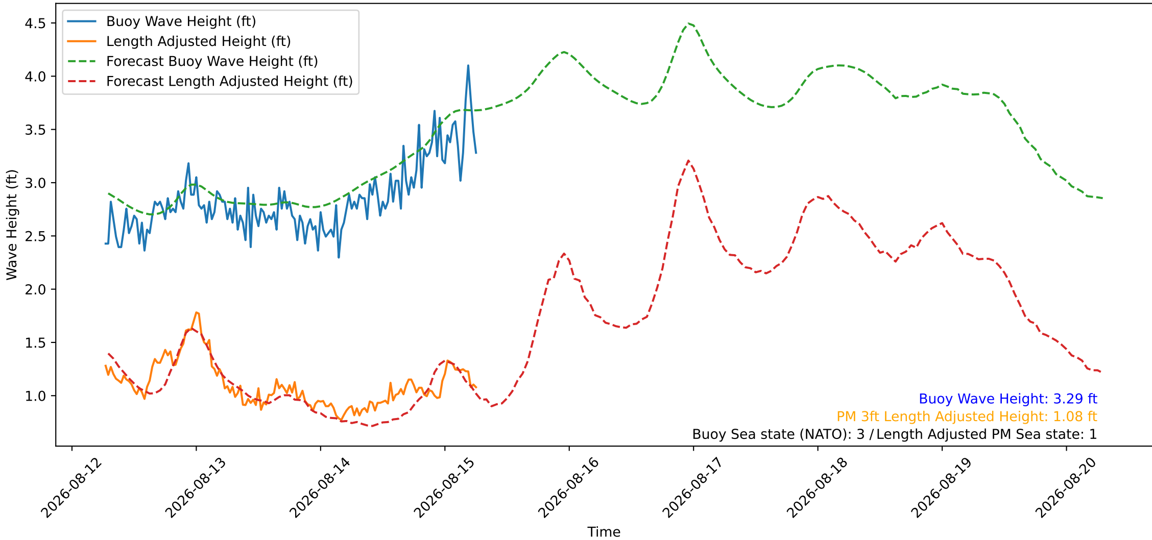
Wave Heights over Time for Oceanside Harbor at 2026-08-15 06:30:27
