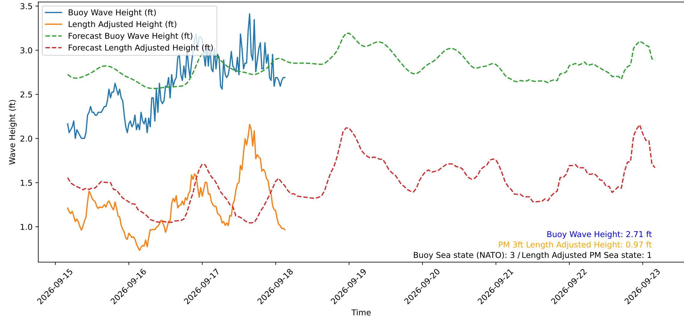
Wave Heights over Time for Red Beach at 2026-09-18 03:50:50
