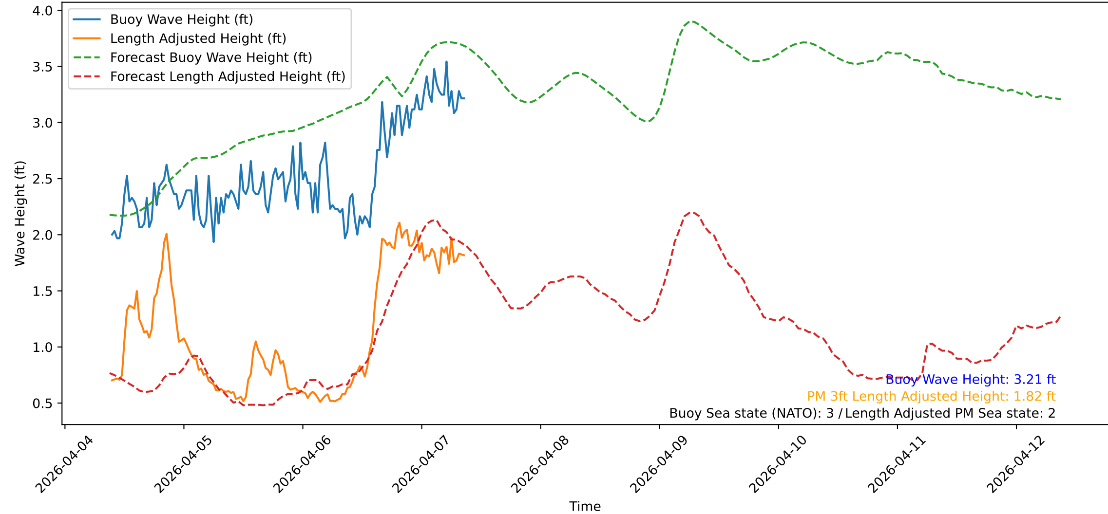
Wave Heights over Time for Red Beach at 2026-04-07 09:20:46
