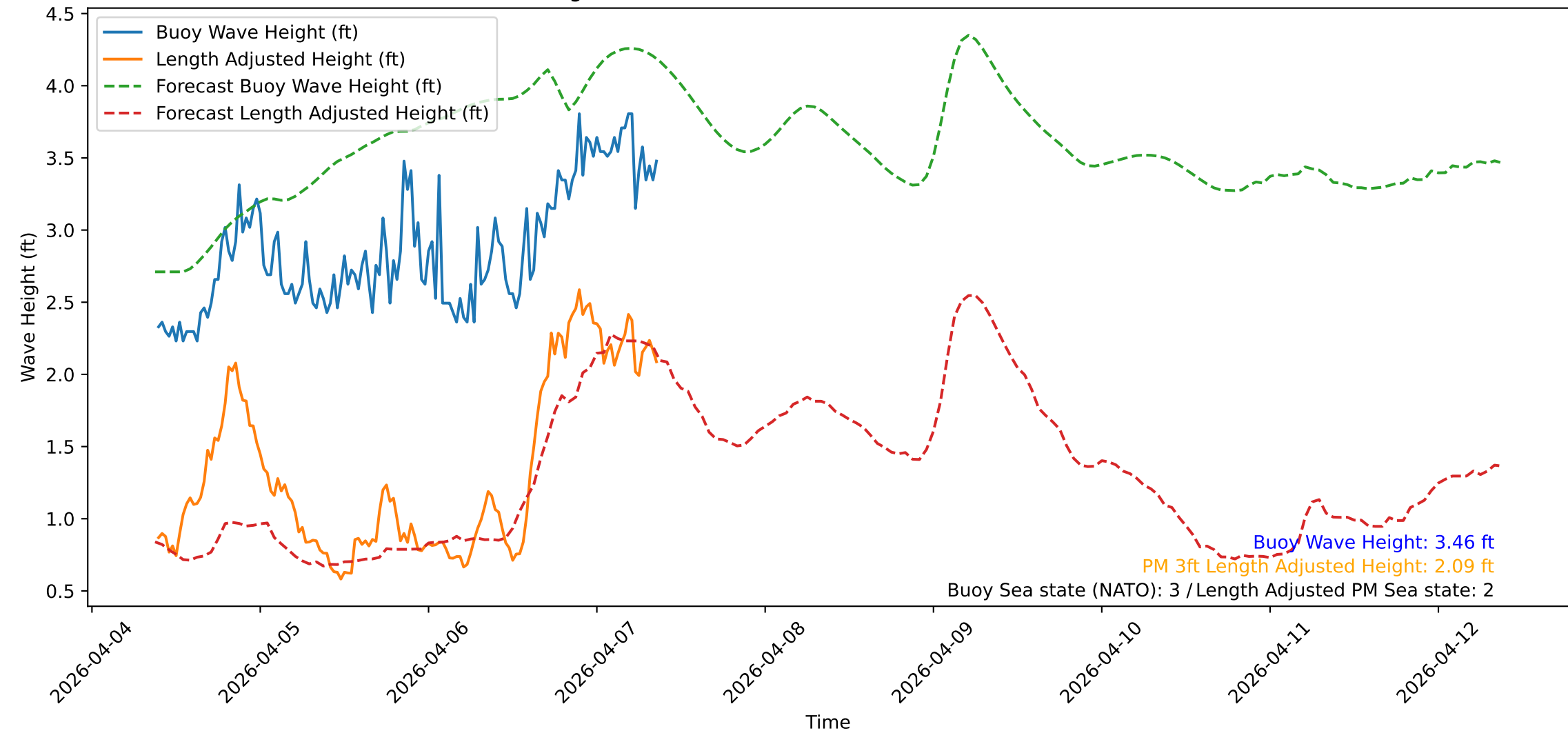
Wave Heights over Time for Green Beach at 2026-04-07 09:21:09
