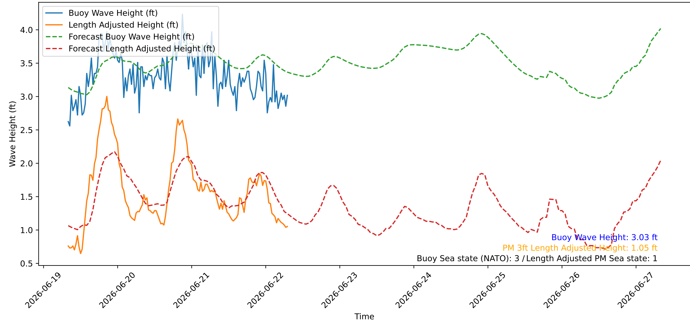
Wave Heights over Time for Green Beach at 2026-06-22 07:51:09
