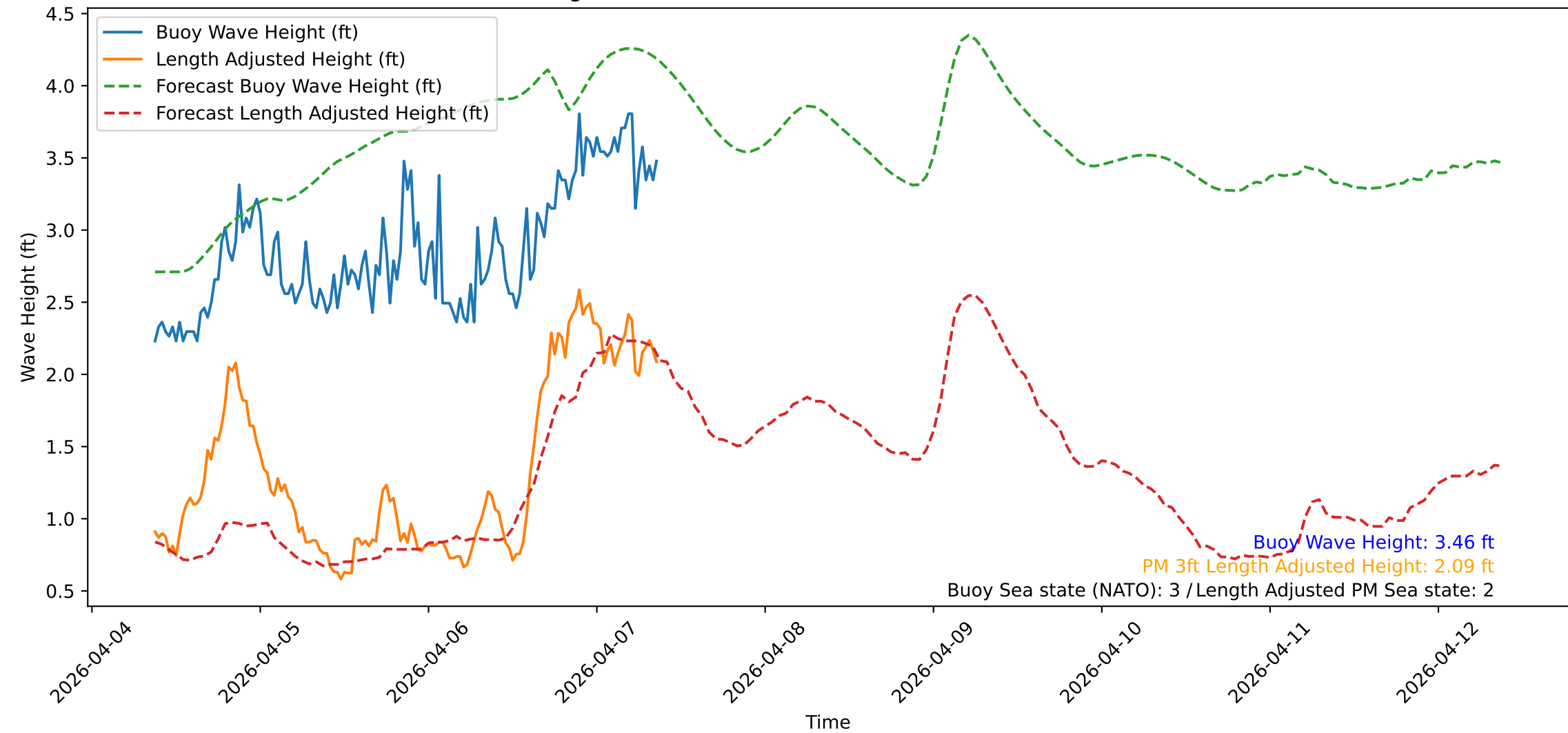
Wave Heights over Time for Green Beach at 2026-04-07 09:11:11
