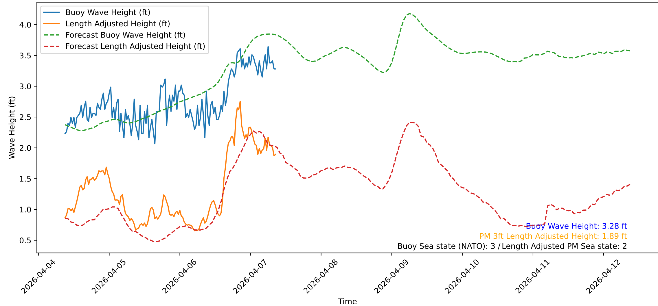
Wave Heights over Time for Oceanside Harbor at 2026-04-07 09:10:32
