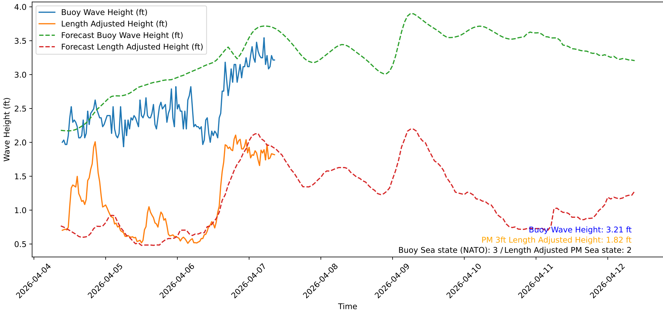
Wave Heights over Time for Red Beach at 2026-04-07 09:10:49
