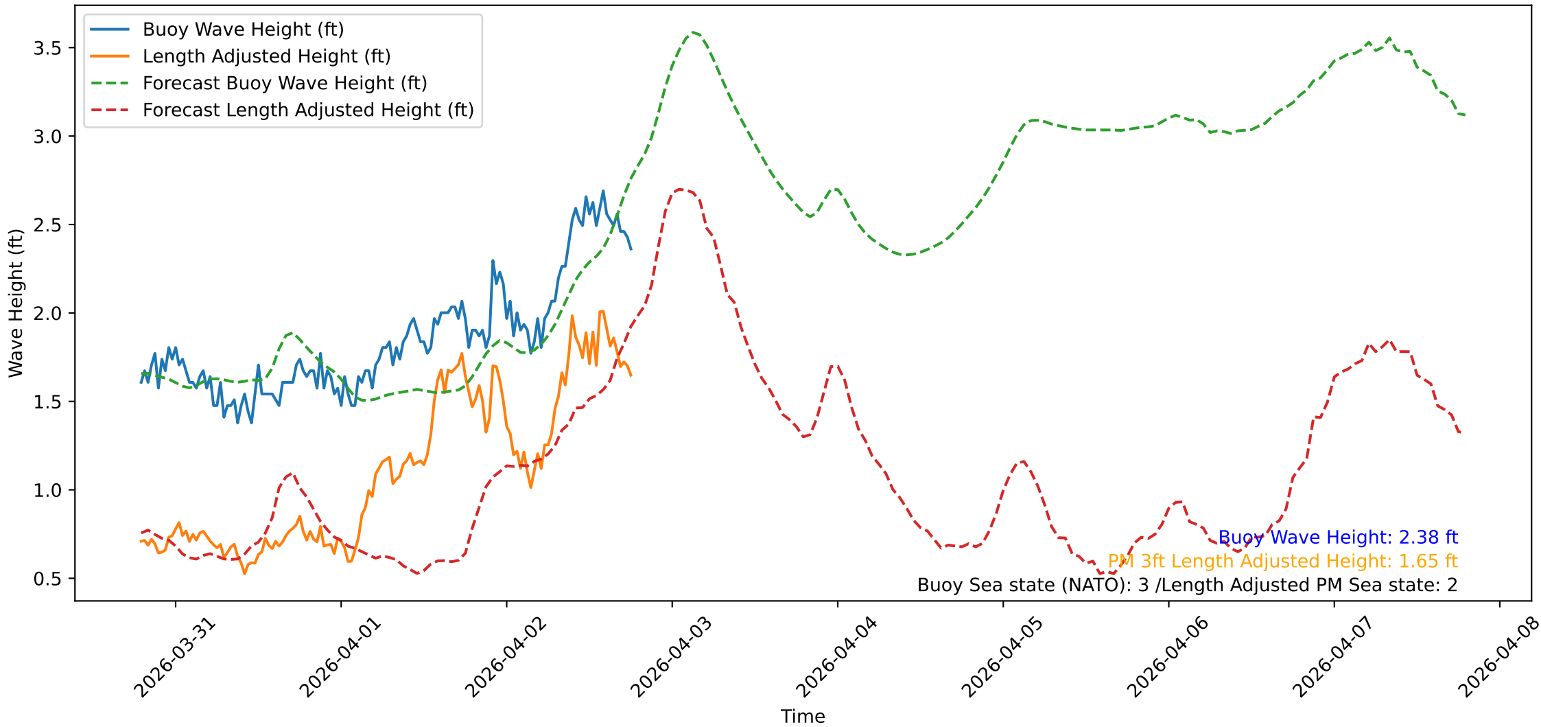
Wave Heights over Time for Red Beach at 2026-04-02 18:50:48
