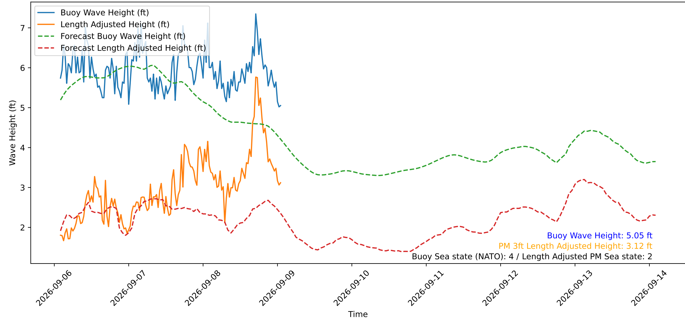
Wave Heights over Time for Oceanside Harbor at 2026-09-09 01:50:30
