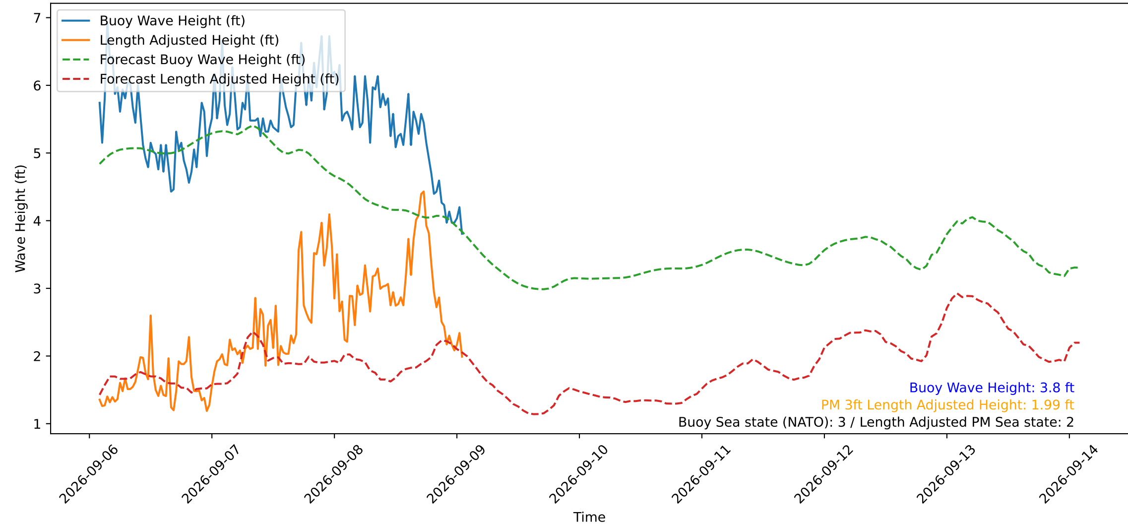
Wave Heights over Time for Red Beach at 2026-09-09 01:50:50
