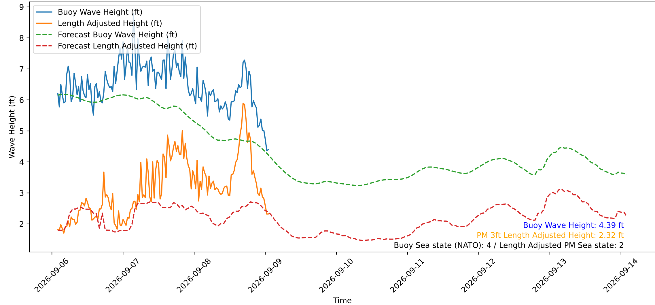
Wave Heights over Time for Green Beach at 2026-09-09 01:51:14
