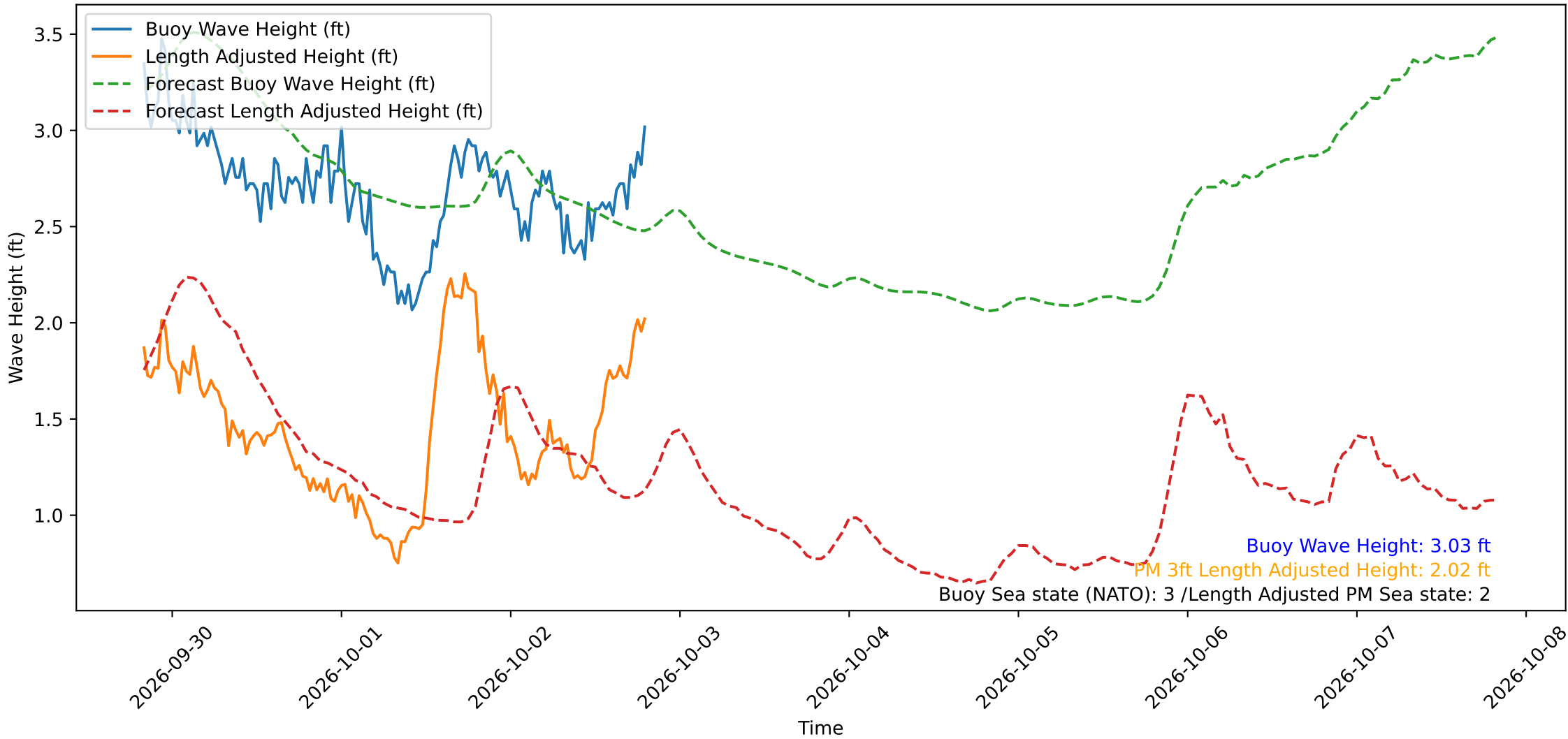
Wave Heights over Time for Red Beach at 2026-10-02 19:40:49
