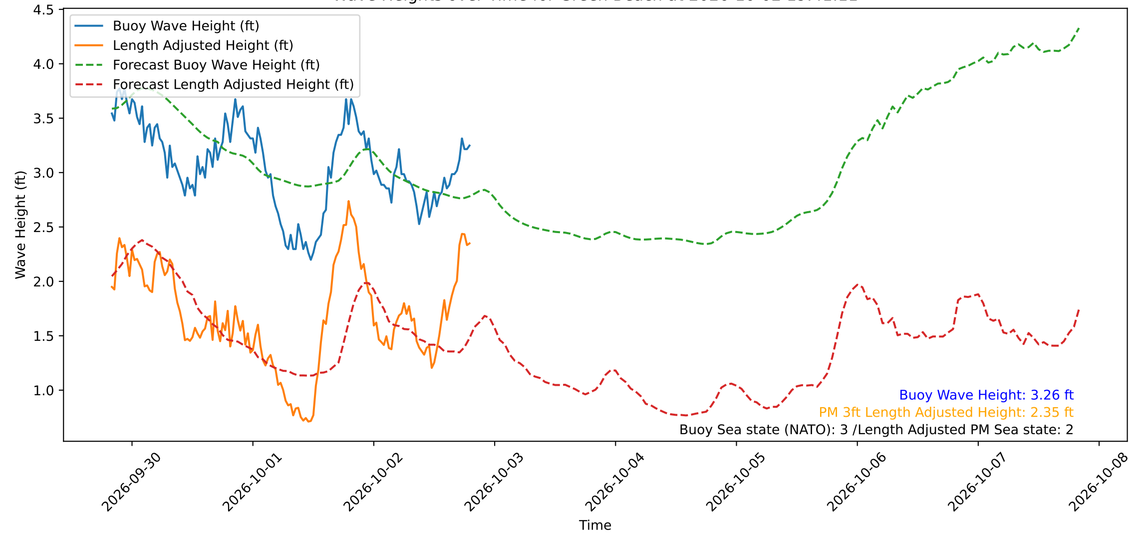
Wave Heights over Time for Green Beach at 2026-10-02 19:41:11
