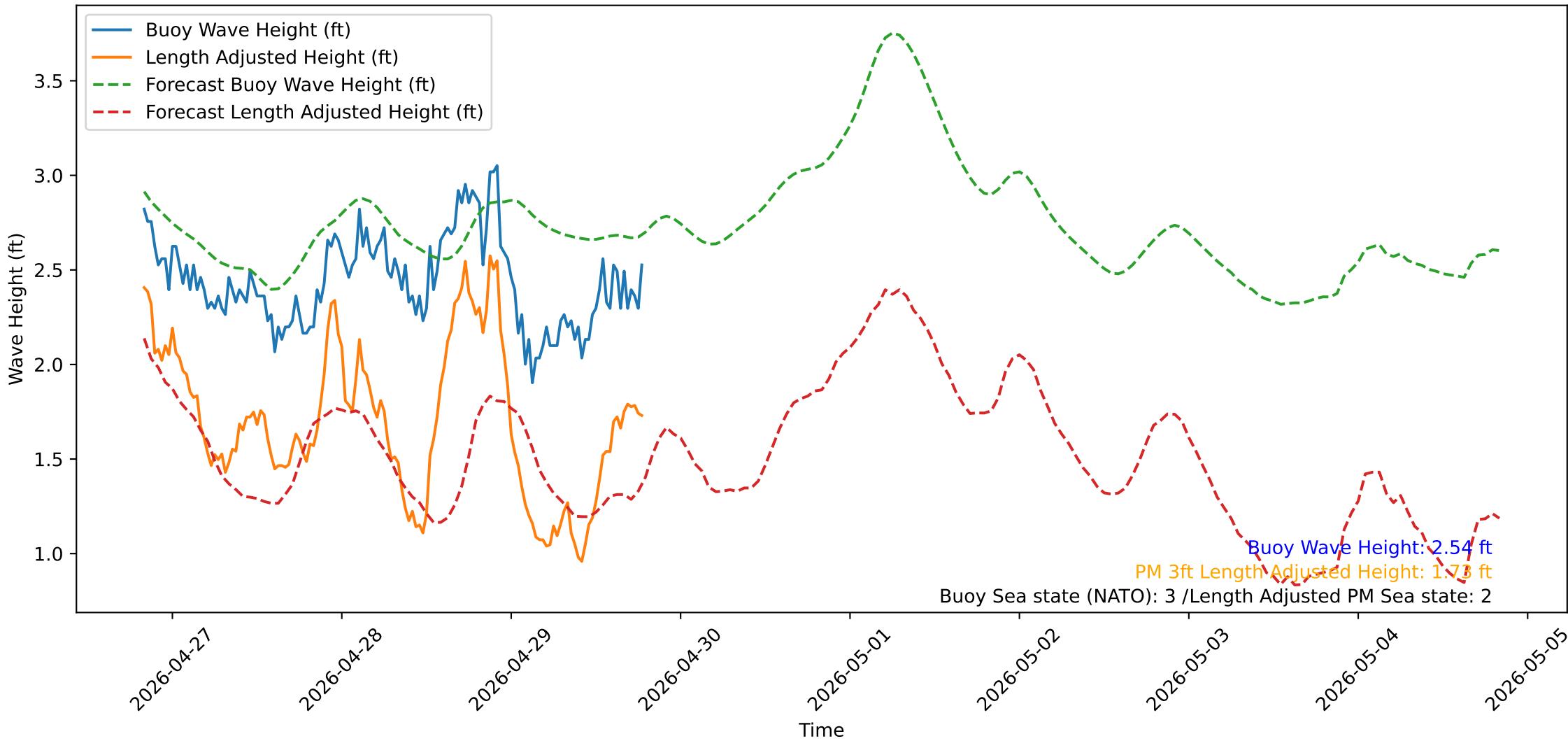
Wave Heights over Time for Oceanside Harbor at 2026-04-29 20:00:31
