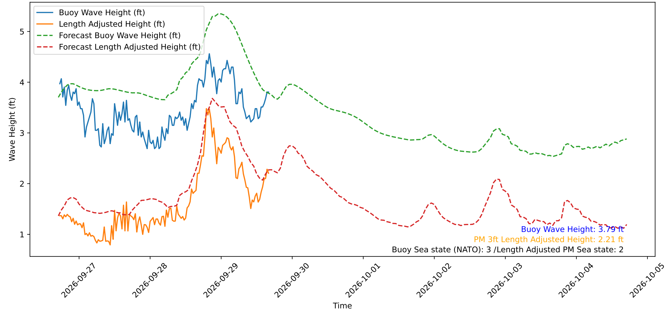
Wave Heights over Time for Green Beach at 2026-09-29 17:01:14
