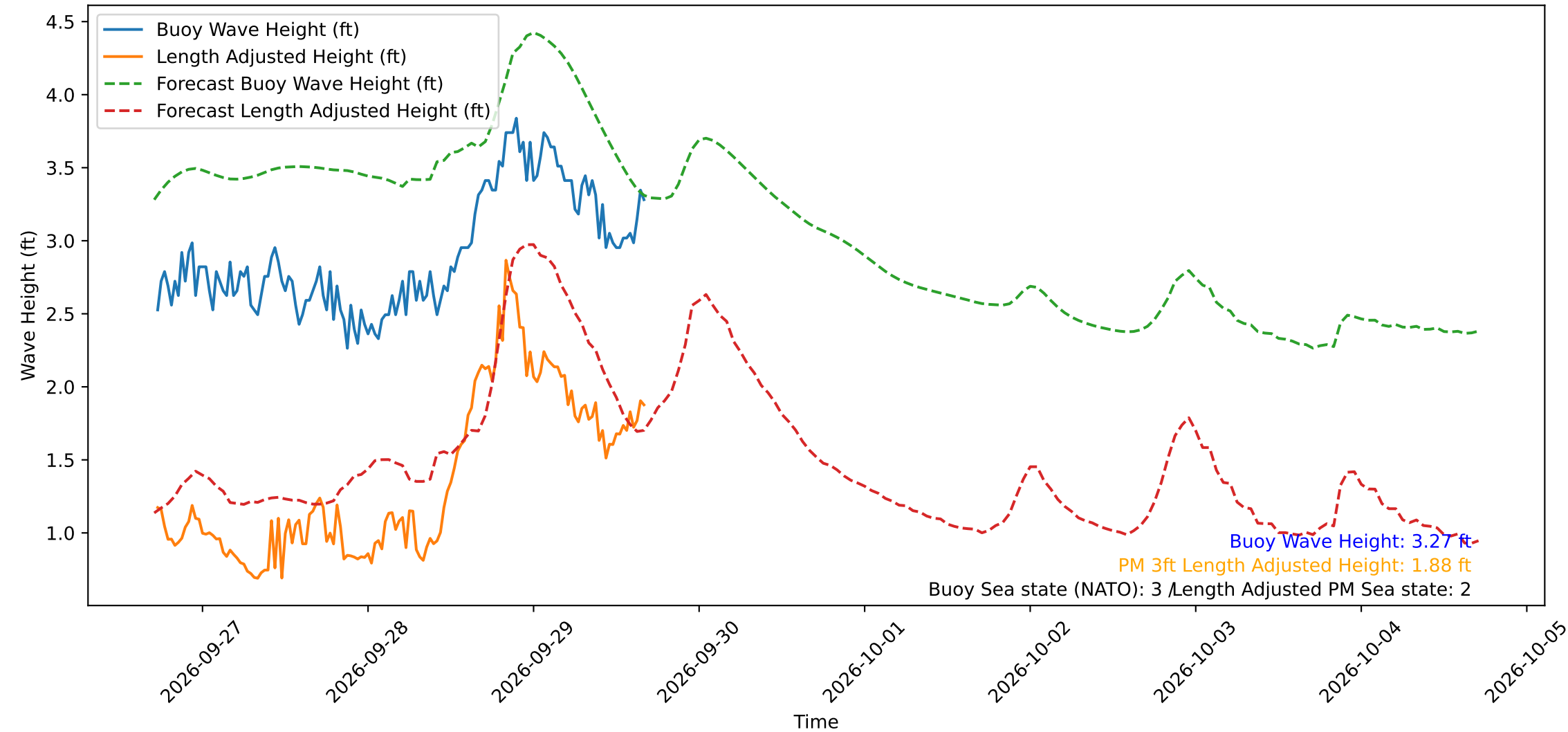
Wave Heights over Time for Red Beach at 2026-09-29 17:00:51
