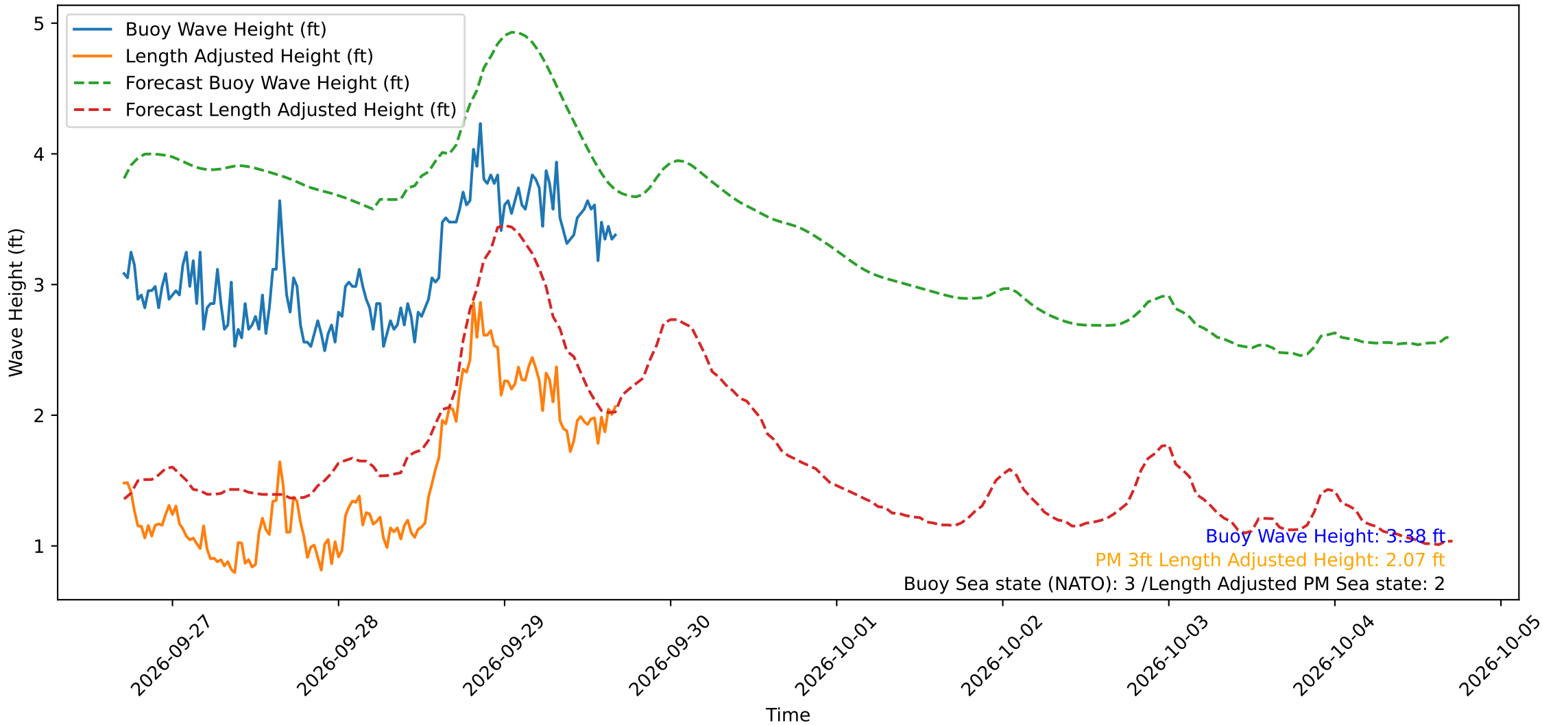
Wave Heights over Time for Oceanside Harbor at 2026-09-29 17:00:31
