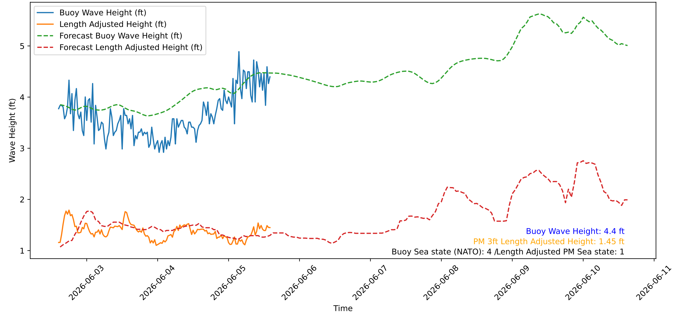
Wave Heights over Time for Oceanside Harbor at 2026-06-05 14:30:26
