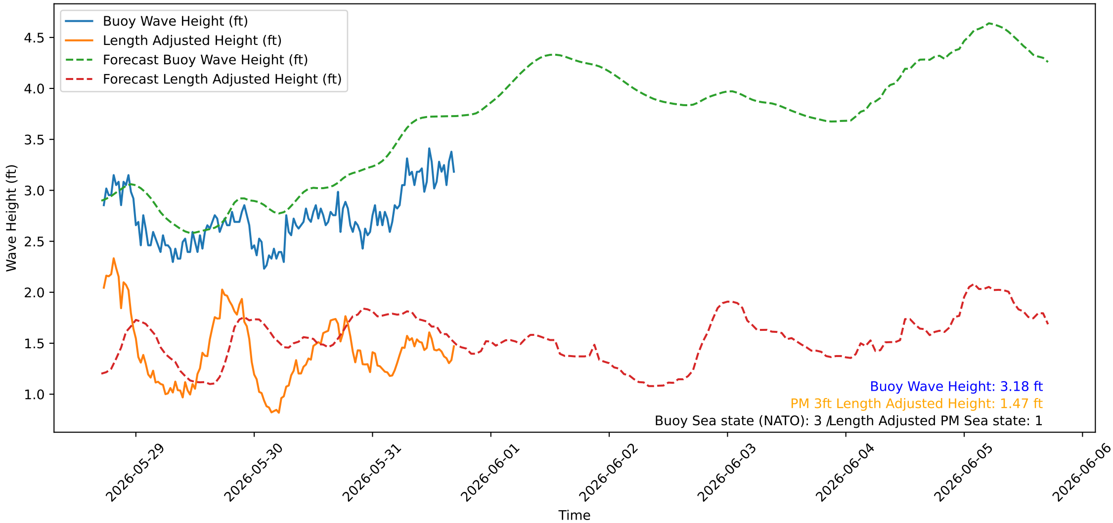
Wave Heights over Time for Red Beach at 2026-05-31 17:10:44
