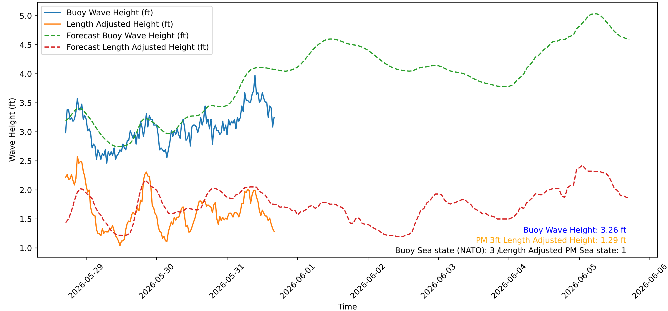
Wave Heights over Time for Green Beach at 2026-05-31 17:11:07
