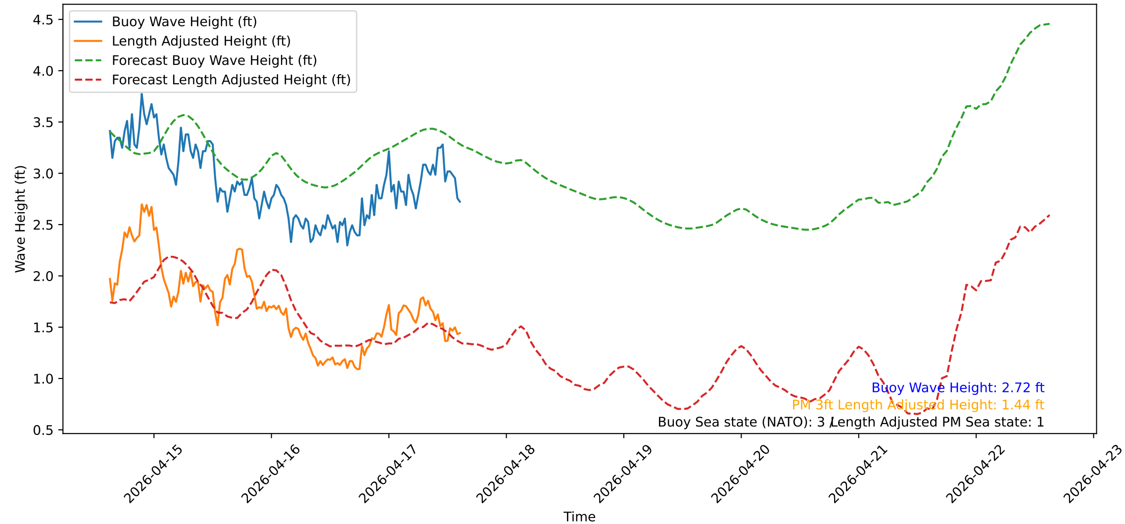
Wave Heights over Time for Oceanside Harbor at 2026-04-17 15:10:34
