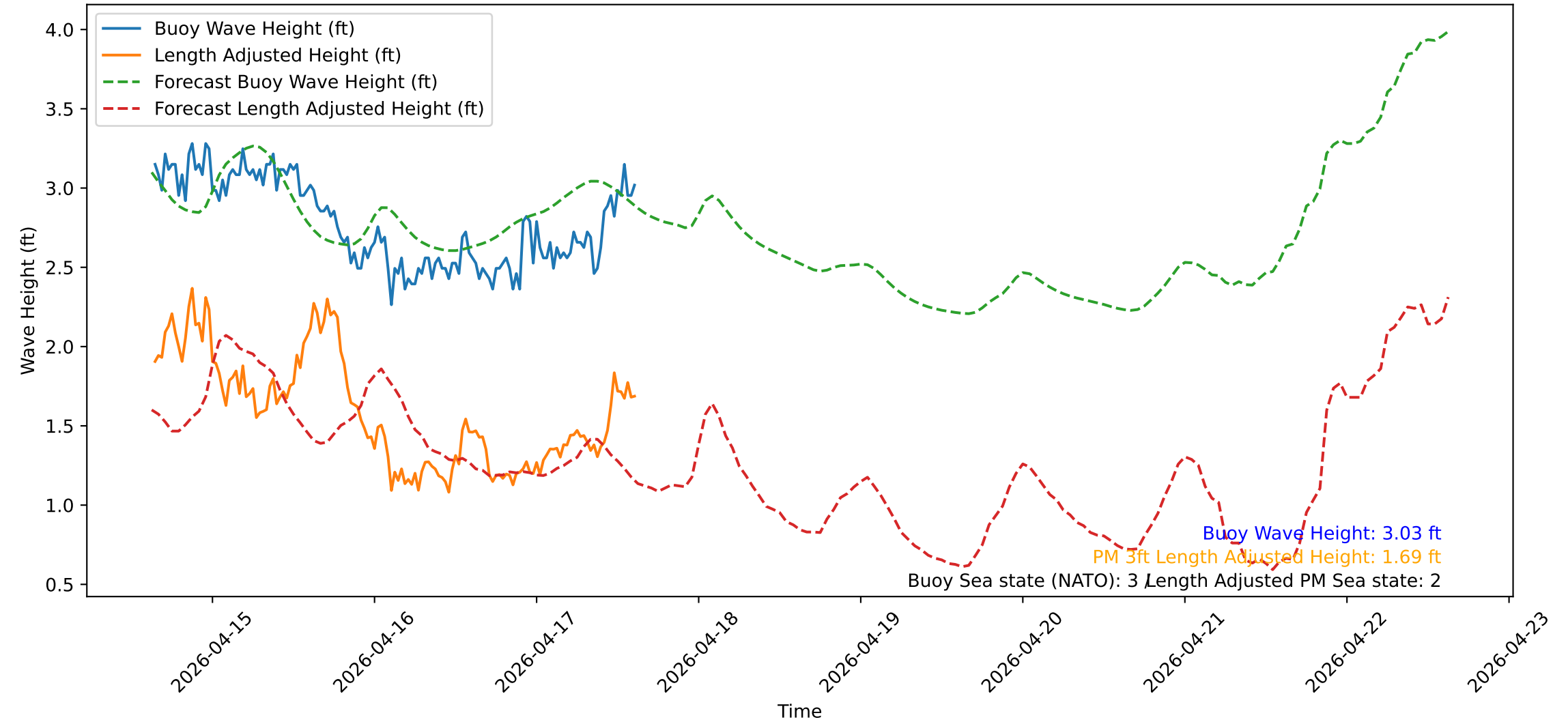
Wave Heights over Time for Red Beach at 2026-04-17 15:10:55
