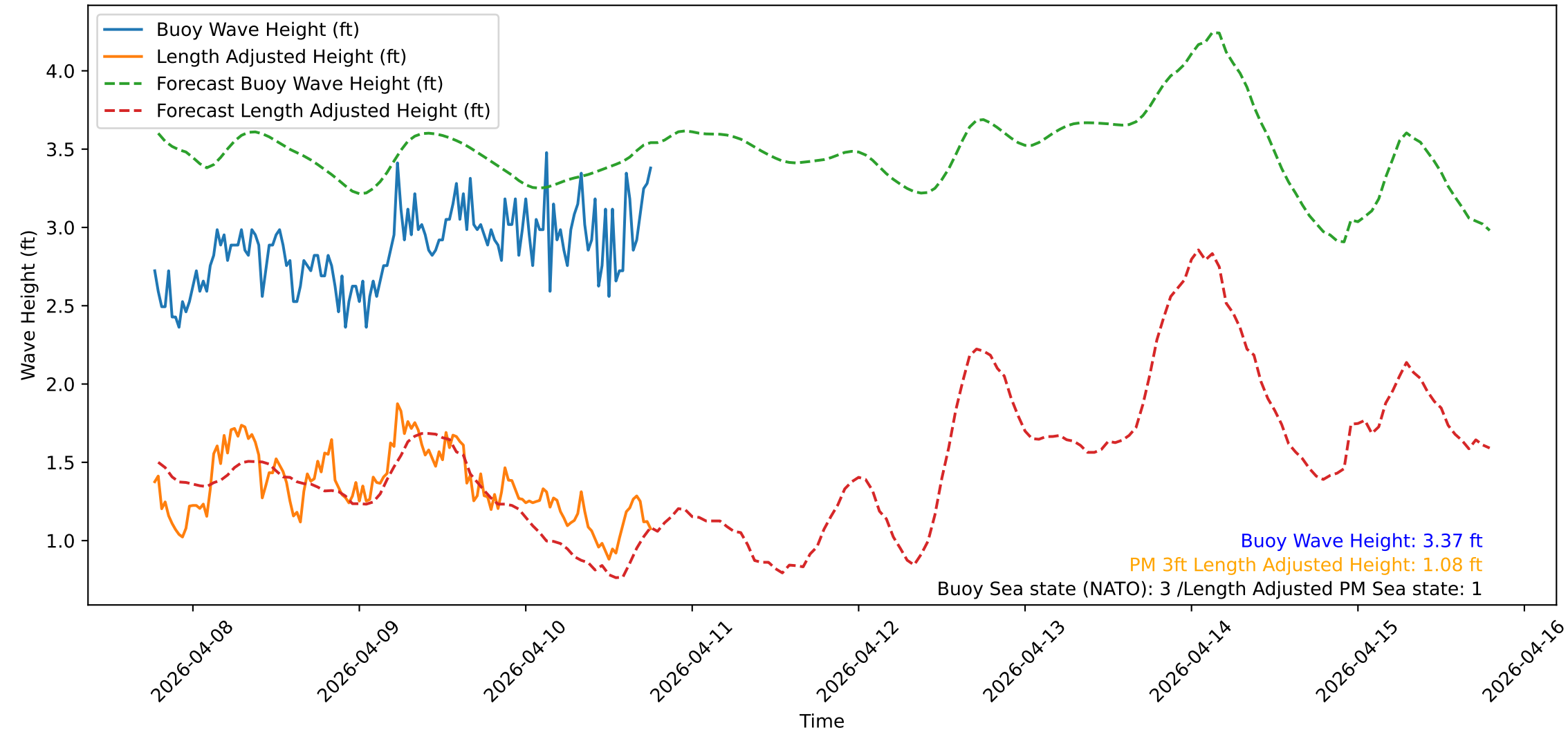
Wave Heights over Time for Green Beach at 2026-04-10 18:41:13
