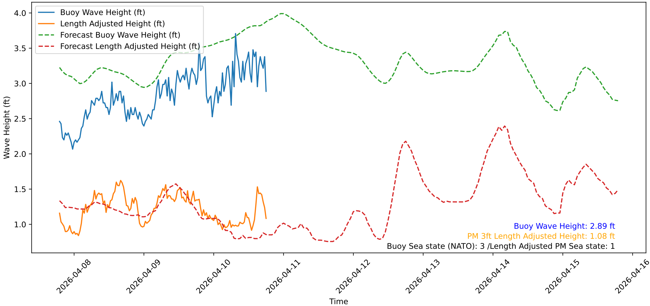
Wave Heights over Time for Red Beach at 2026-04-10 18:40:50
