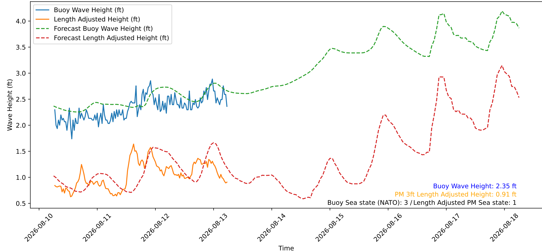
Wave Heights over Time for Red Beach at 2026-08-13 06:20:47
