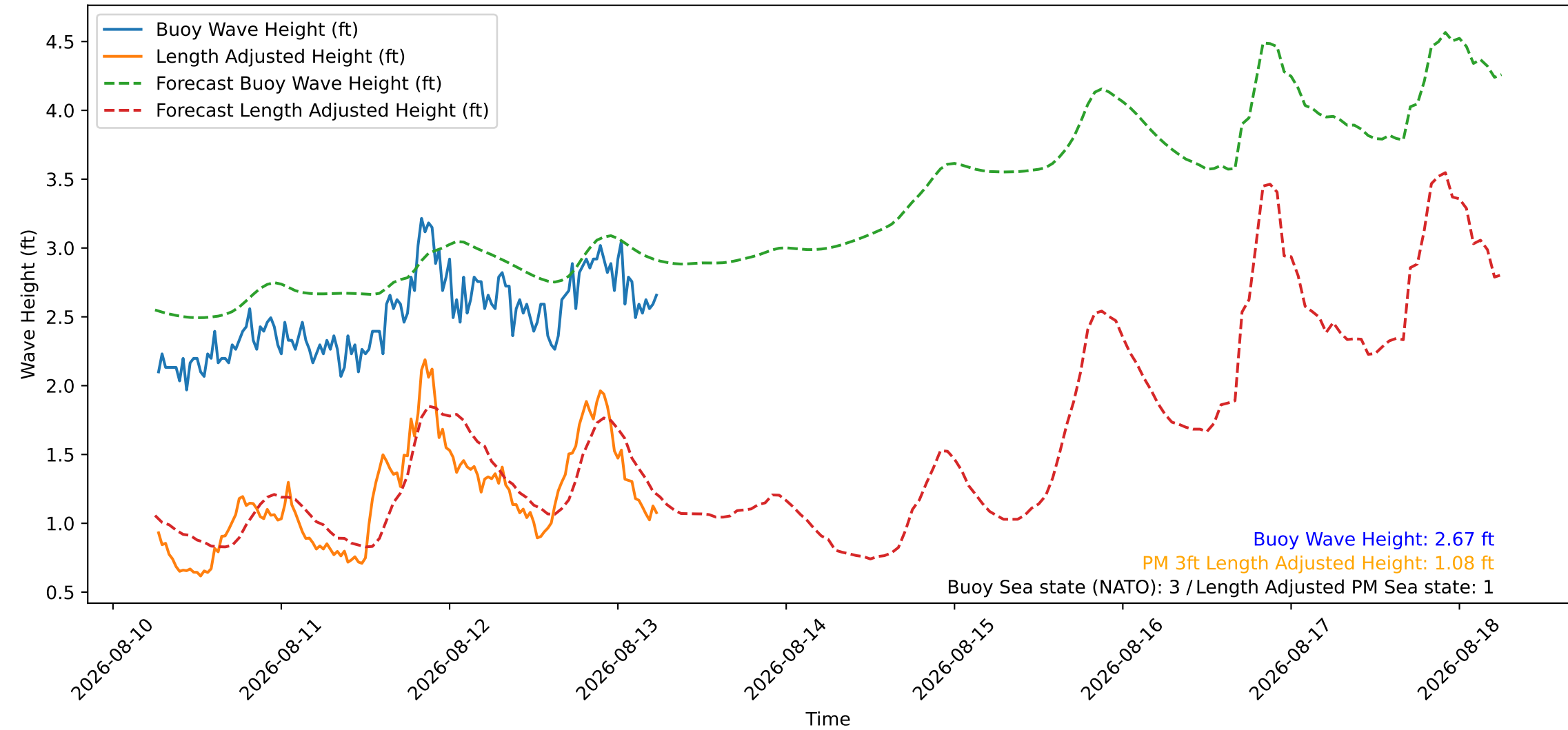
Wave Heights over Time for Green Beach at 2026-08-13 06:21:09
