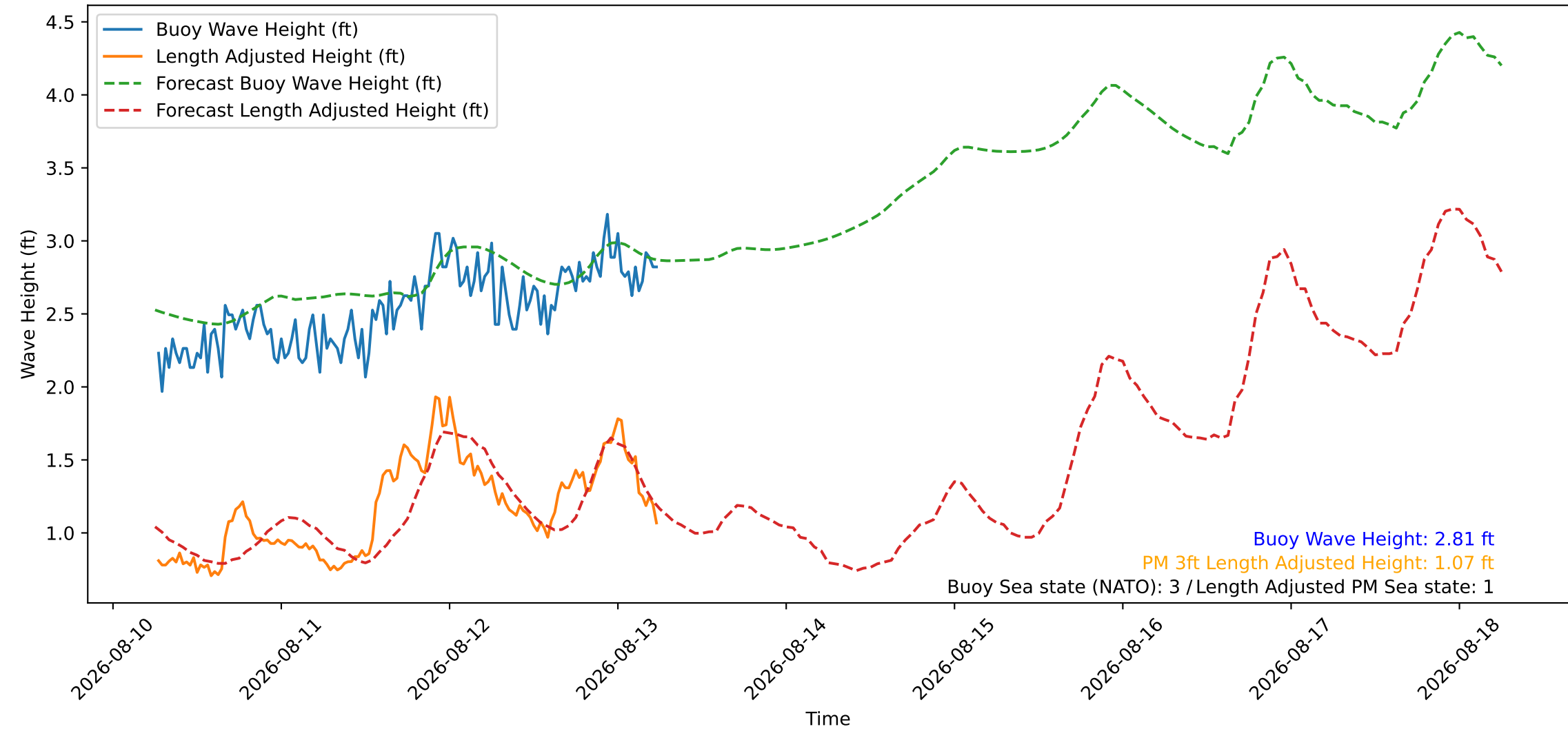
Wave Heights over Time for Oceanside Harbor at 2026-08-13 06:20:27
