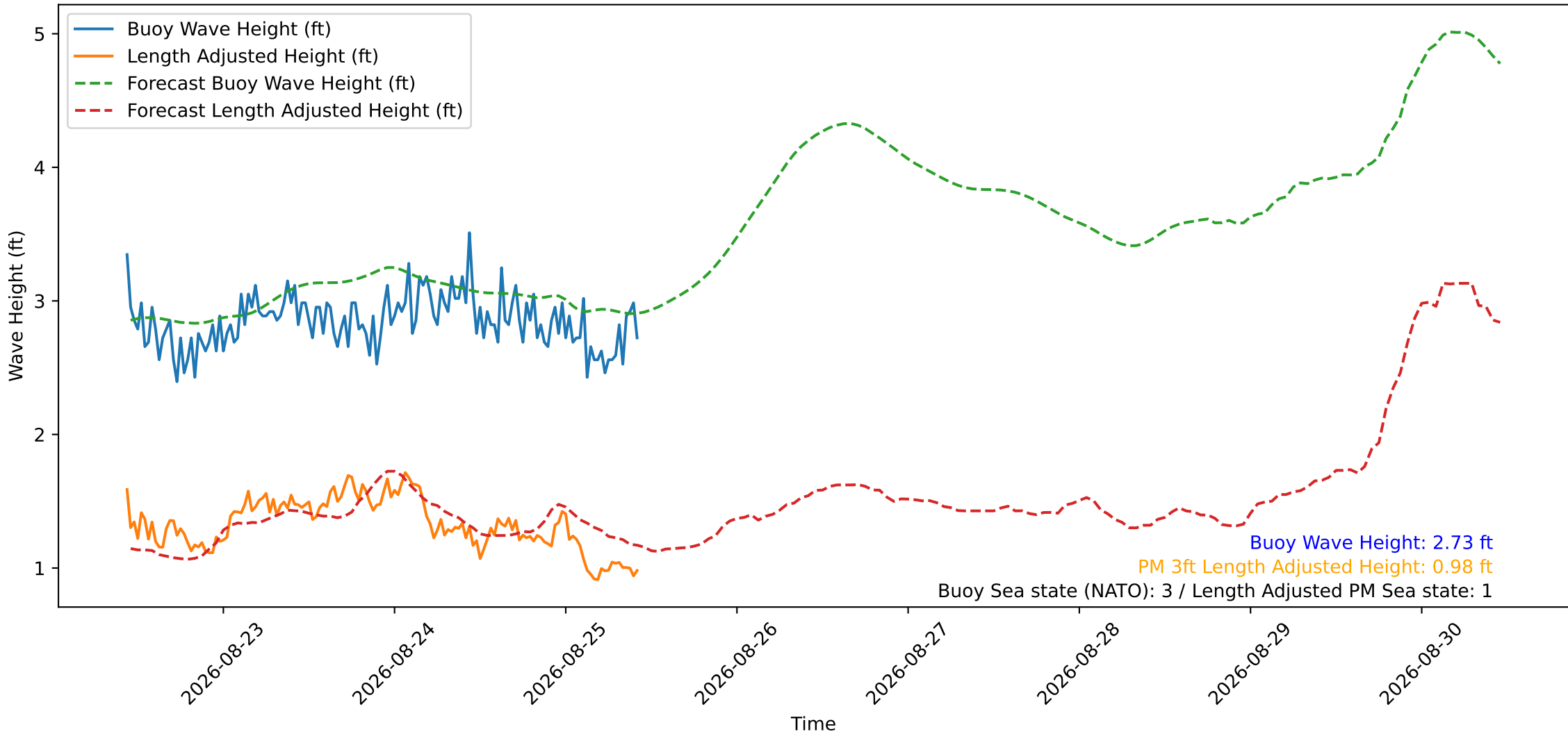
Wave Heights over Time for Oceanside Harbor at 2026-08-25 10:30:29
