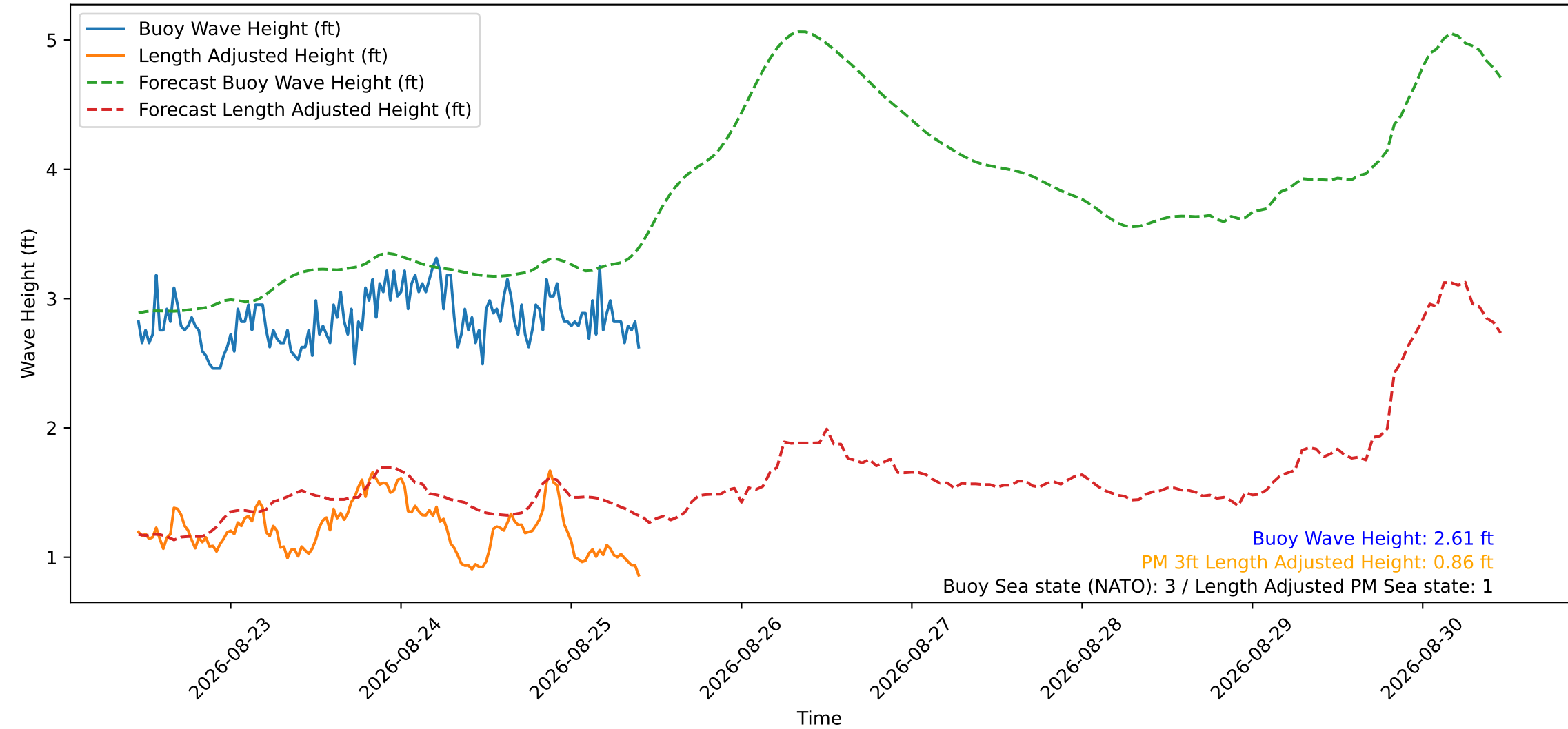
Wave Heights over Time for Green Beach at 2026-08-25 10:31:11
