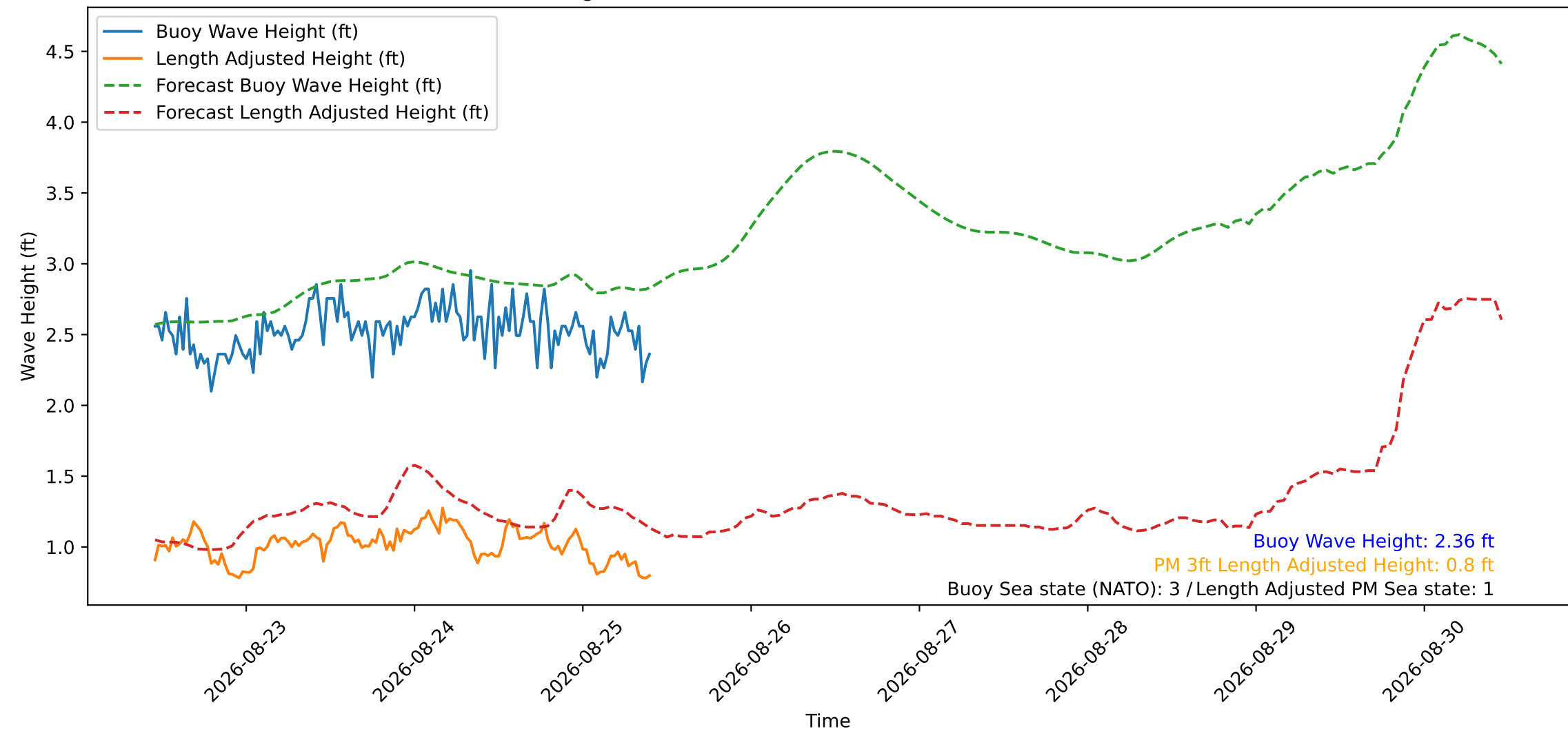
Wave Heights over Time for Red Beach at 2026-08-25 10:30:48
