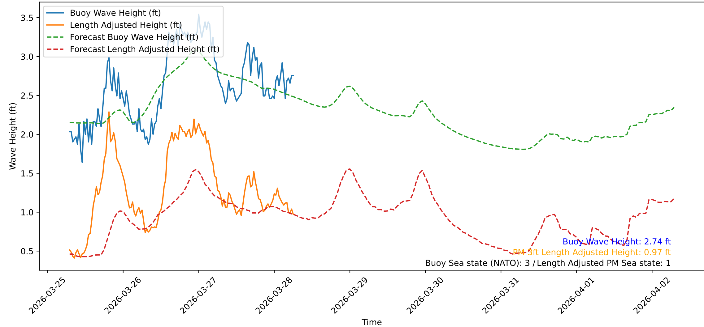
Wave Heights over Time for Green Beach at 2026-03-28 06:51:09
