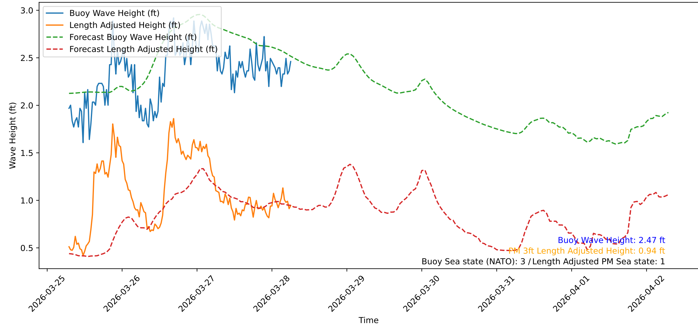
Wave Heights over Time for Oceanside Harbor at 2026-03-28 06:50:31
