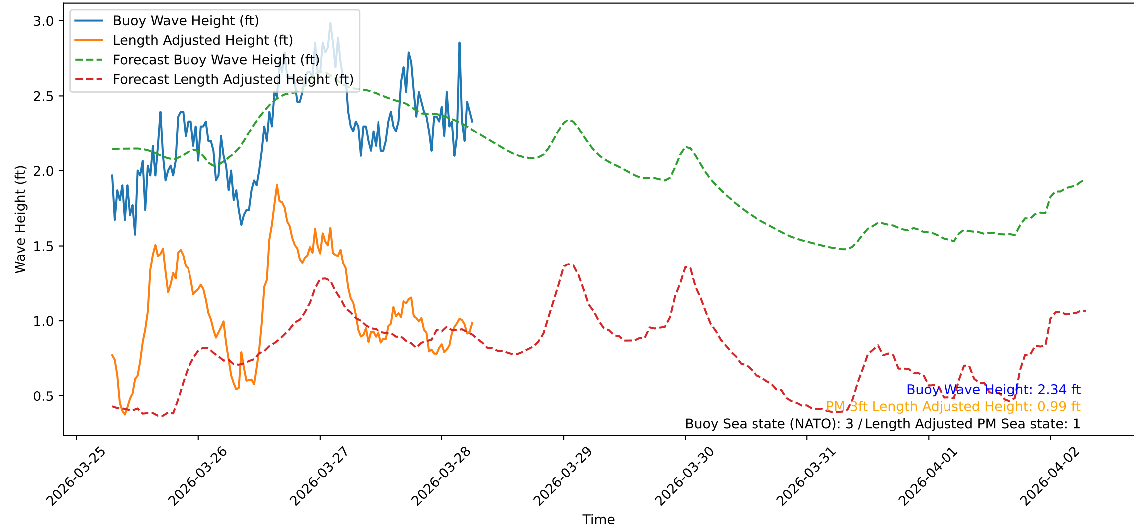
Wave Heights over Time for Red Beach at 2026-03-28 06:50:47
