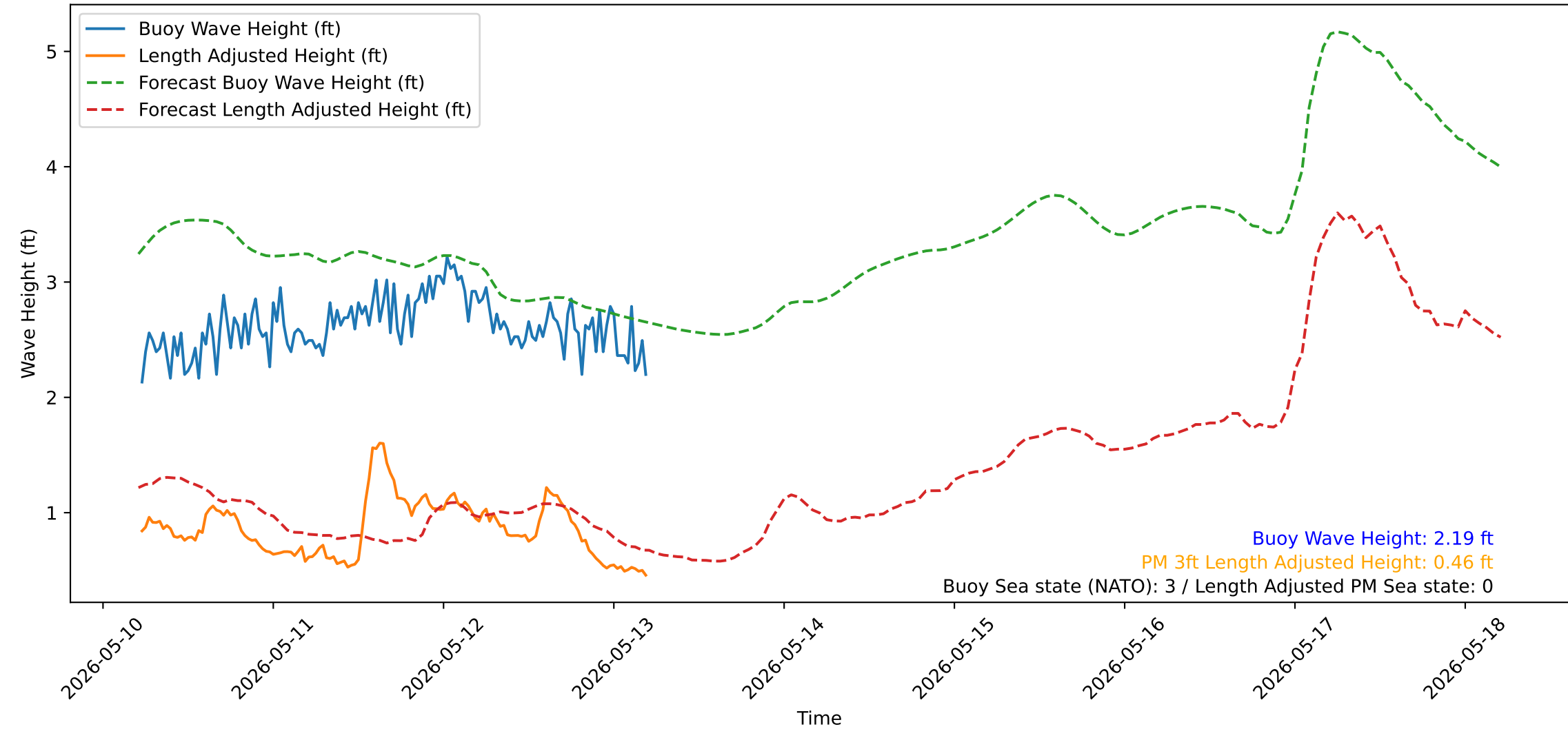
Wave Heights over Time for Red Beach at 2026-05-13 05:10:51
