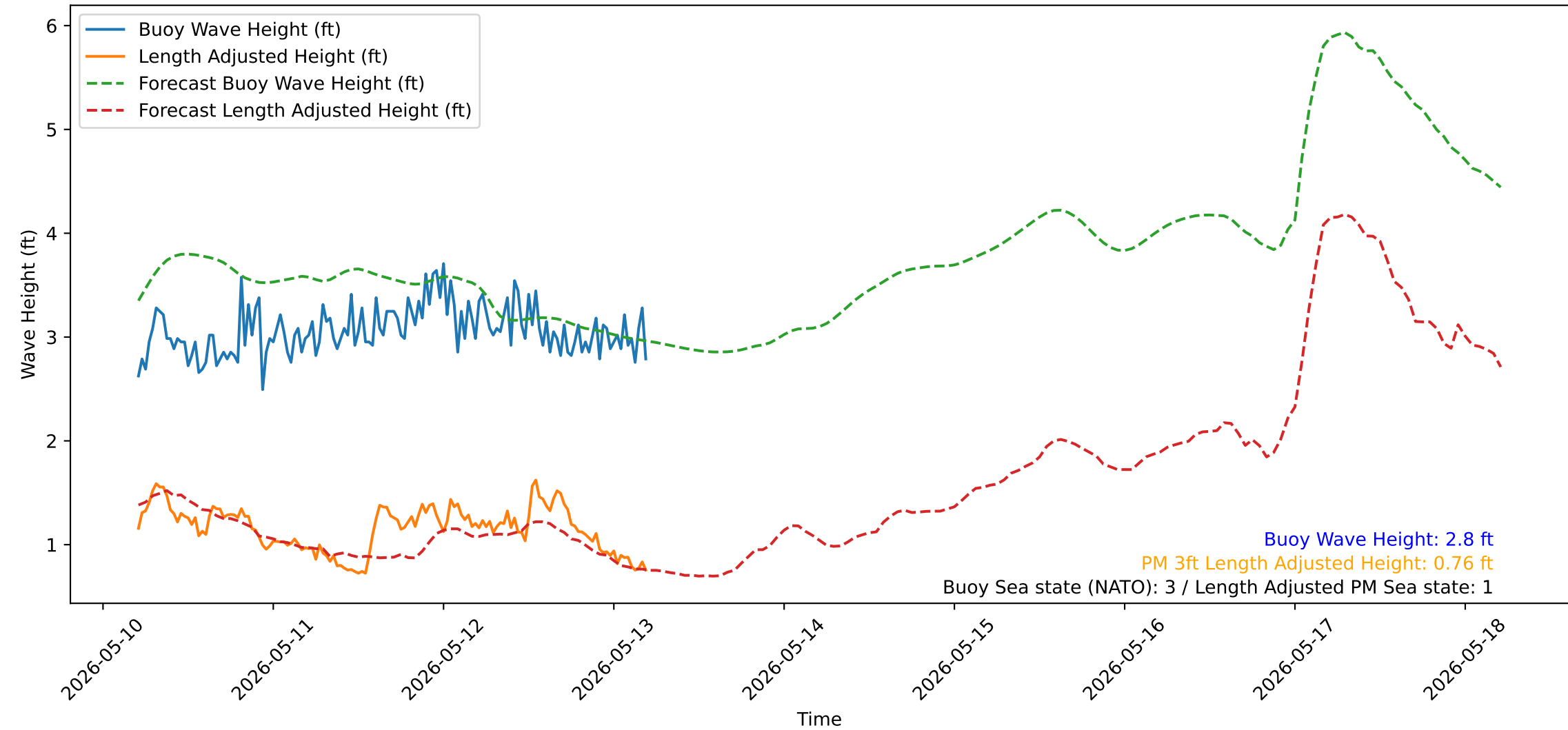
Wave Heights over Time for Oceanside Harbor at 2026-05-13 05:10:31
