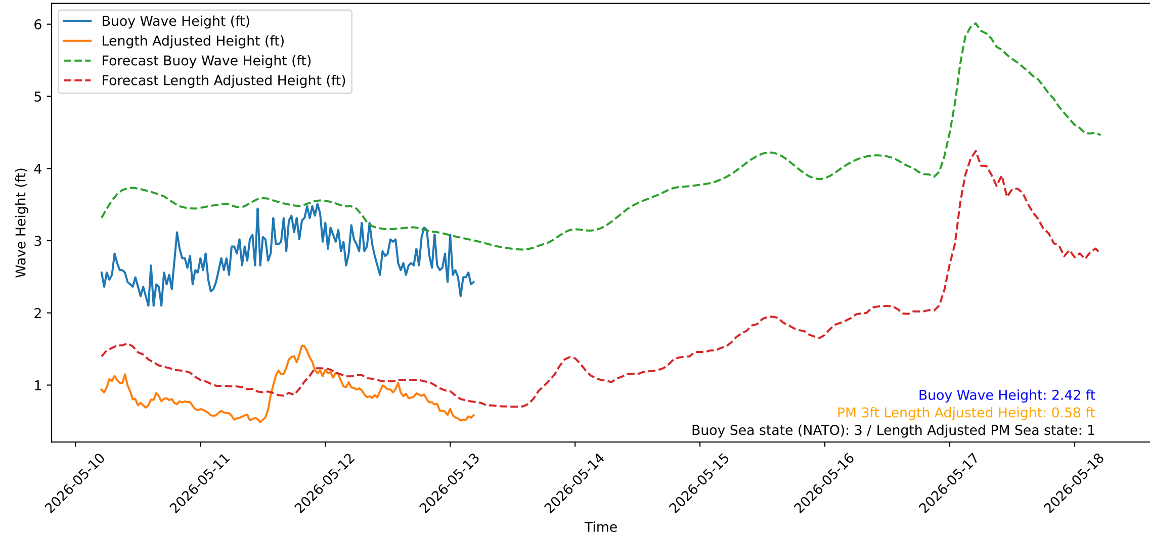
Wave Heights over Time for Green Beach at 2026-05-13 05:11:13
