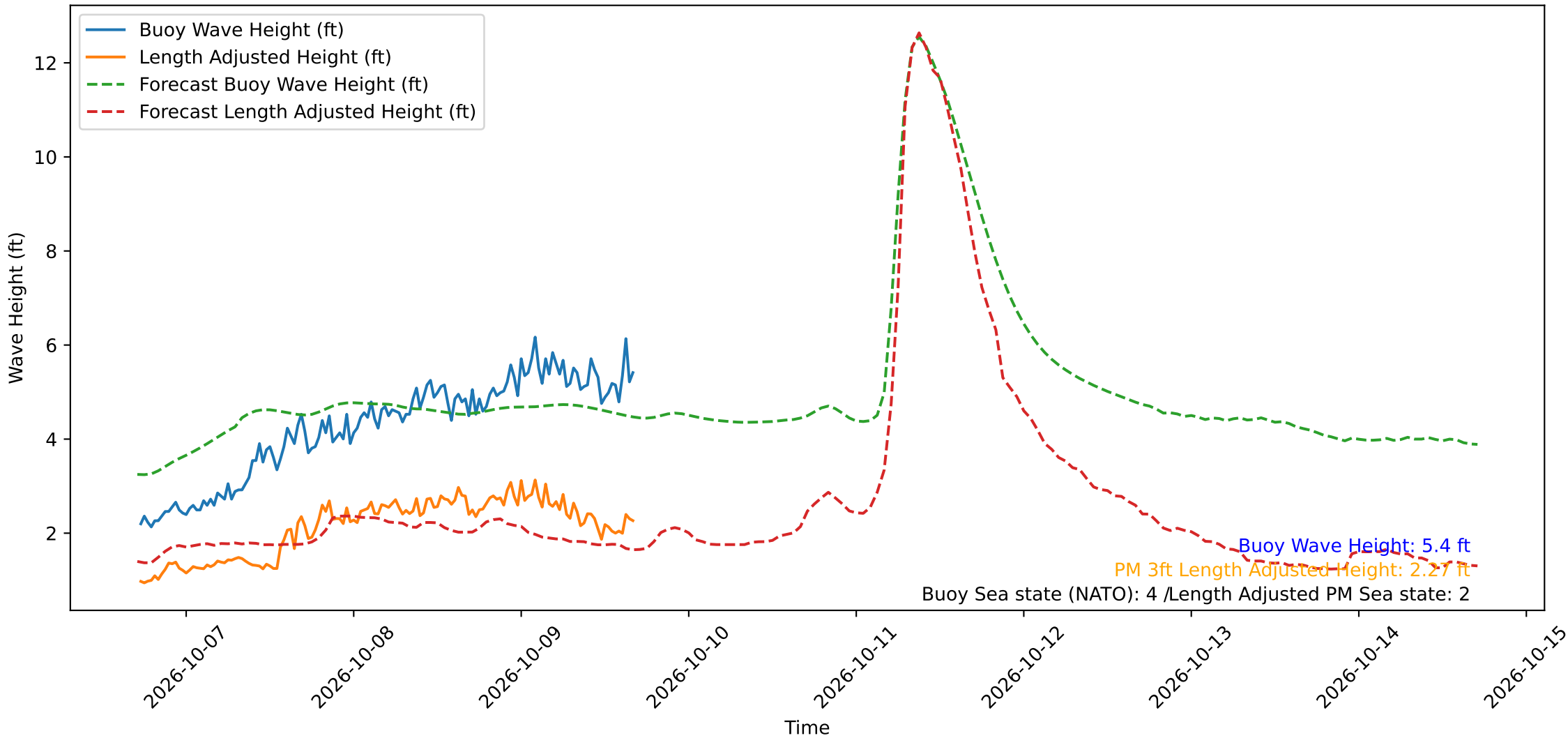
Wave Heights over Time for Green Beach at 2026-10-09 17:01:12
