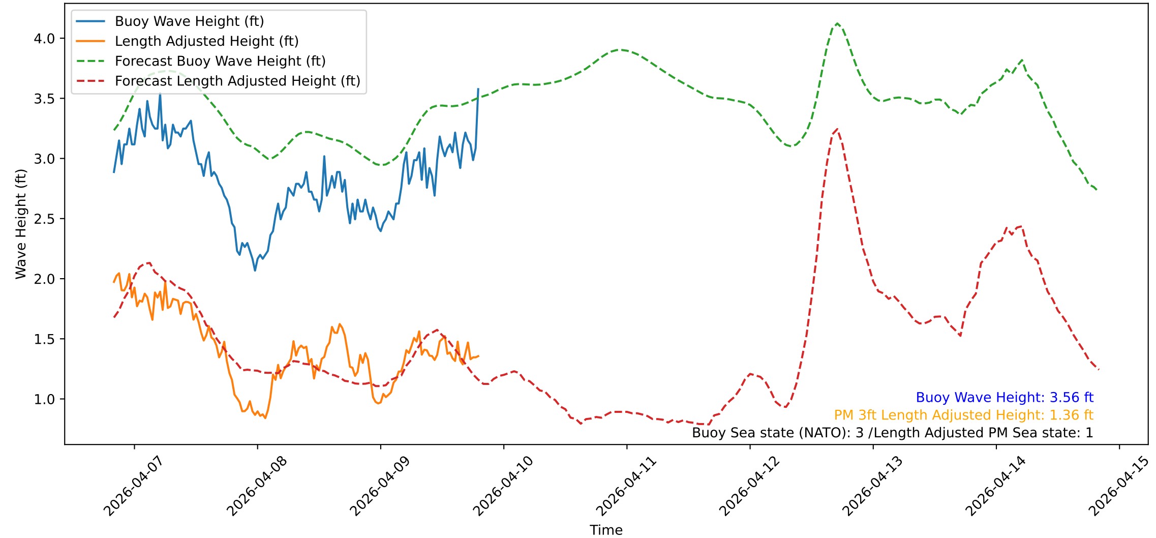
Wave Heights over Time for Red Beach at 2026-04-09 19:50:48
