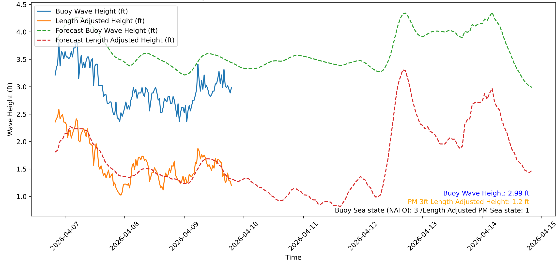
Wave Heights over Time for Green Beach at 2026-04-09 19:51:11
