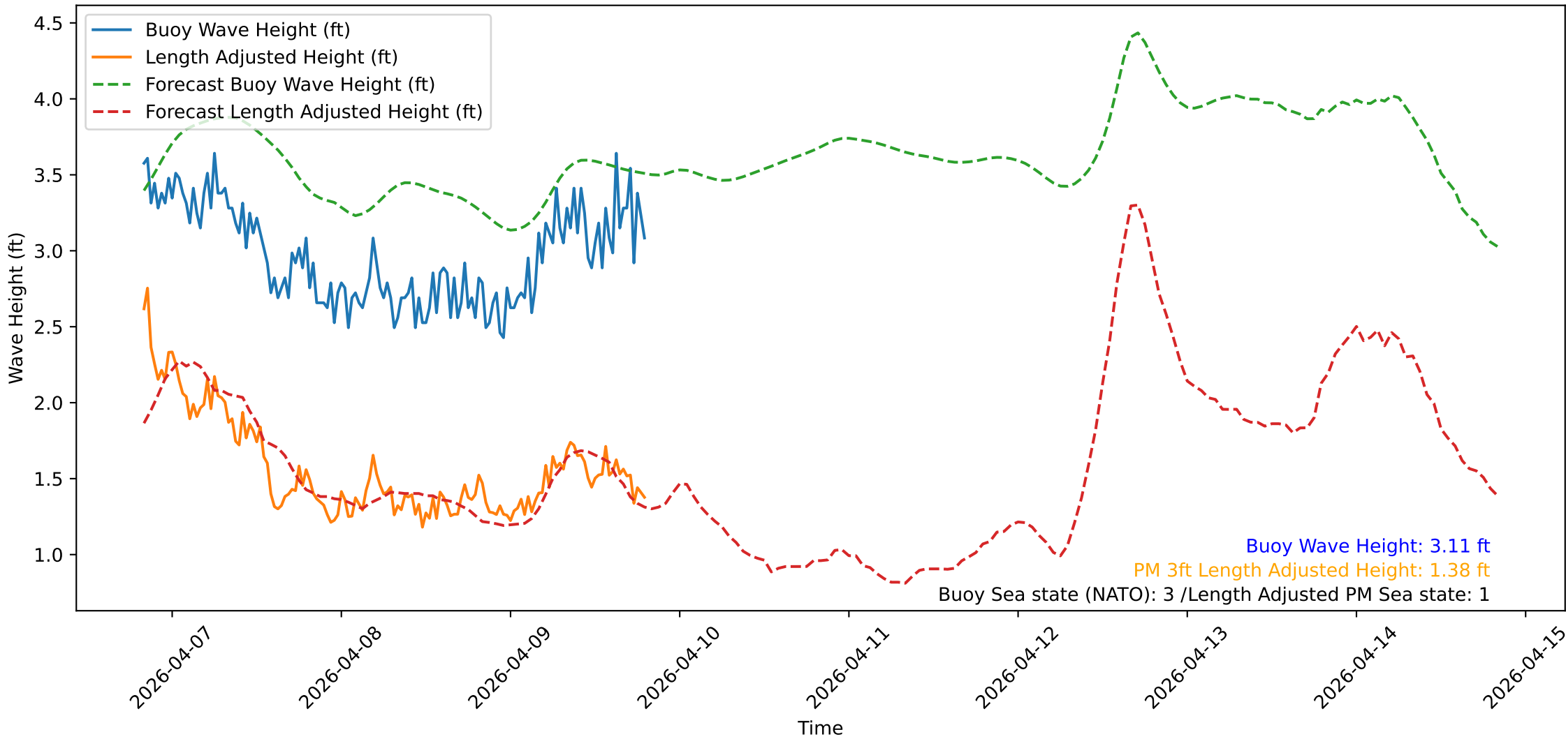
Wave Heights over Time for Oceanside Harbor at 2026-04-09 19:50:32
