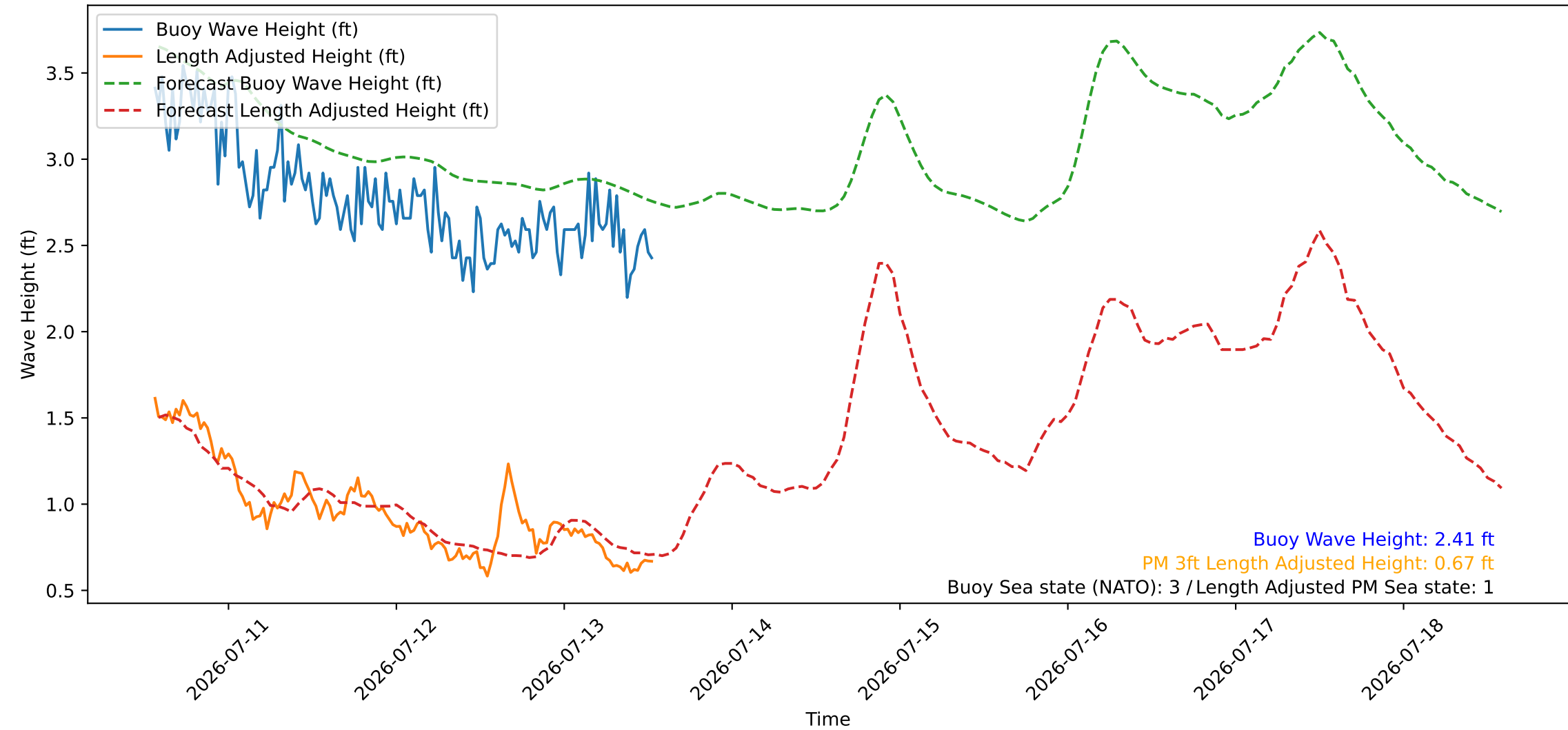
Wave Heights over Time for Green Beach at 2026-07-13 13:31:07
