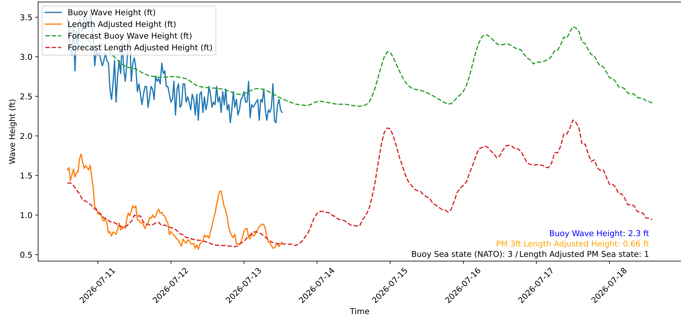
Wave Heights over Time for Red Beach at 2026-07-13 13:30:45
