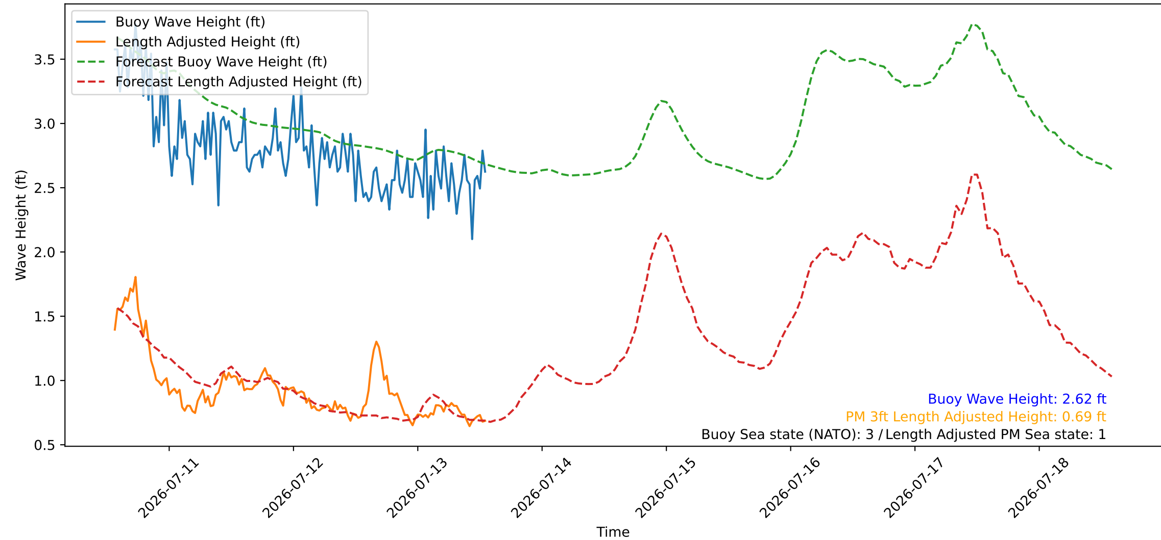
Wave Heights over Time for Oceanside Harbor at 2026-07-13 13:30:26
