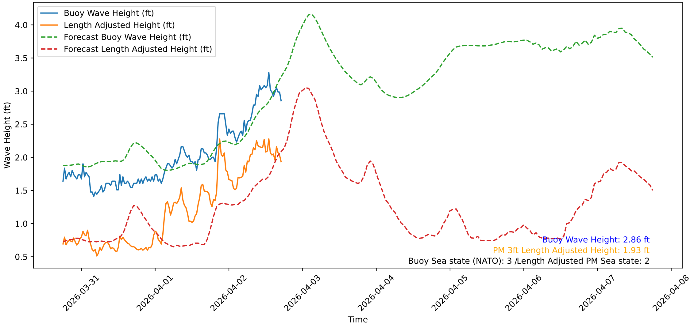
Wave Heights over Time for Green Beach at 2026-04-02 18:11:09
