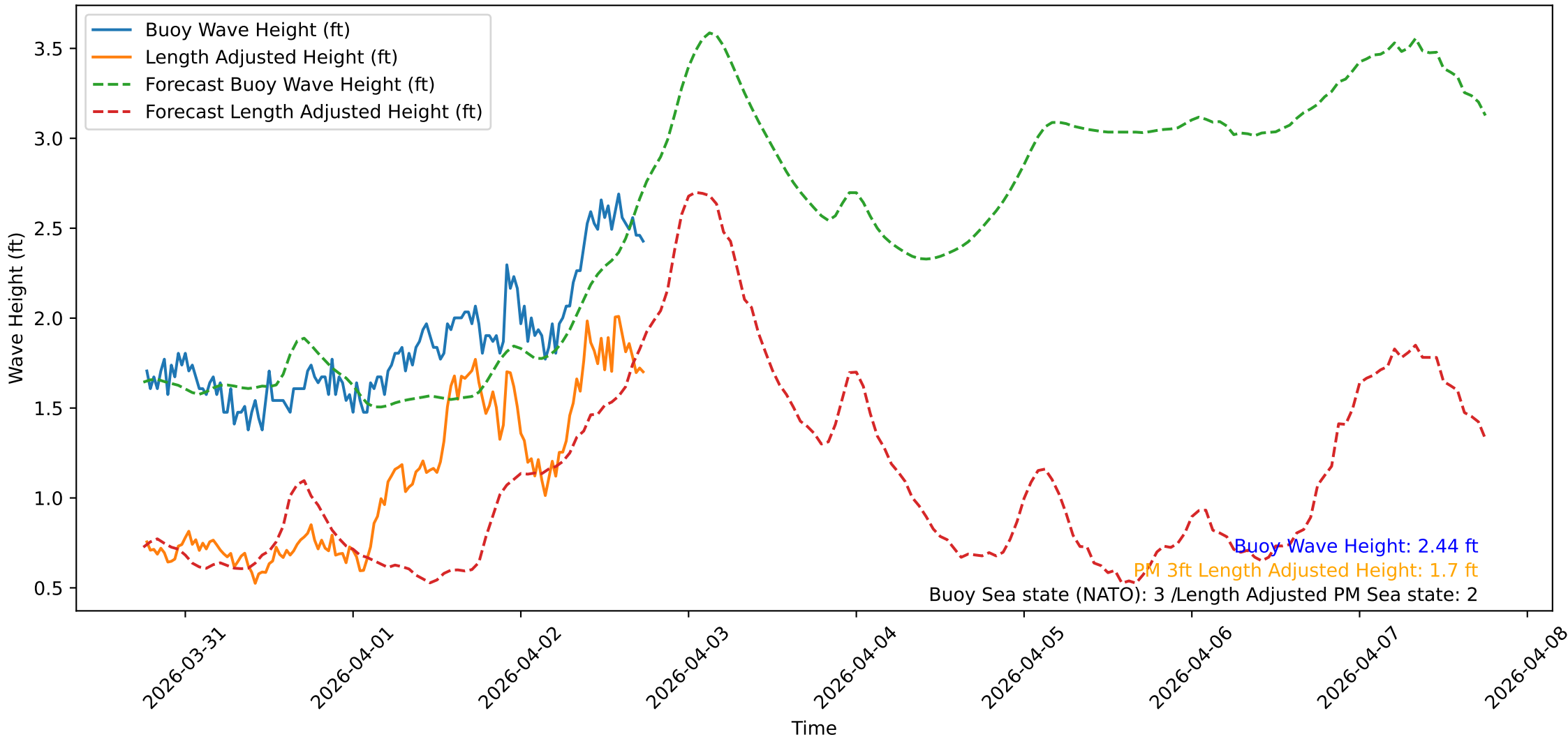
Wave Heights over Time for Red Beach at 2026-04-02 18:10:47
