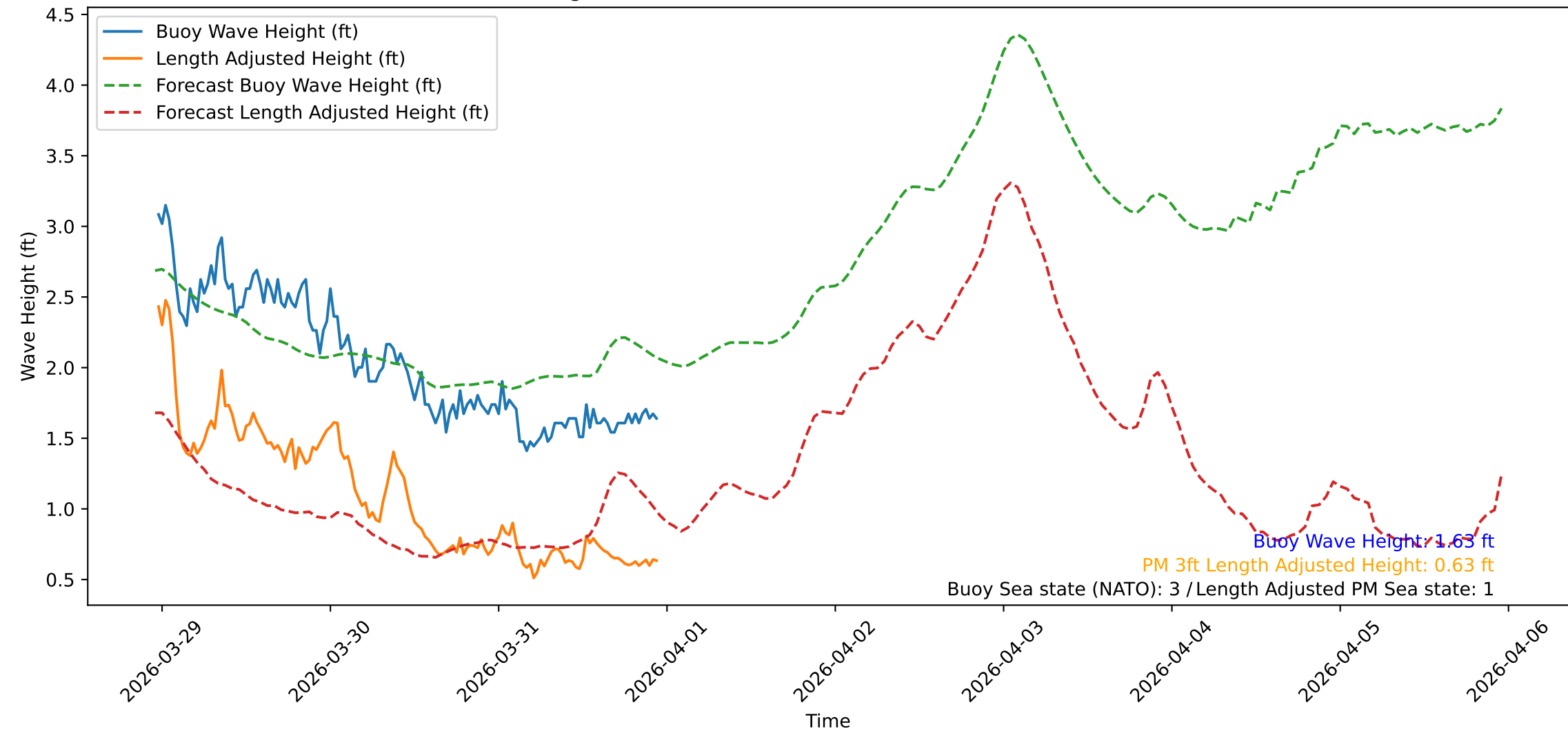
Wave Heights over Time for Green Beach at 2026-03-31 23:21:11
