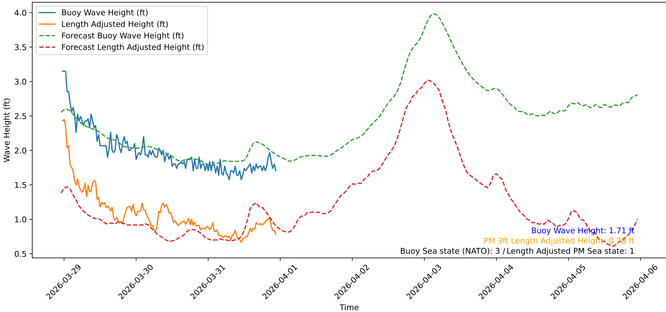
Wave Heights over Time for Oceanside Harbor at 2026-03-31 23:20:32
