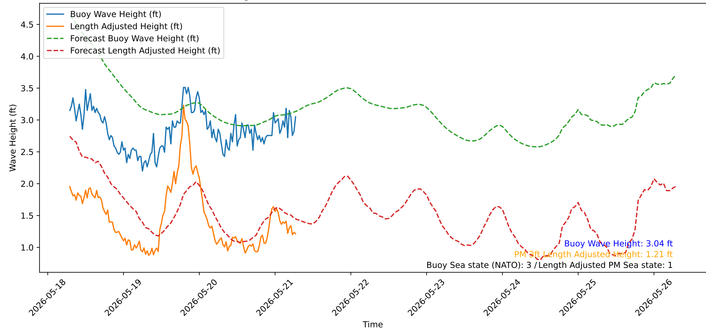
Wave Heights over Time for Oceanside Harbor at 2026-05-21 07:10:32
