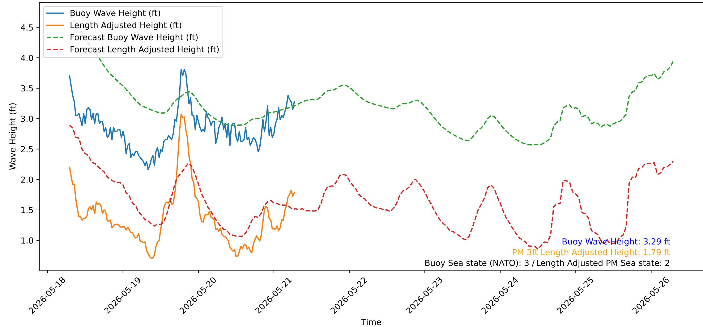
Wave Heights over Time for Green Beach at 2026-05-21 07:11:14
