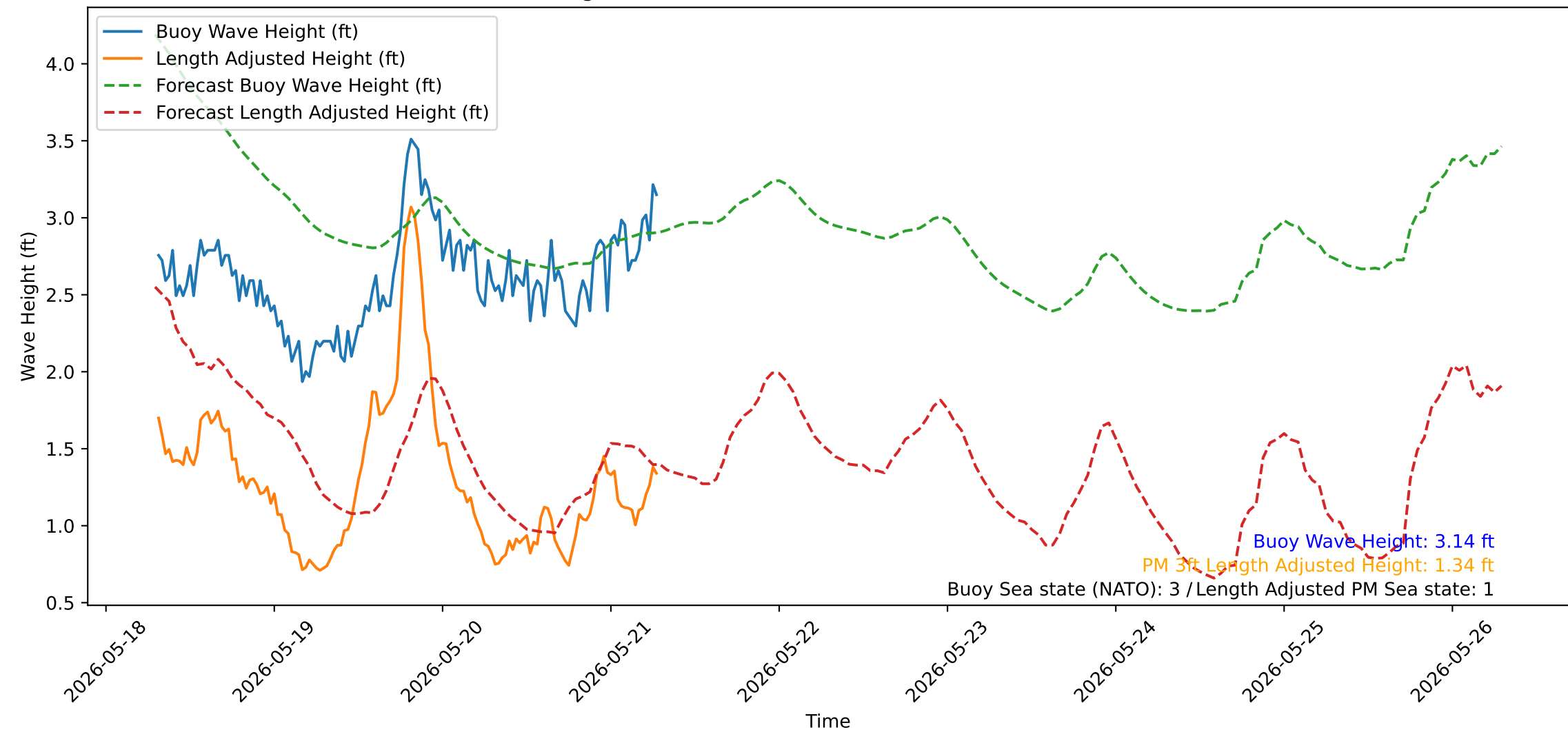
Wave Heights over Time for Red Beach at 2026-05-21 07:10:51
