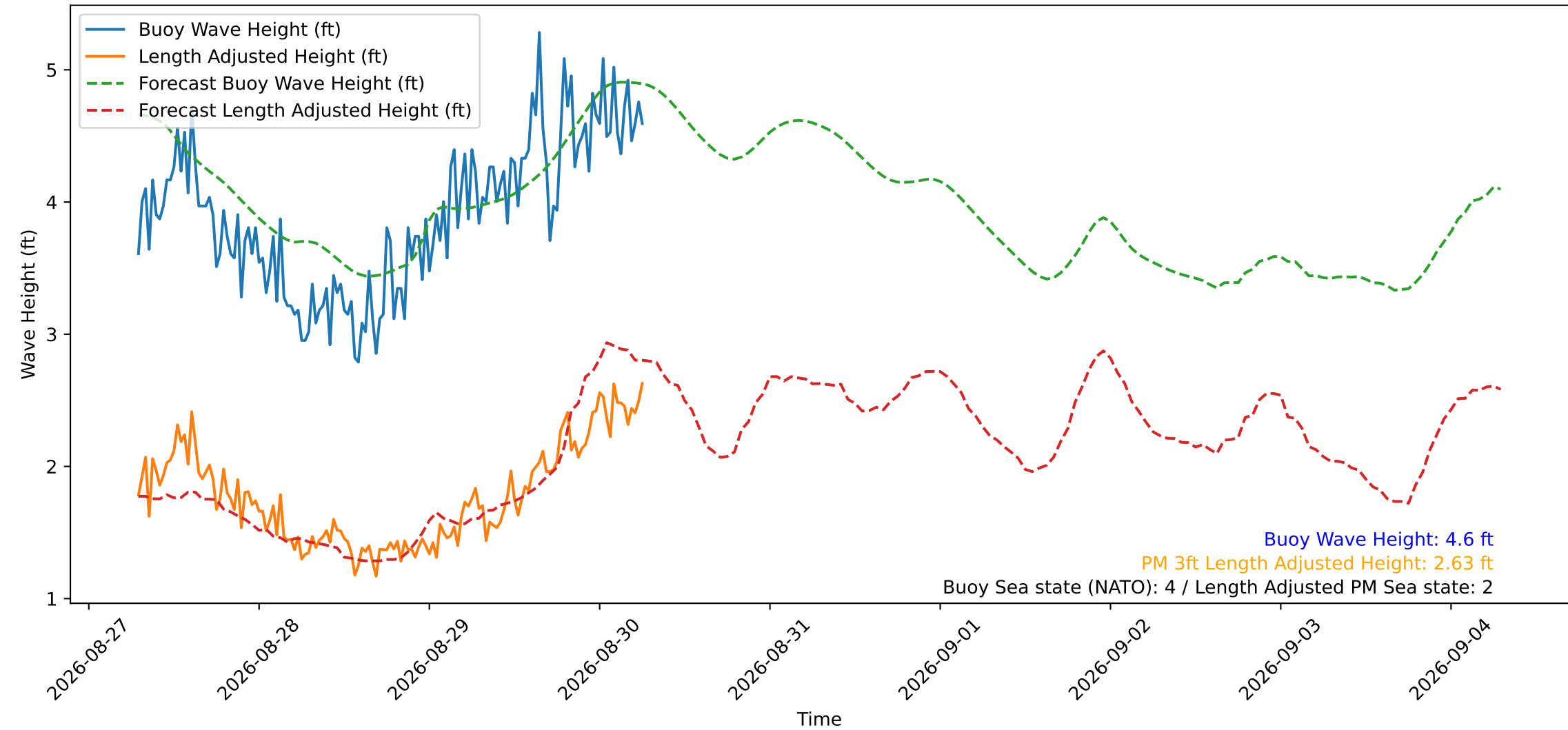
Wave Heights over Time for Oceanside Harbor at 2026-08-30 07:00:30
