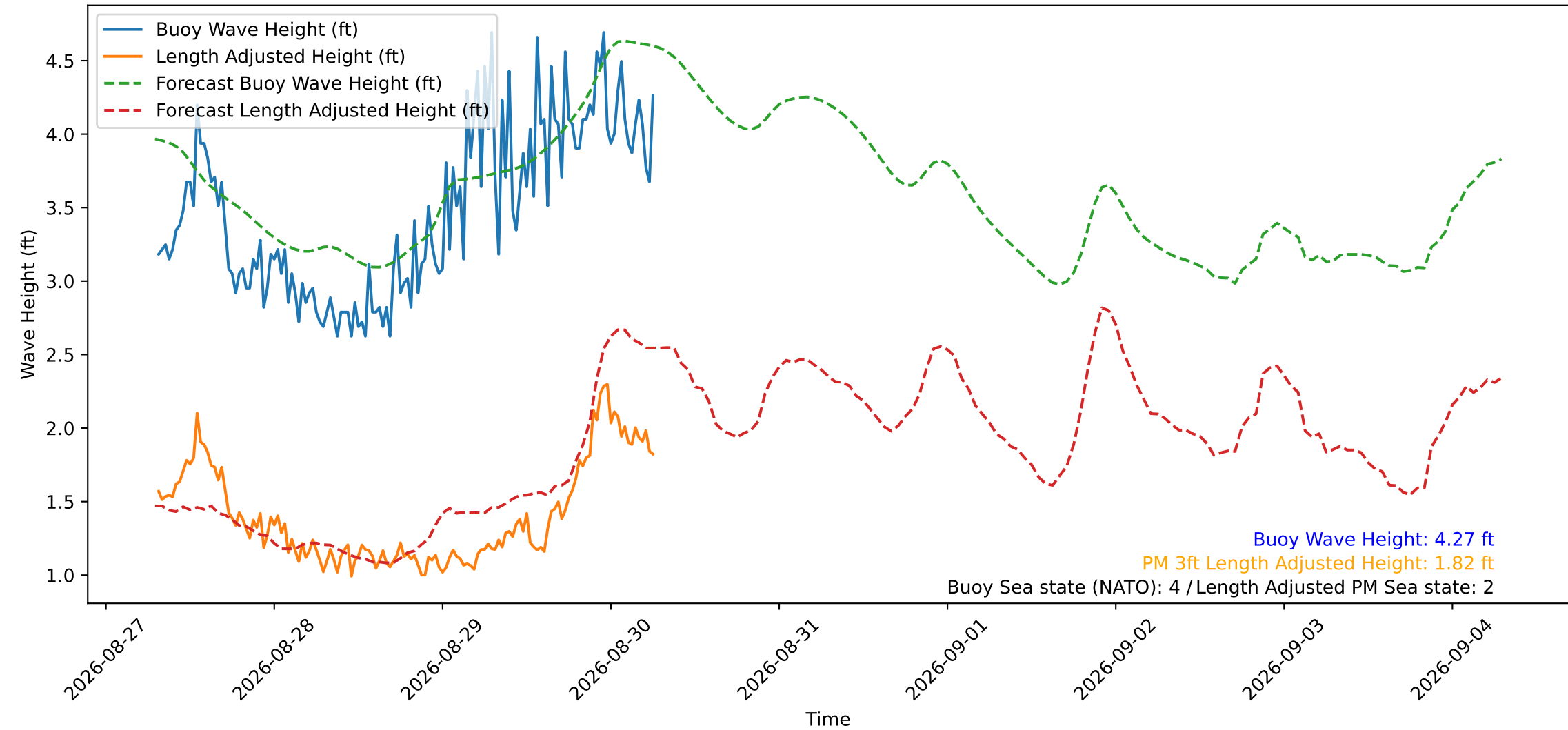
Wave Heights over Time for Red Beach at 2026-08-30 07:00:49
