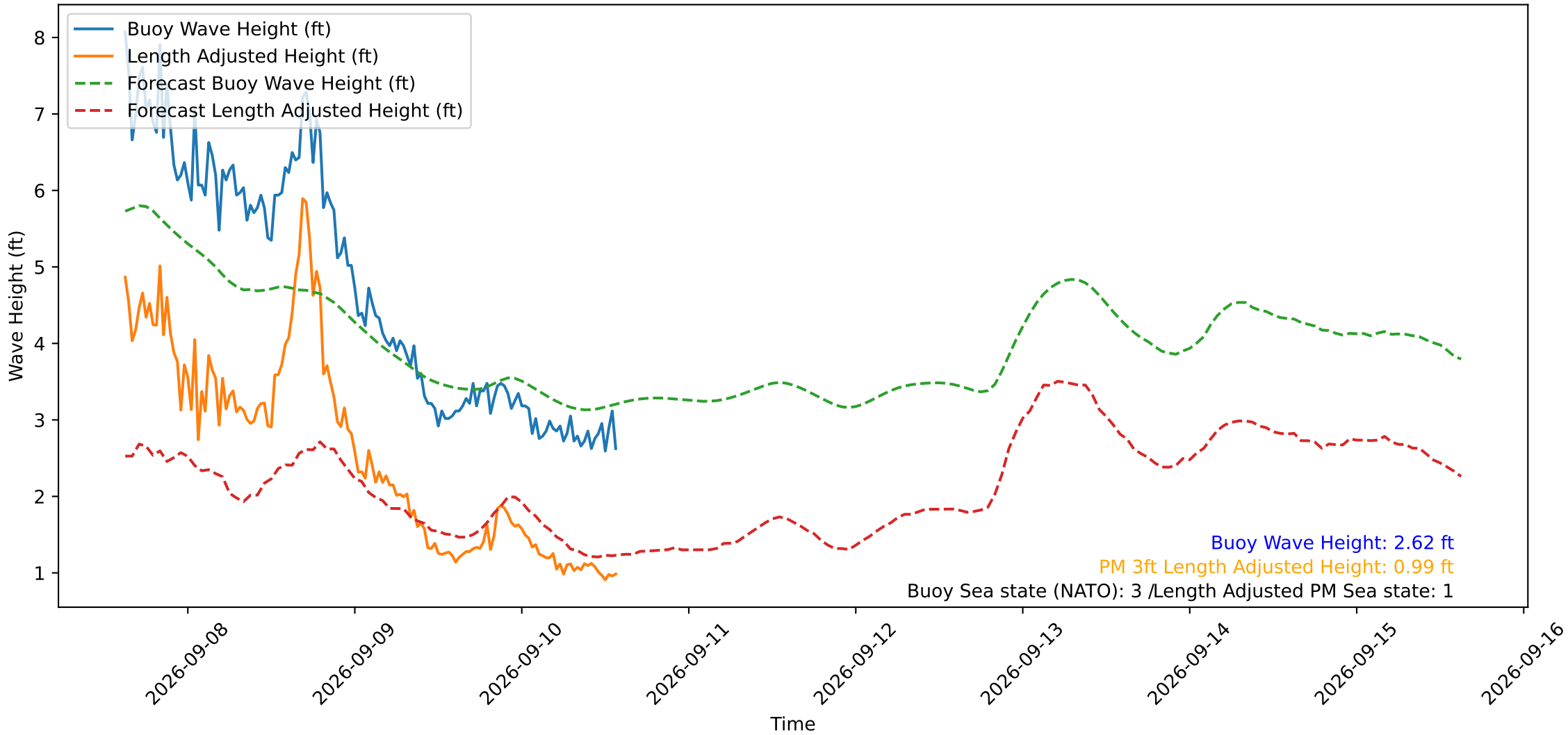
Wave Heights over Time for Green Beach at 2026-09-10 14:31:12
