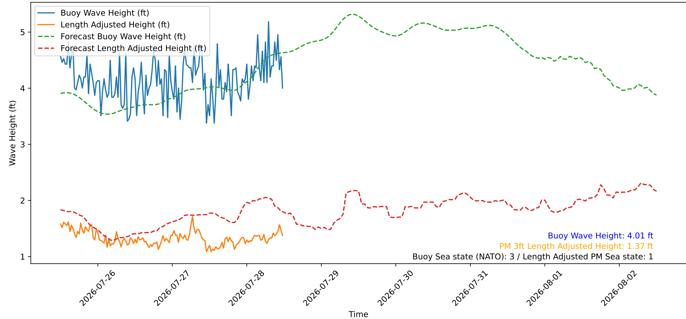
Wave Heights over Time for Green Beach at 2026-07-28 12:11:09
