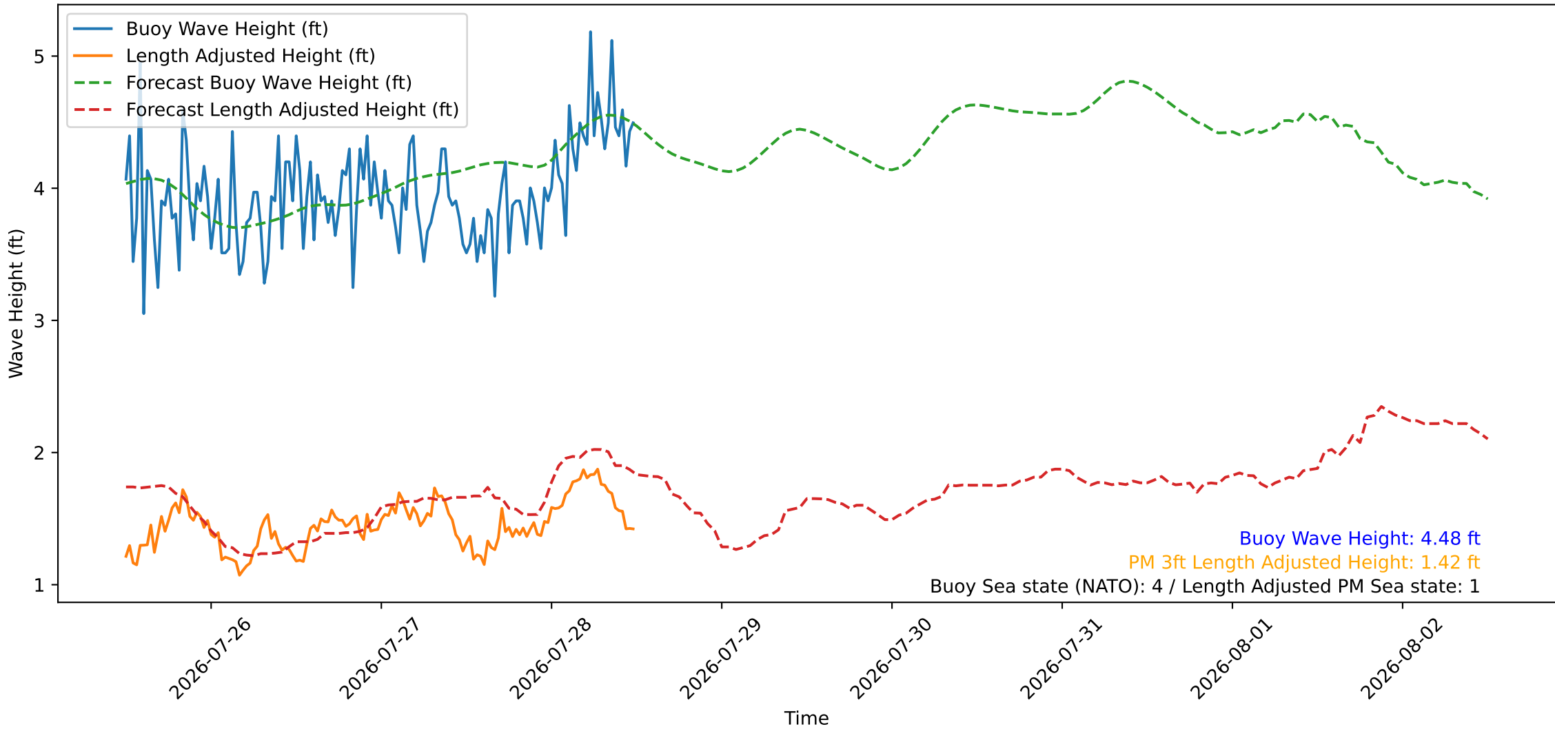
Wave Heights over Time for Oceanside Harbor at 2026-07-28 12:10:26
