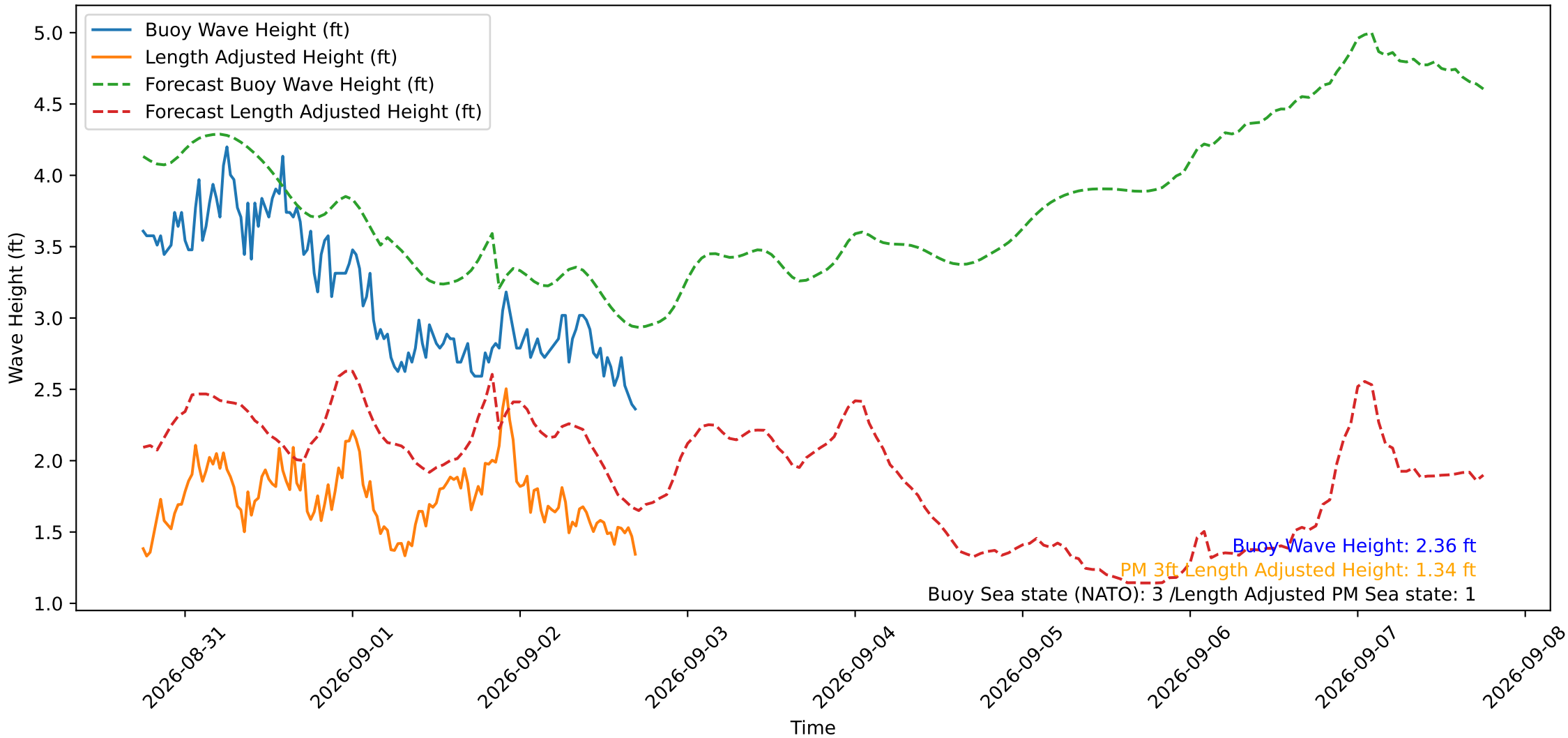
Wave Heights over Time for Red Beach at 2026-09-02 17:30:49
