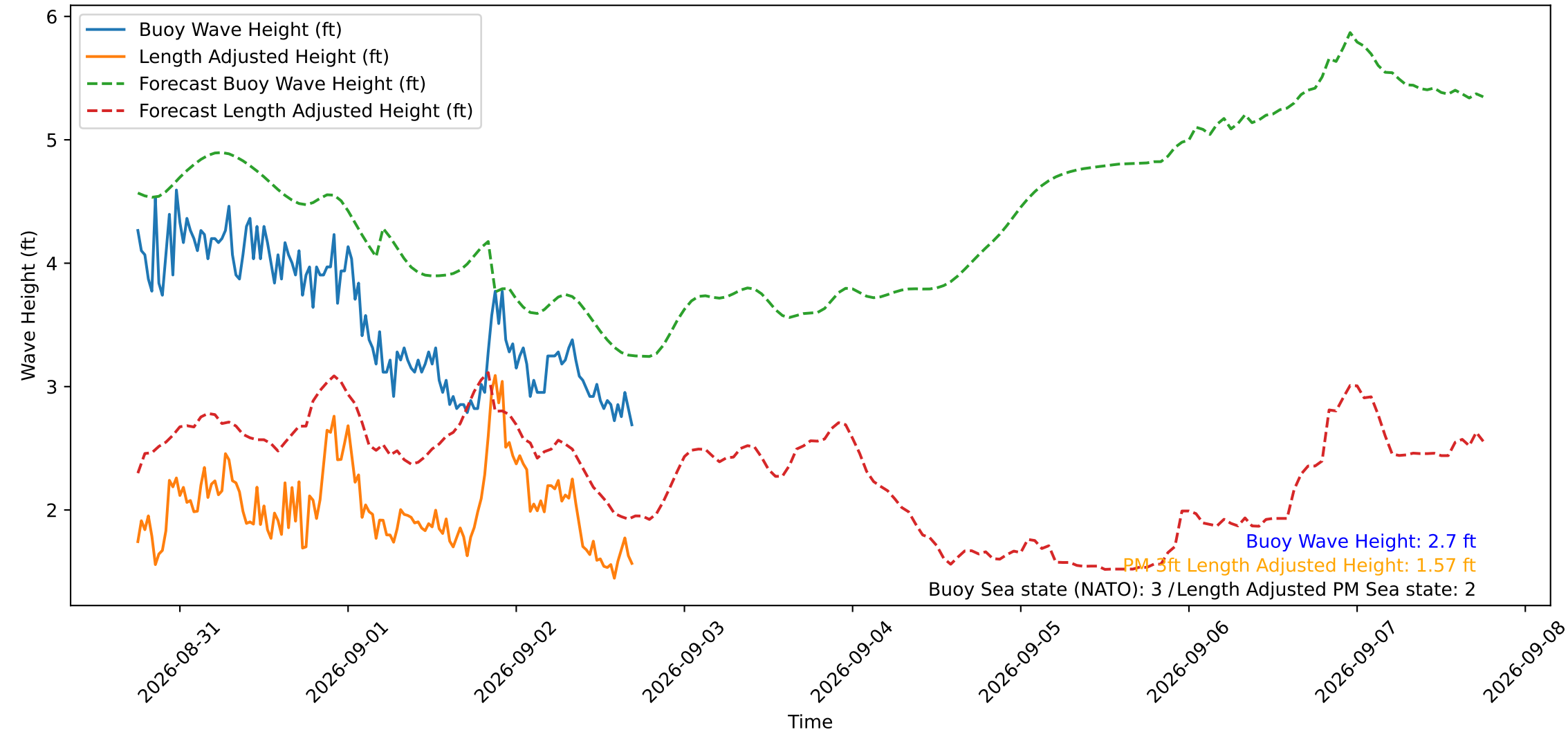
Wave Heights over Time for Green Beach at 2026-09-02 17:31:13
