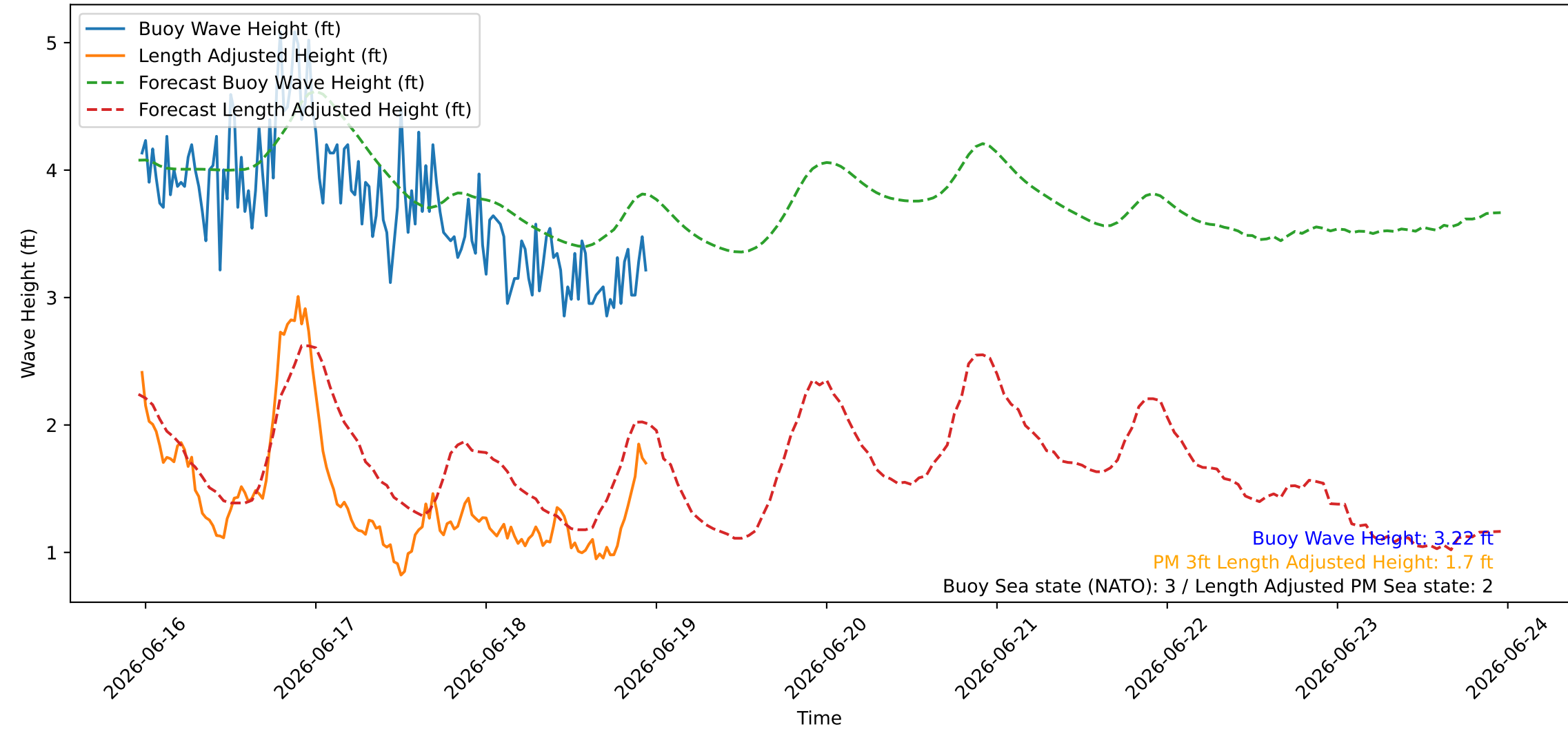
Wave Heights over Time for Green Beach at 2026-06-18 23:21:09
