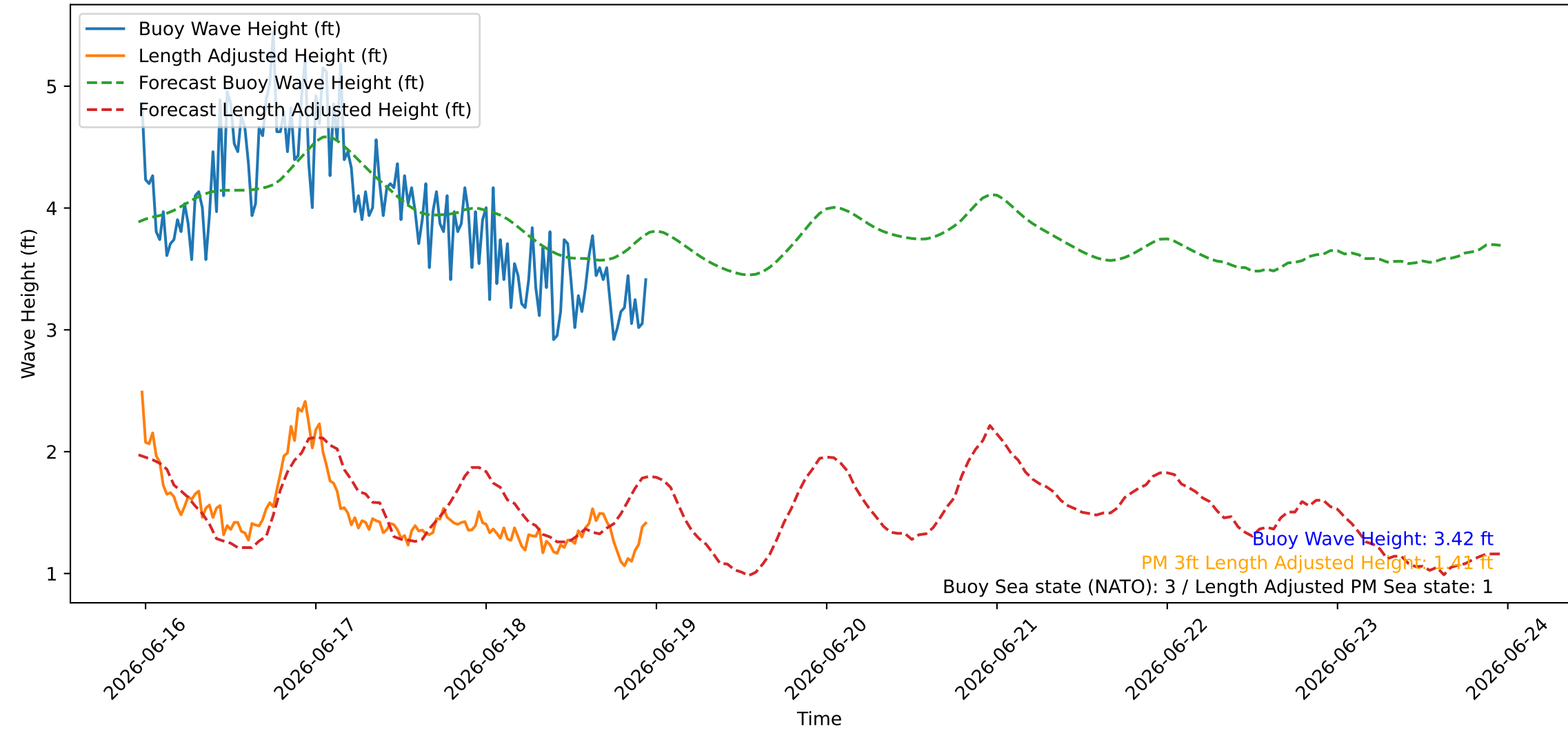
Wave Heights over Time for Oceanside Harbor at 2026-06-18 23:20:26
